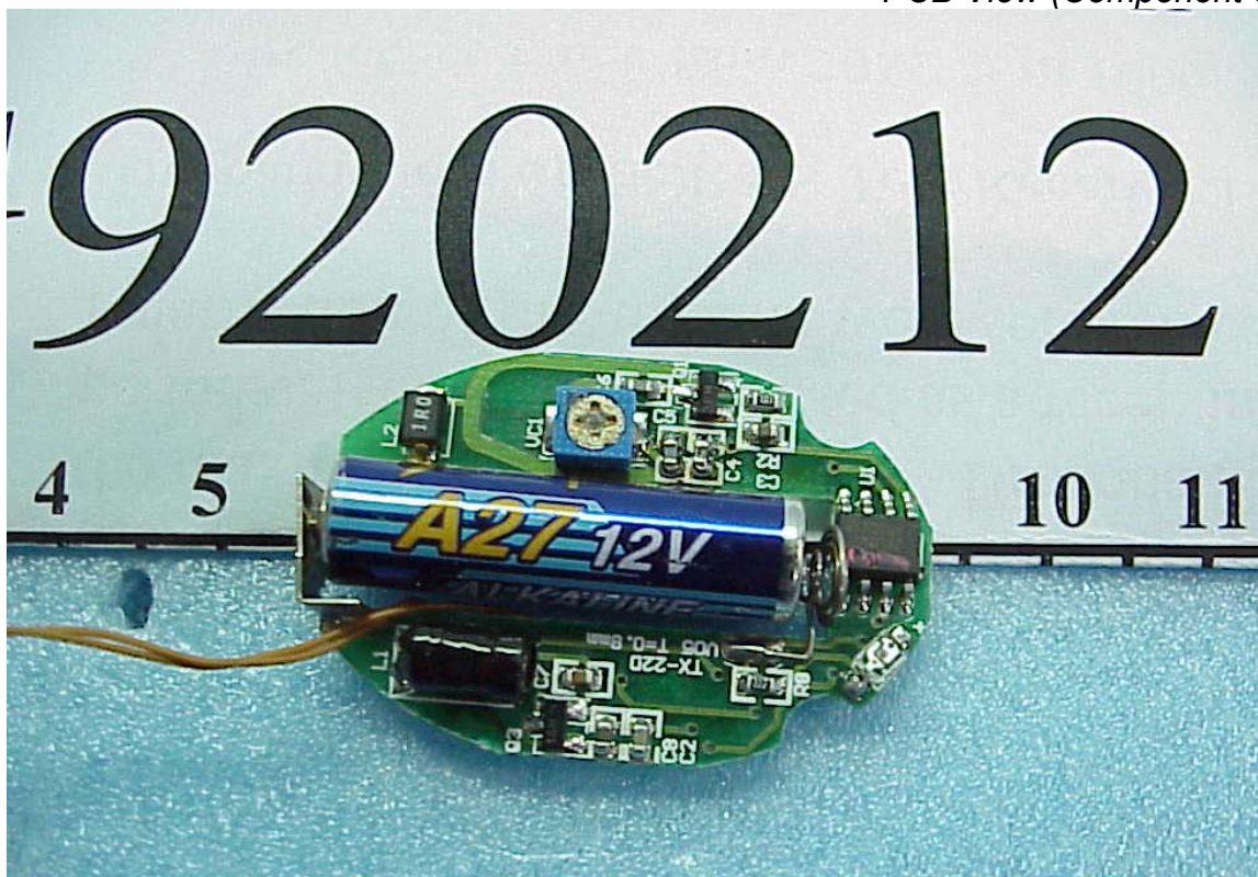
Photos 4 PCB View (Component Side)
