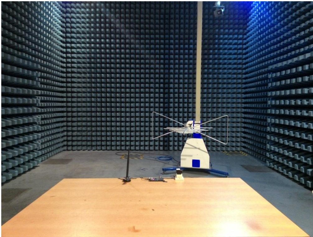
FCC Part15B Radiated Emission below 1GHz -Front
