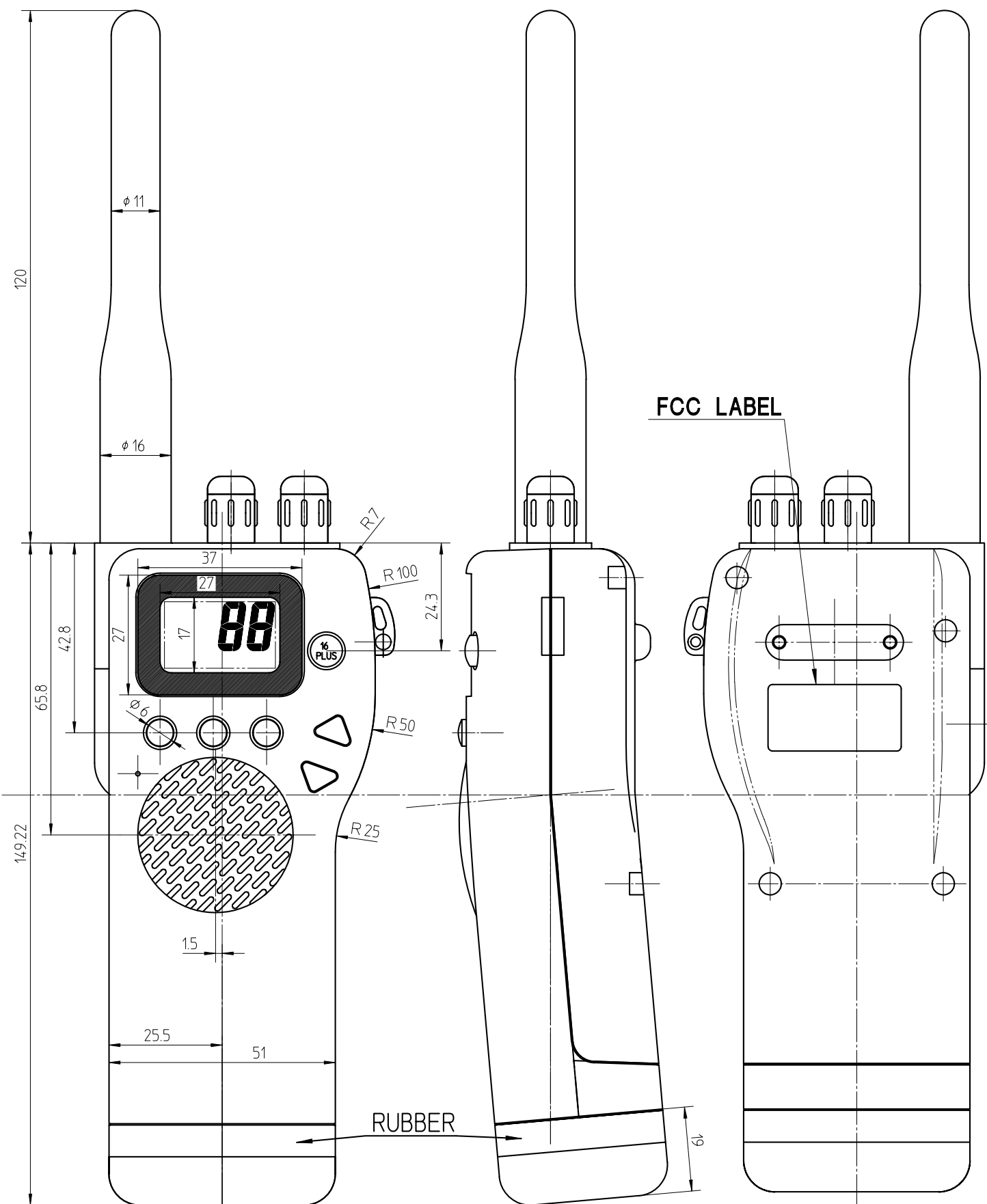
RAY 100 Handheld VHF
