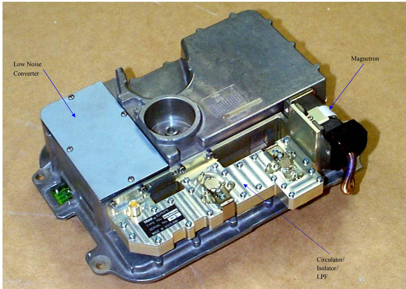
4kW Open Array Scanner Unit
