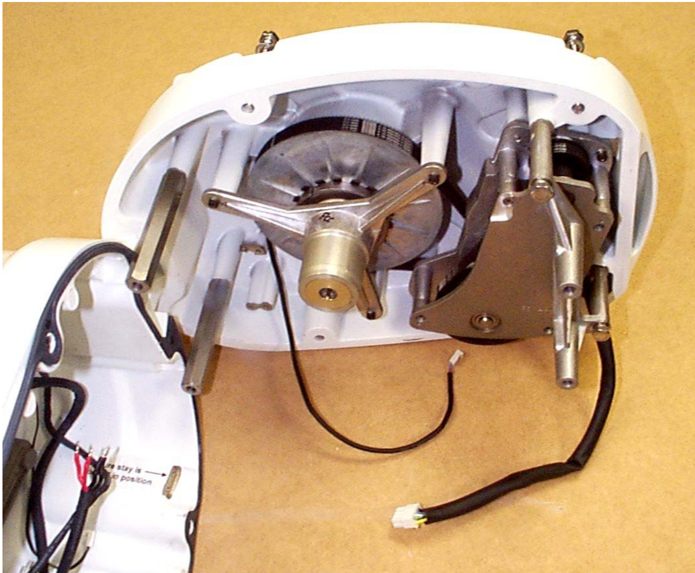
4Kw Open Array Scanner Unit
