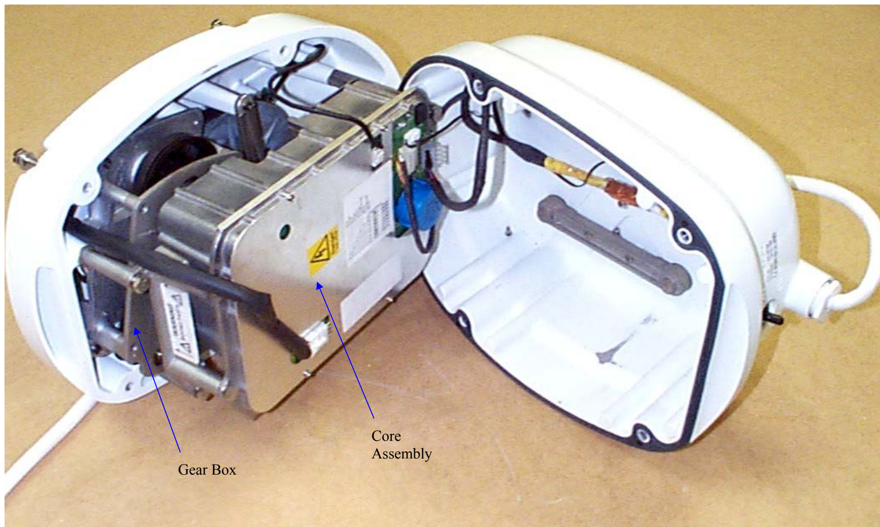
4Kw Open Array Scanner Unit
