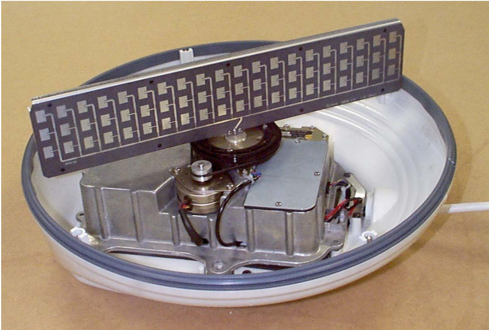
2Kw, 18" Radome Scanner Unit
