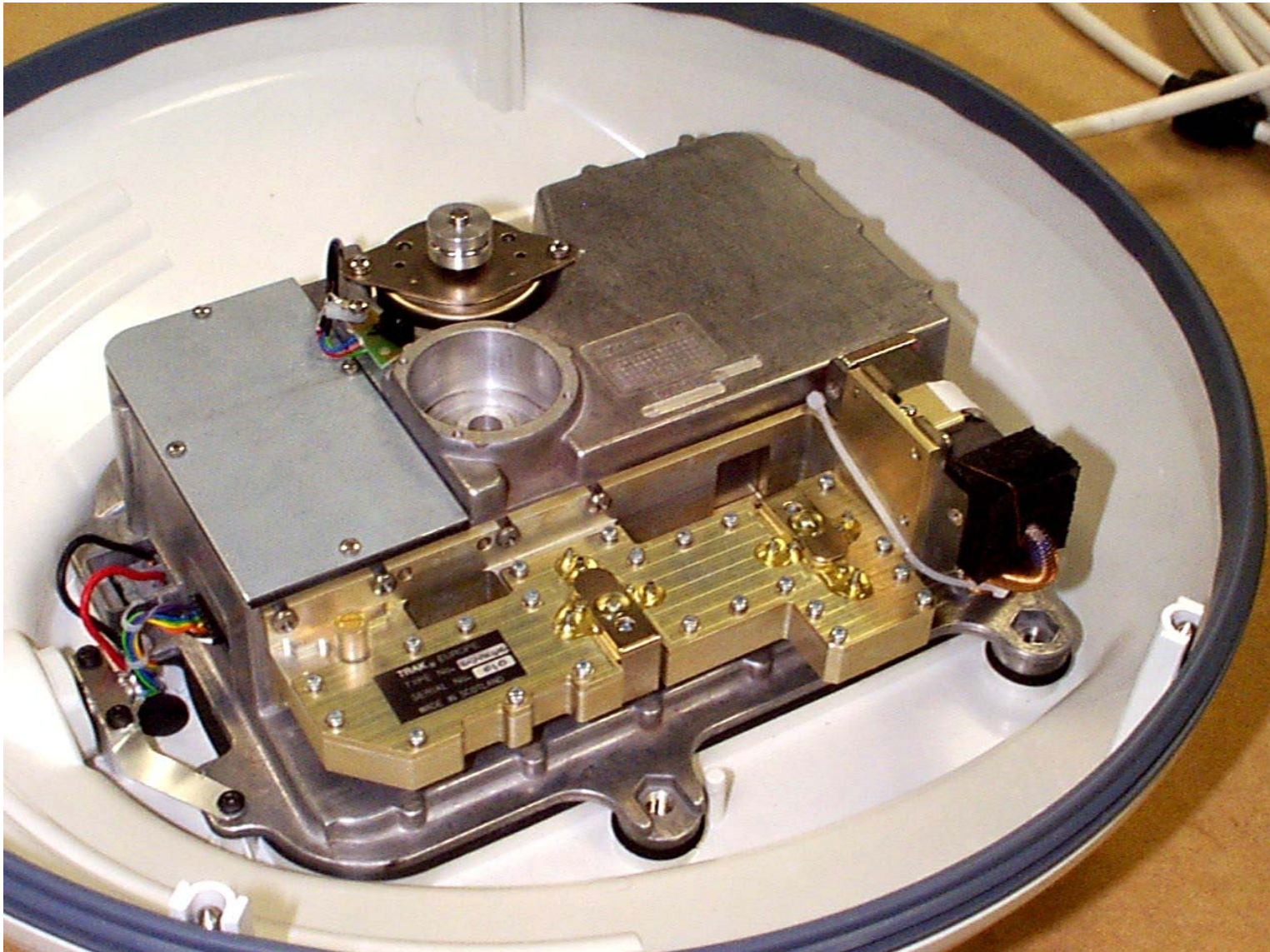
2Kw, 18" Radome Scanner Unit
