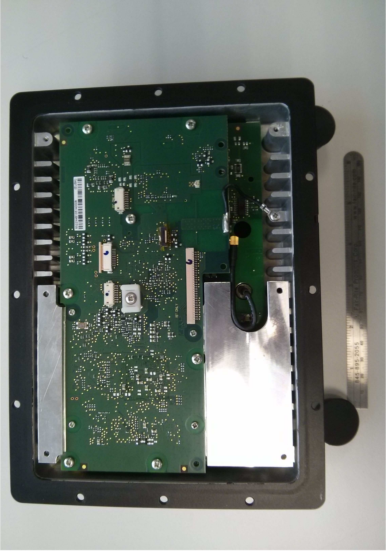
Figure 4 – CPU Module Plate removed
