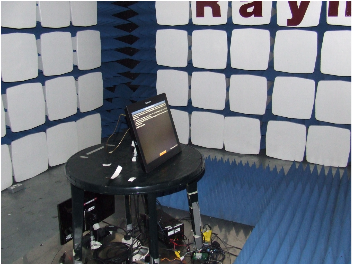
Displays Radiated Measurements Setup
