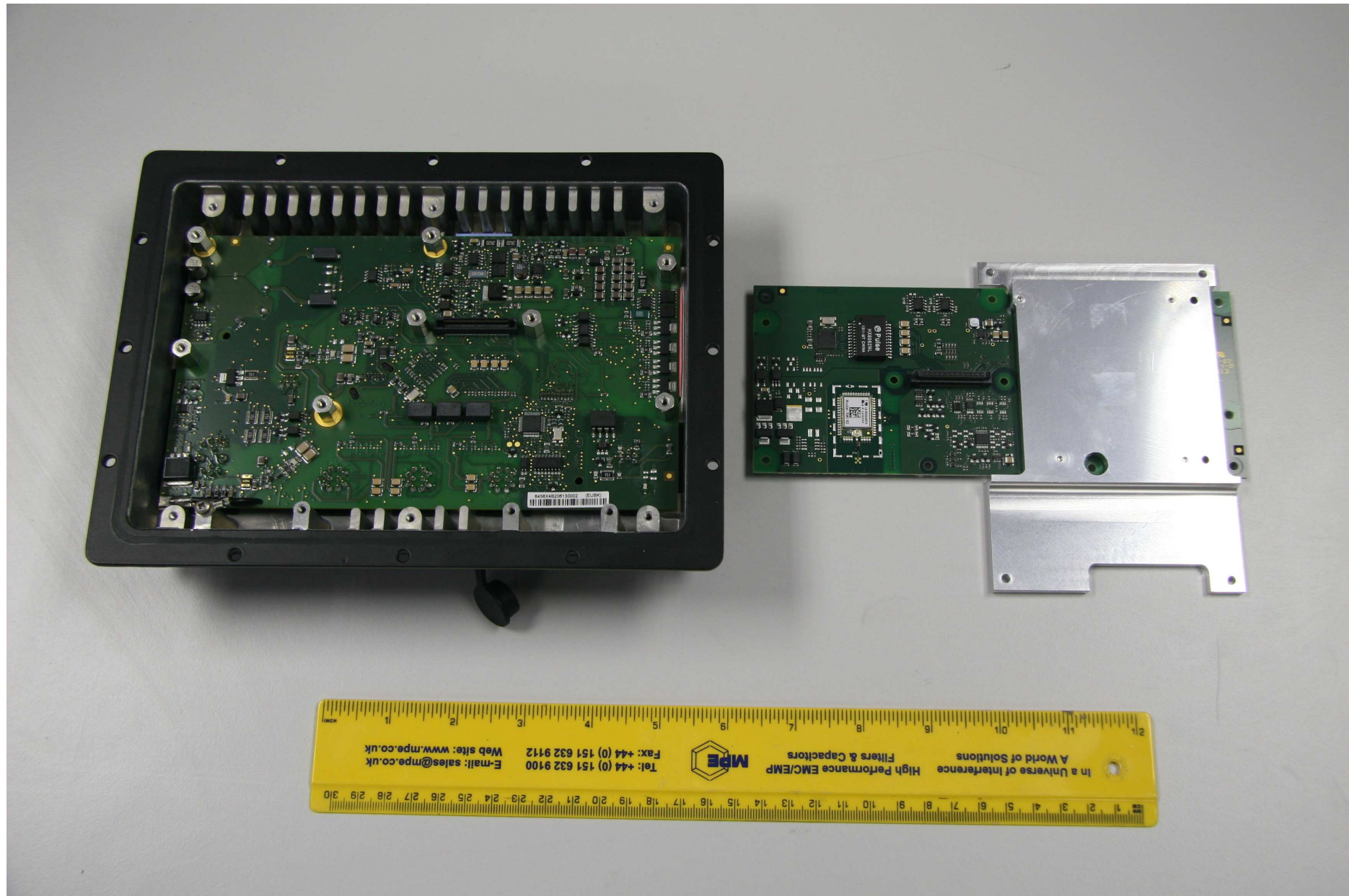
Figure 8 – I/O board in unit, CPU board removed
