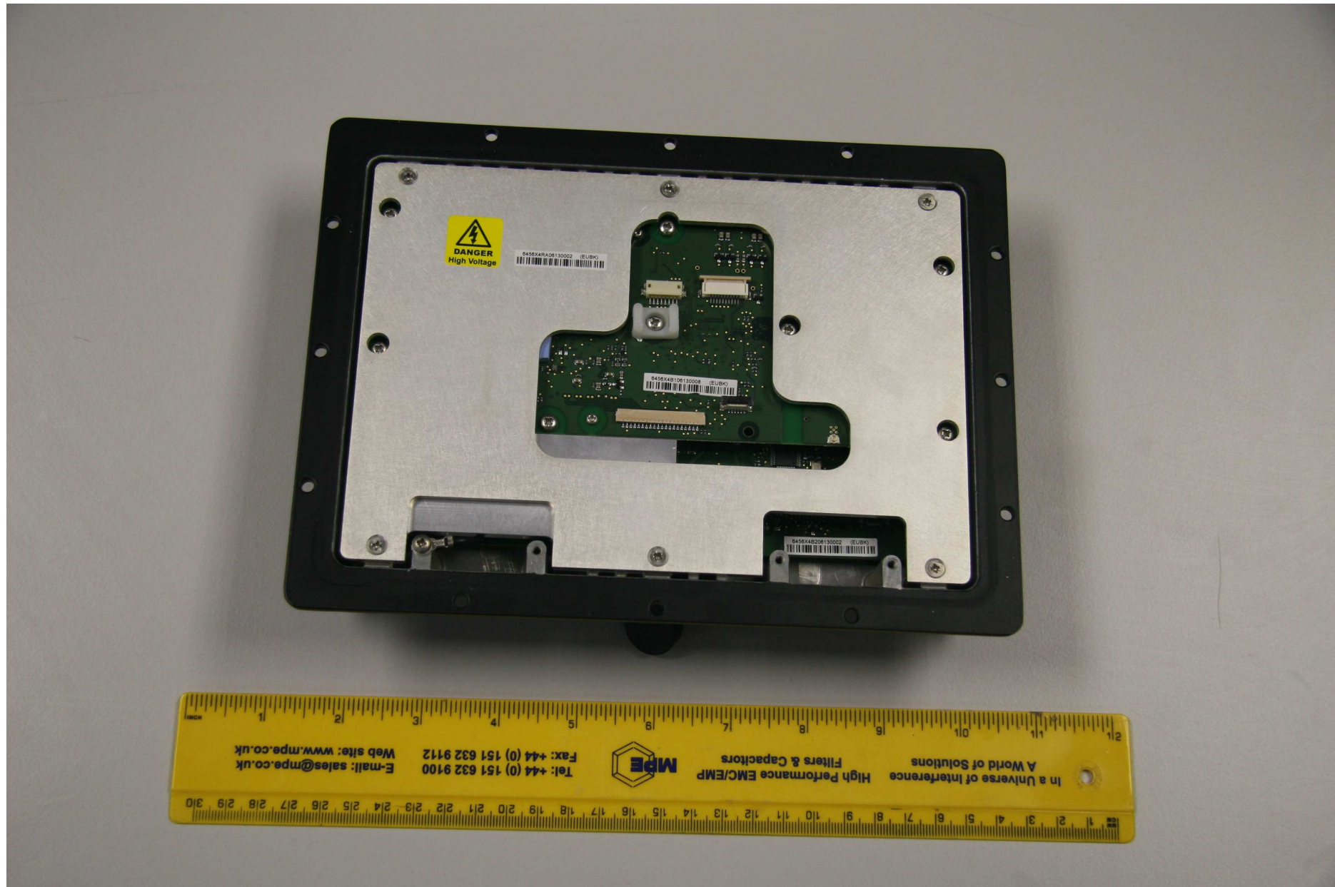
Figure 6 – Processor module front
