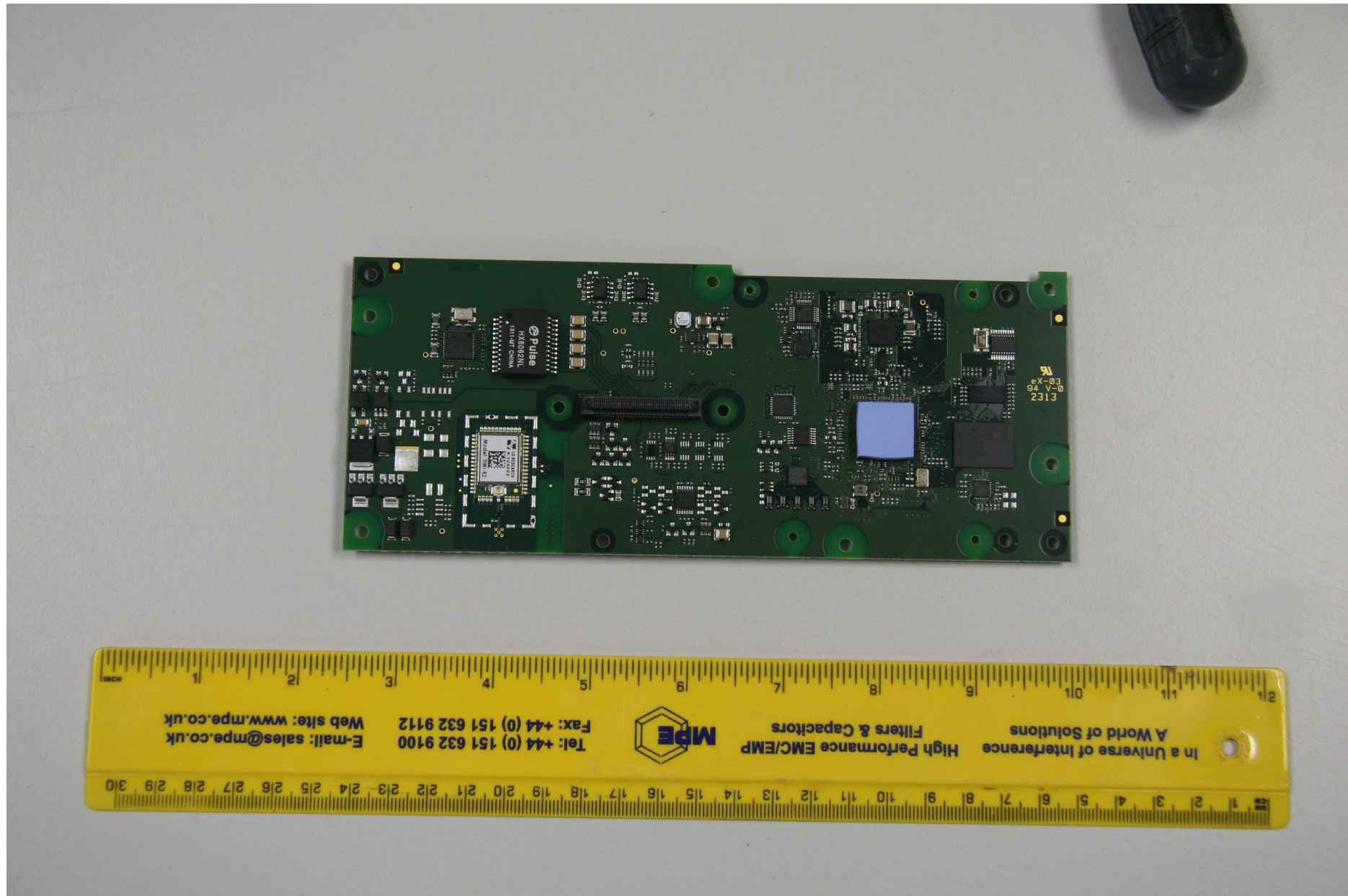
Figure 14 – Rear of CPU board, heatsink removed
