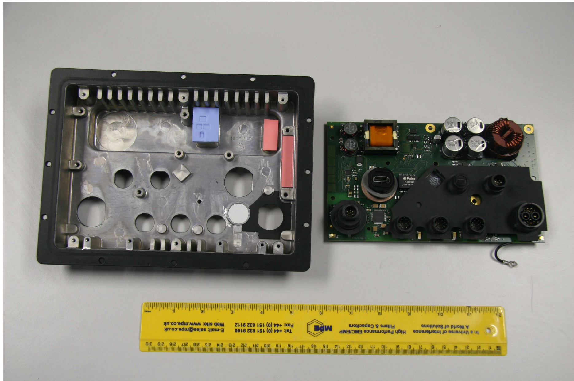
Figure 9 – I/O board removed
