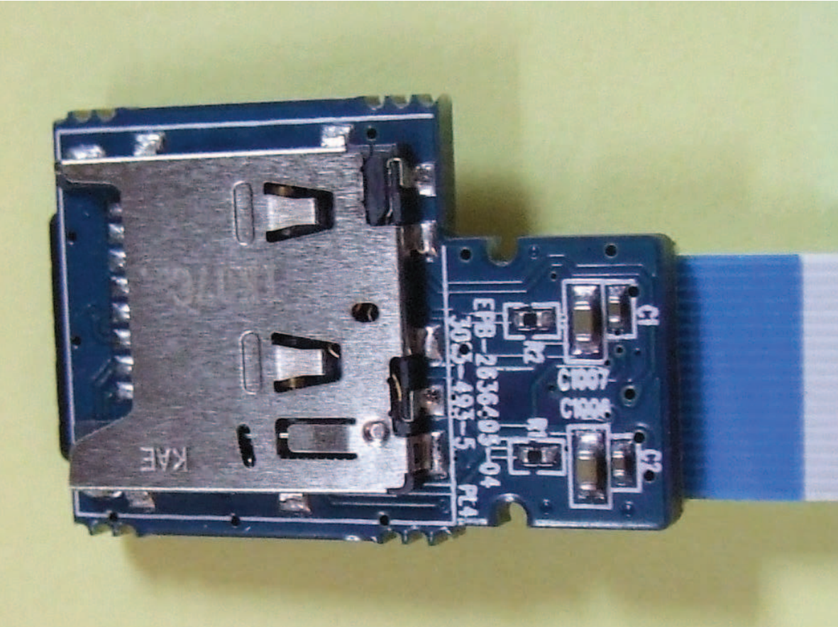
Figure 19 - Micro SD Reader (bottom)
