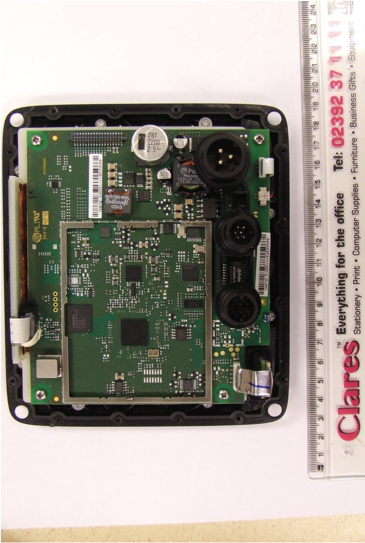
Figure 9 - CPU (top, CAN's removed)
