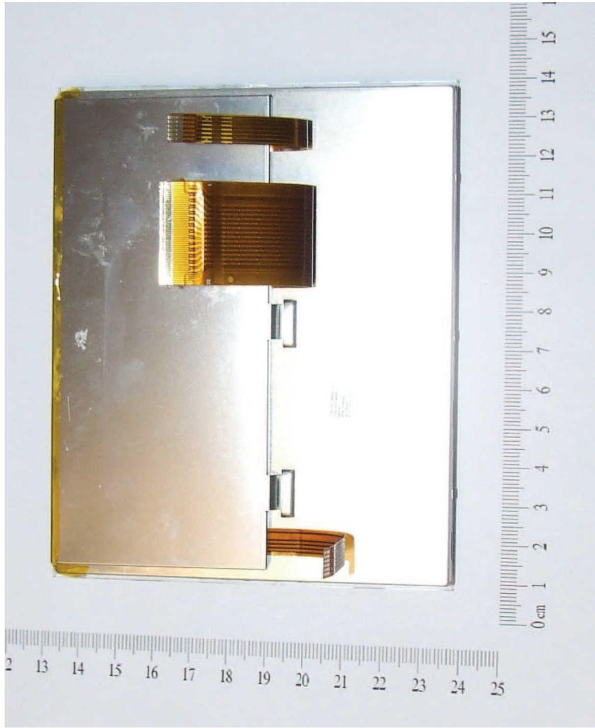
Figure 13 - Rear of LCD
