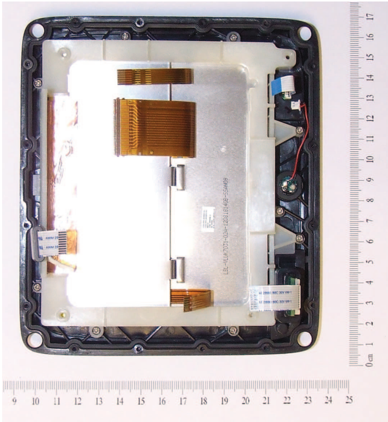
Figure 11 - Rear of LCD (CPU PCB removed)
