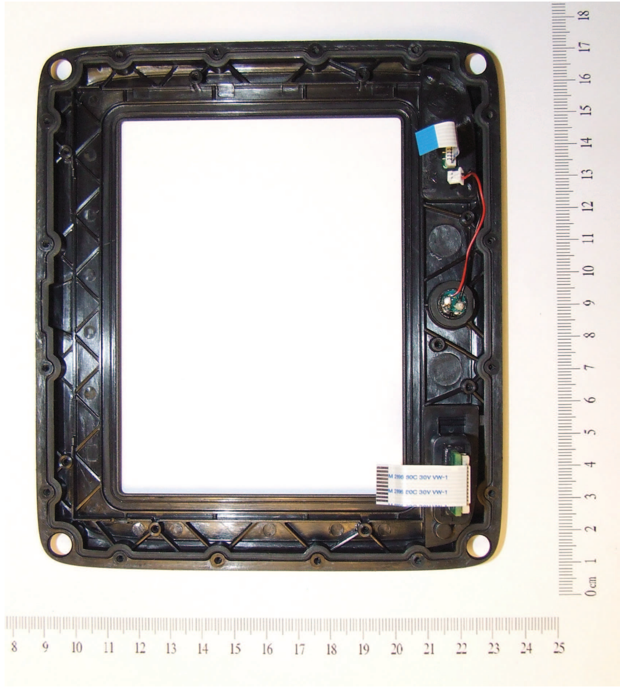
Figure 14 - Rear of front facia
