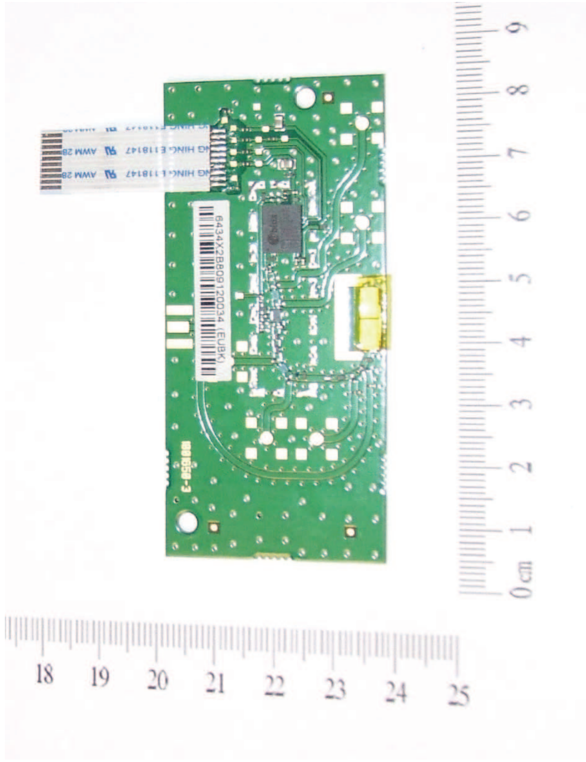
Figure 16 - GPS PCB (top)
