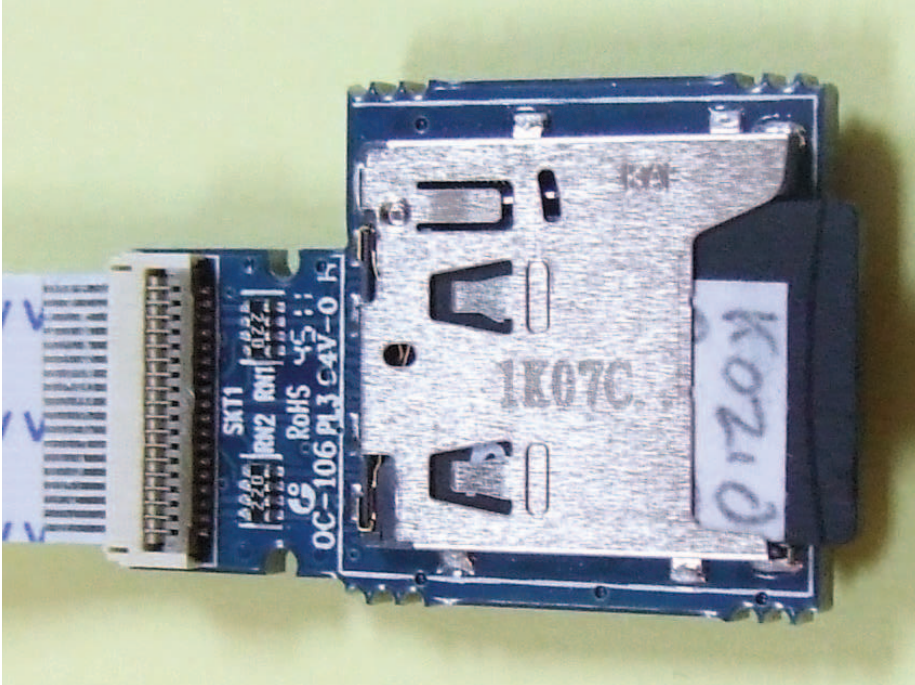
Figure 18 - Micro SD Reader (top)
