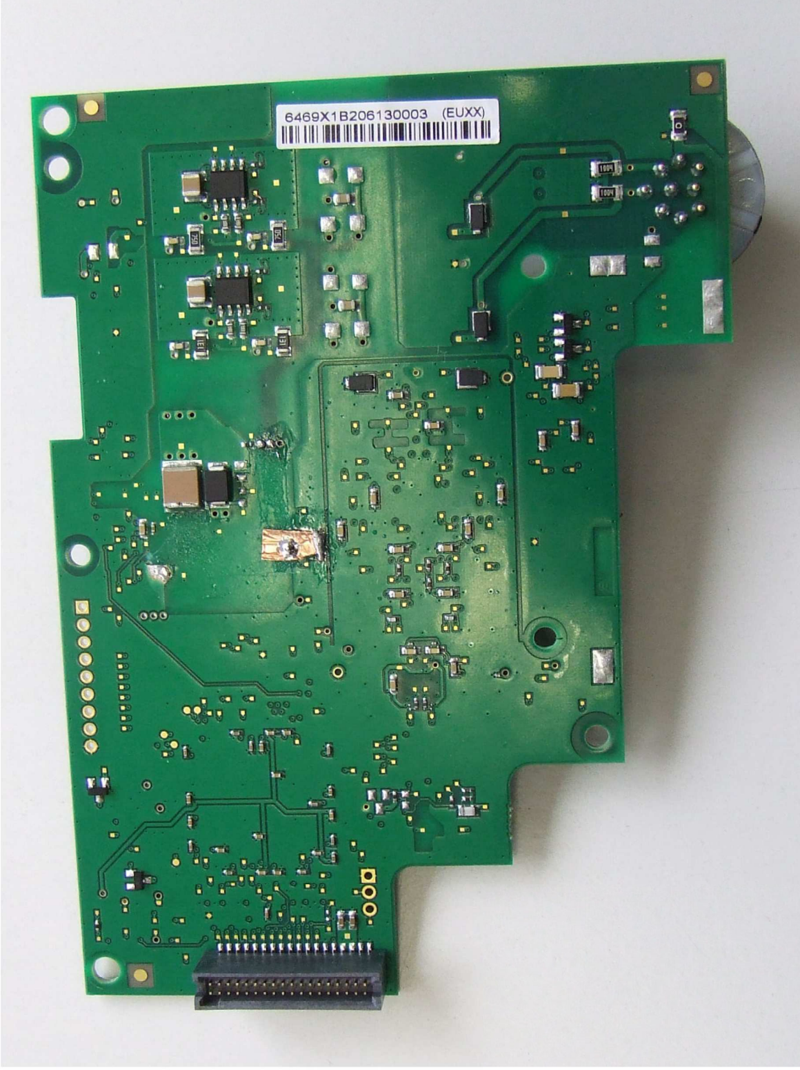
Figure 9 – a68 Sonar PCB (bottom)
