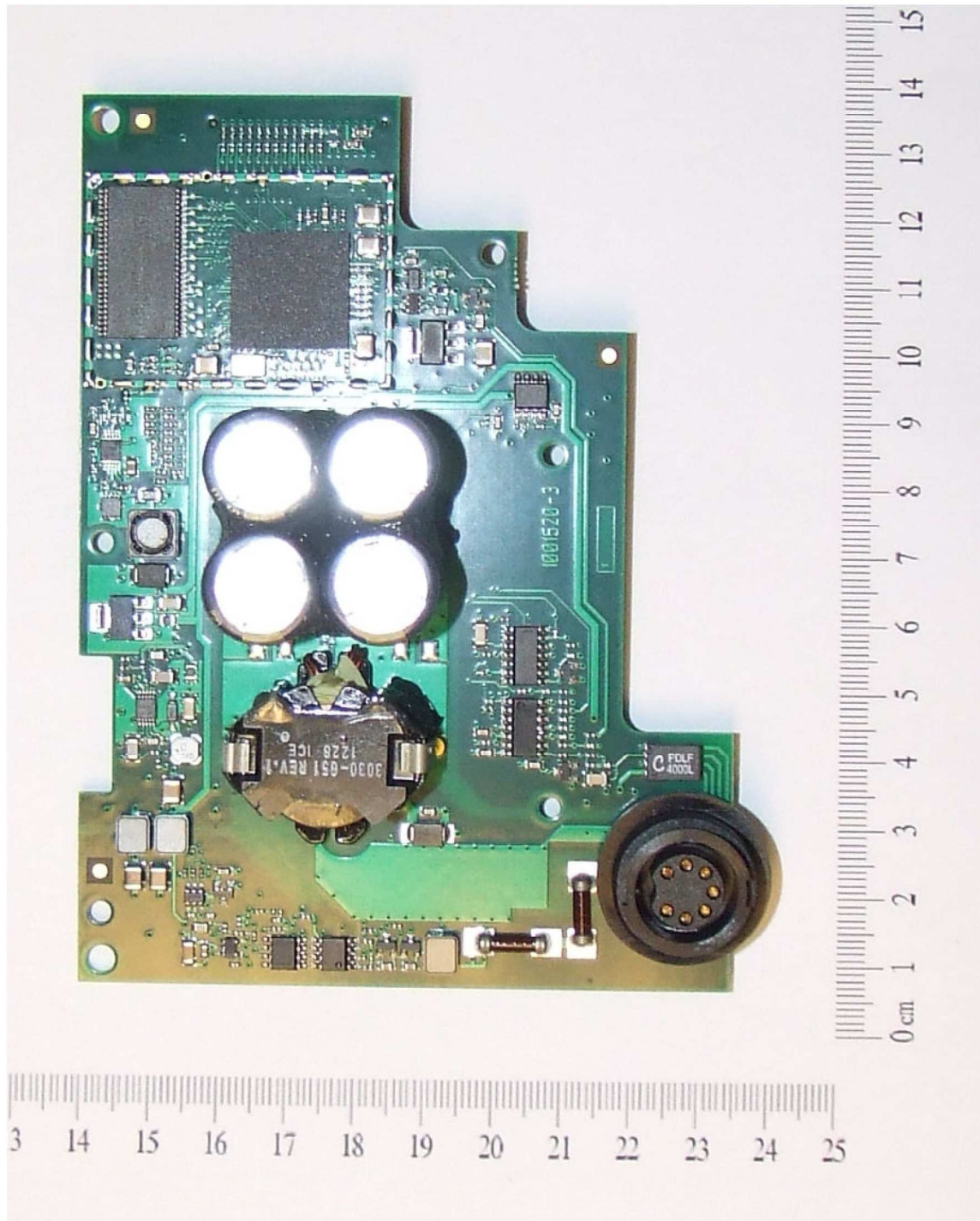
Figure 6 – a67 Sonar PCB (top)
