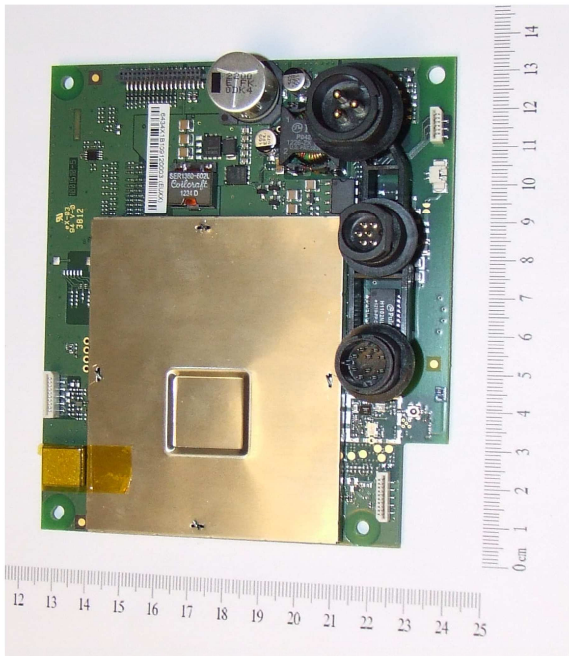
Figure 10 - CPU PCB (top)
