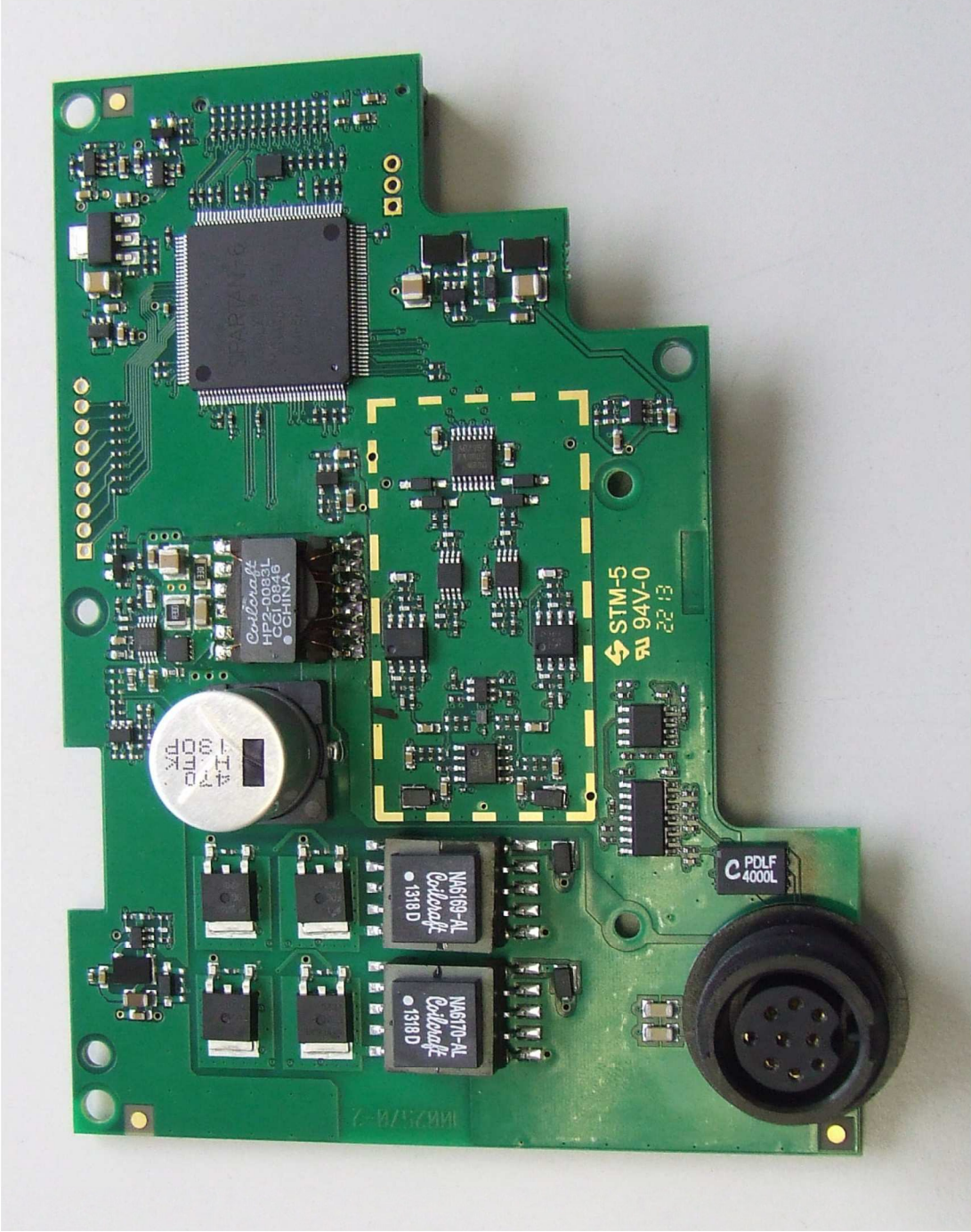
Figure 8 - a68 Sonar PCB (top)
