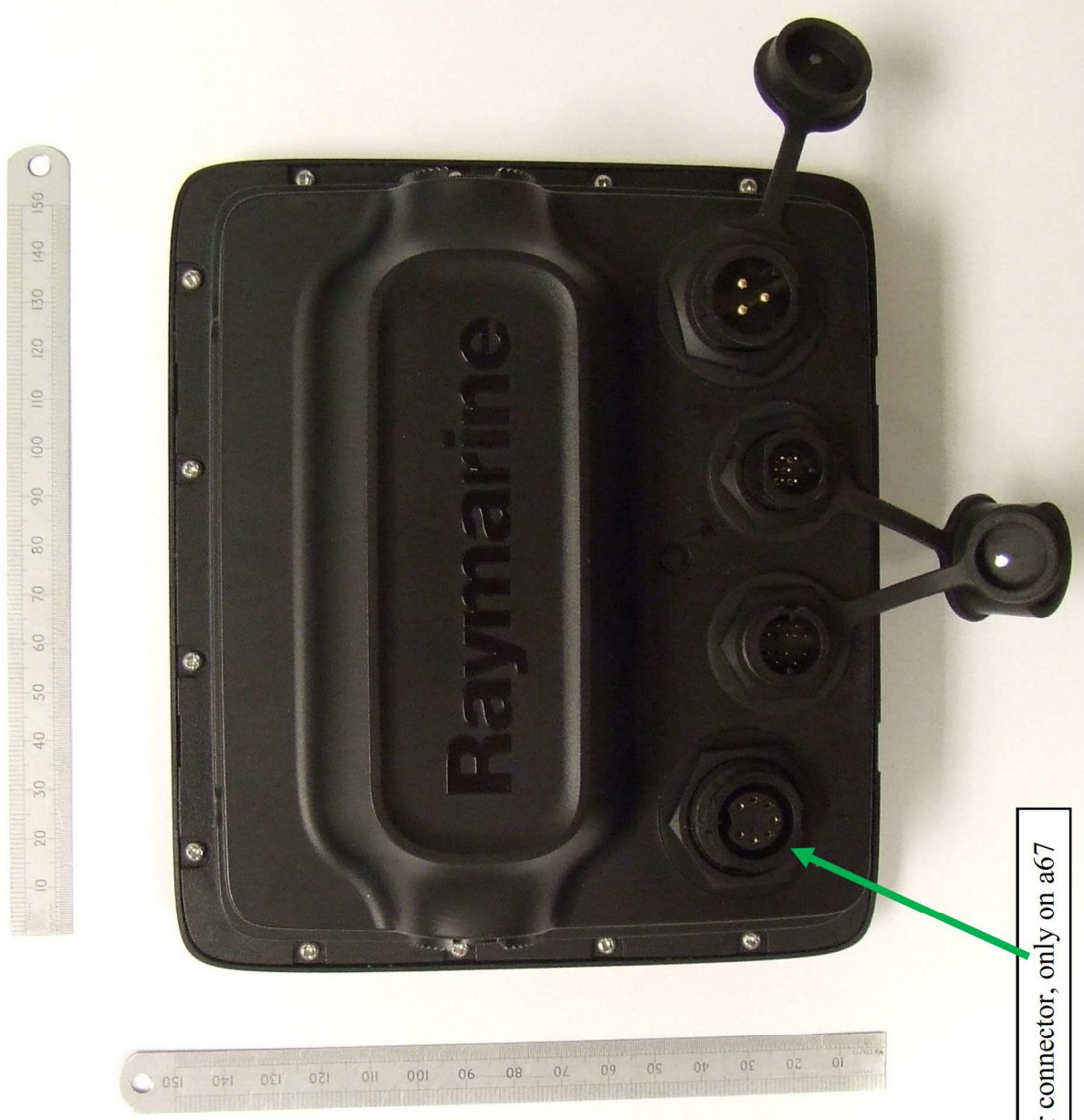
Figure 2 - Rear of A6
