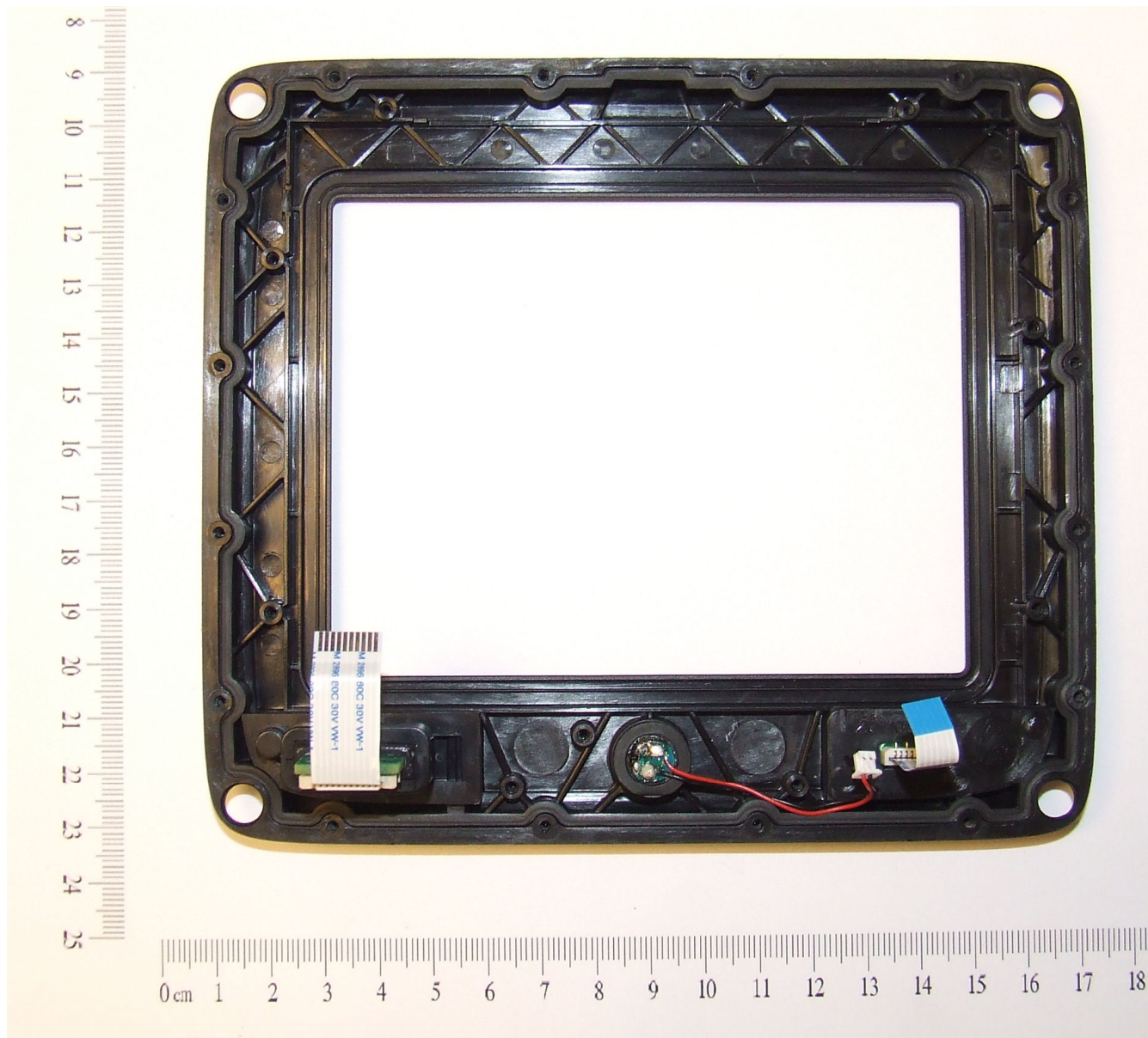
Figure 14 - Rear of front facia
