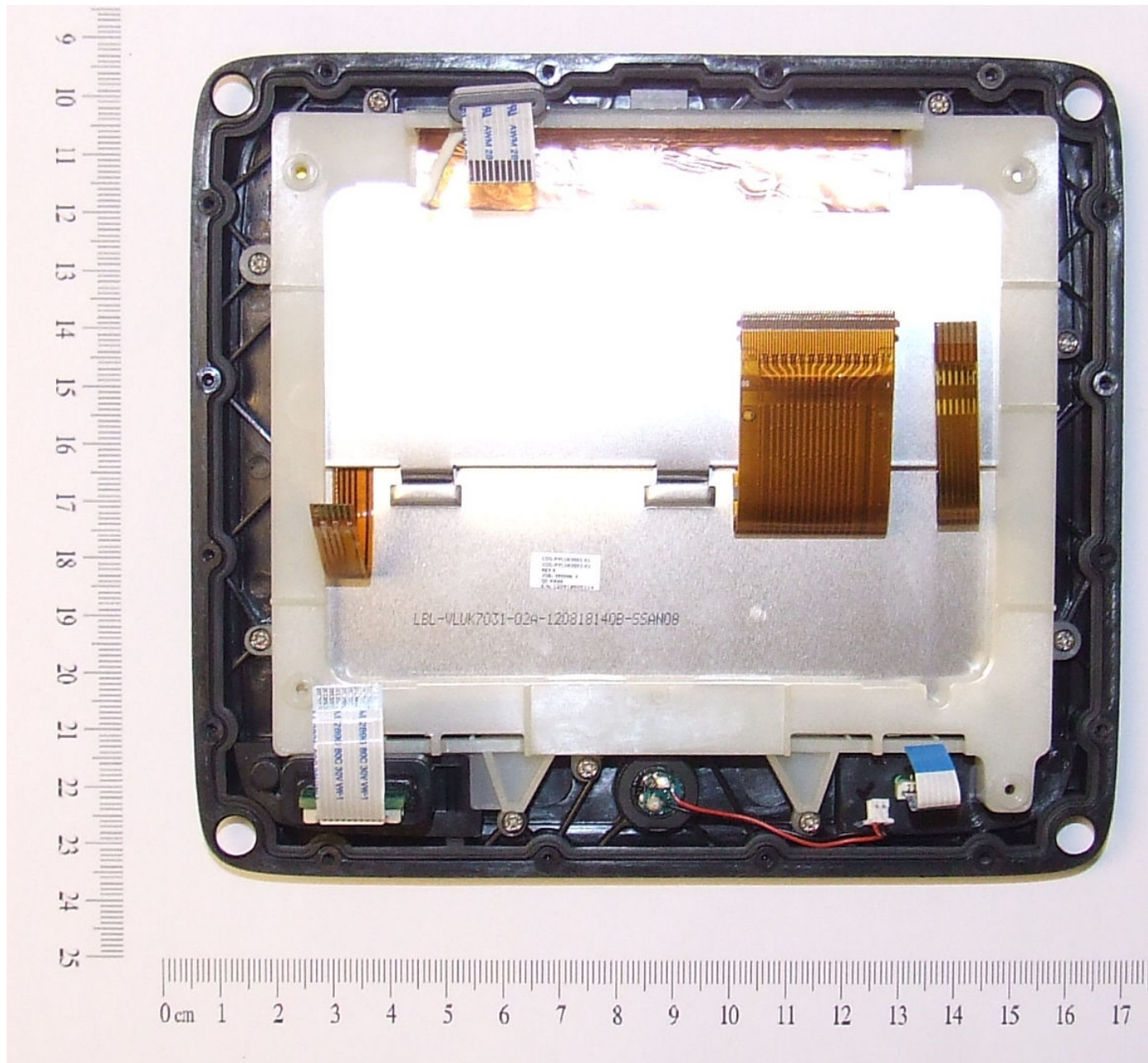
Figure 11 - Rear of LCD (CPU PCB removed)
