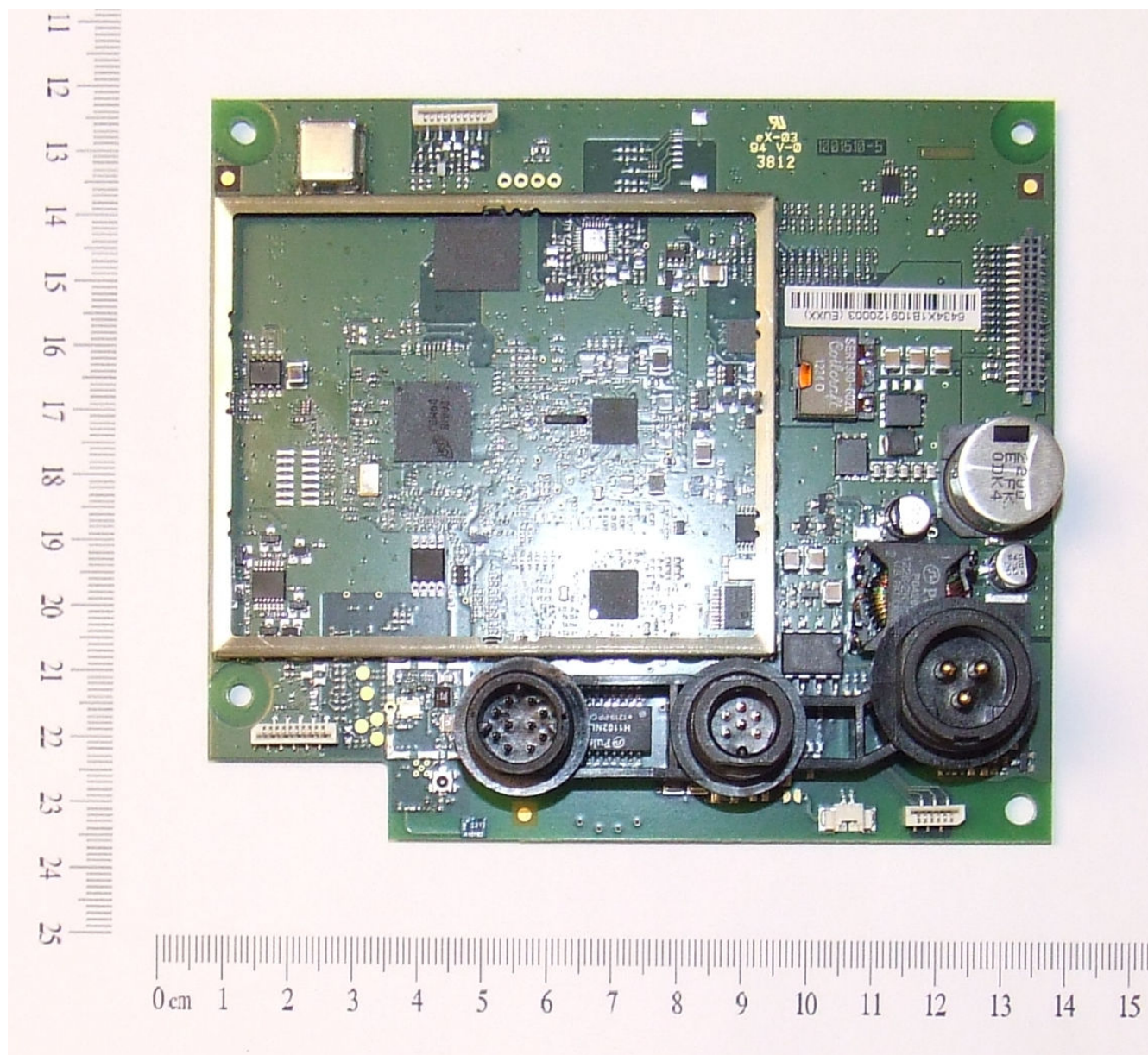
Figure 9 - CPU (top, CAN's removed)
