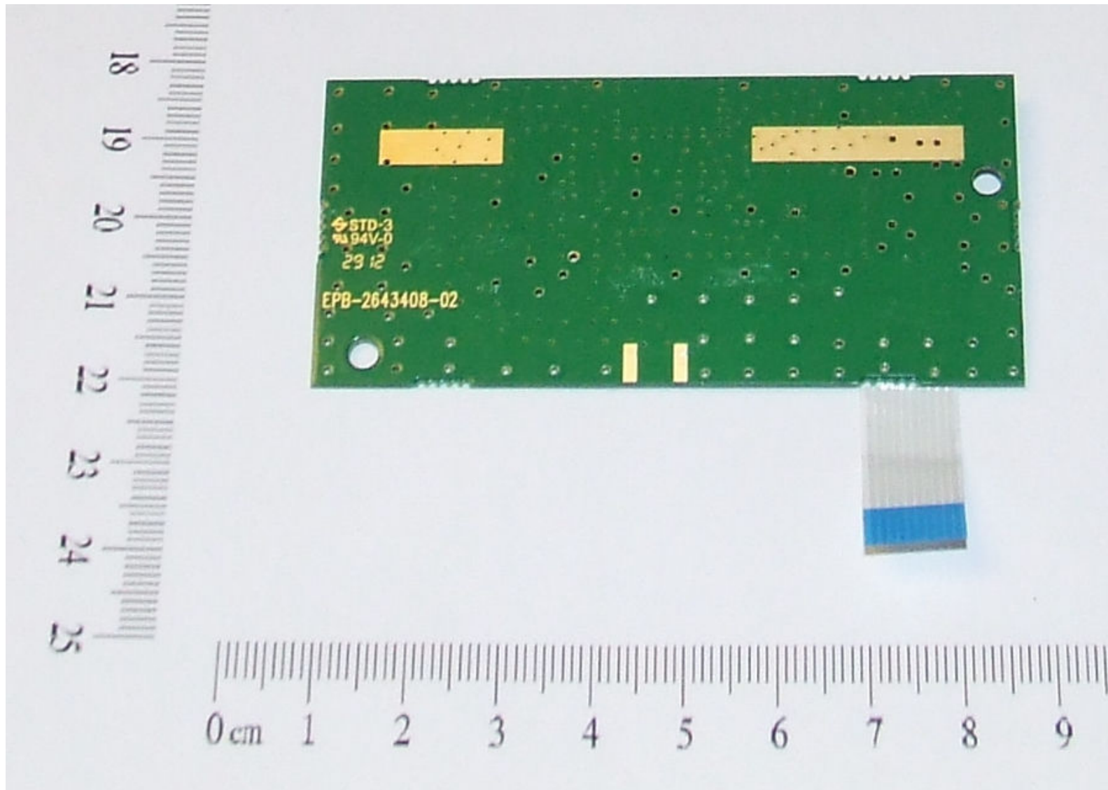
Figure 17 - GPS PCB (bottom)
