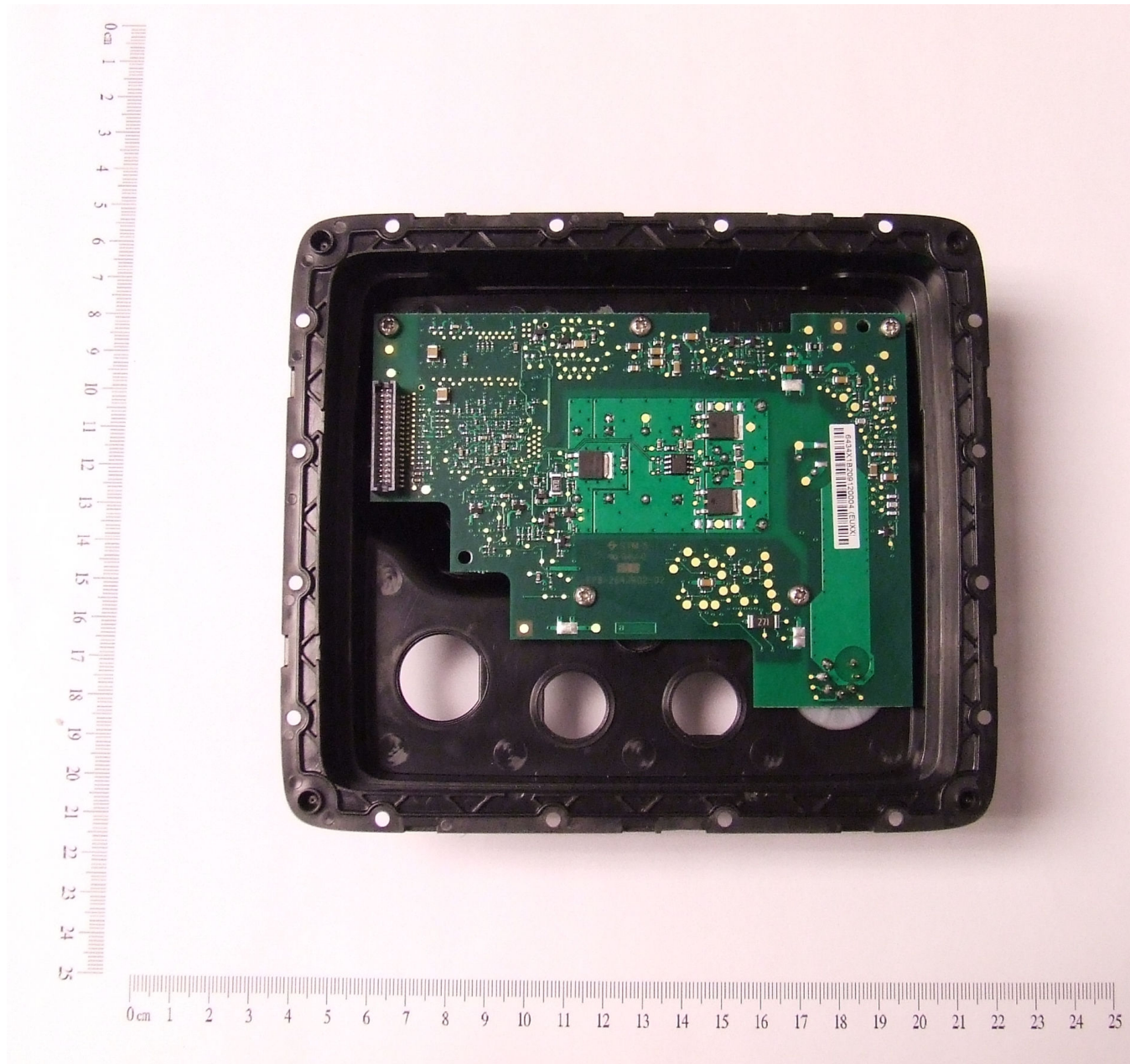
Figure 5 - Inside of A6 rear casing showing Sonar PCB (a67 only)
