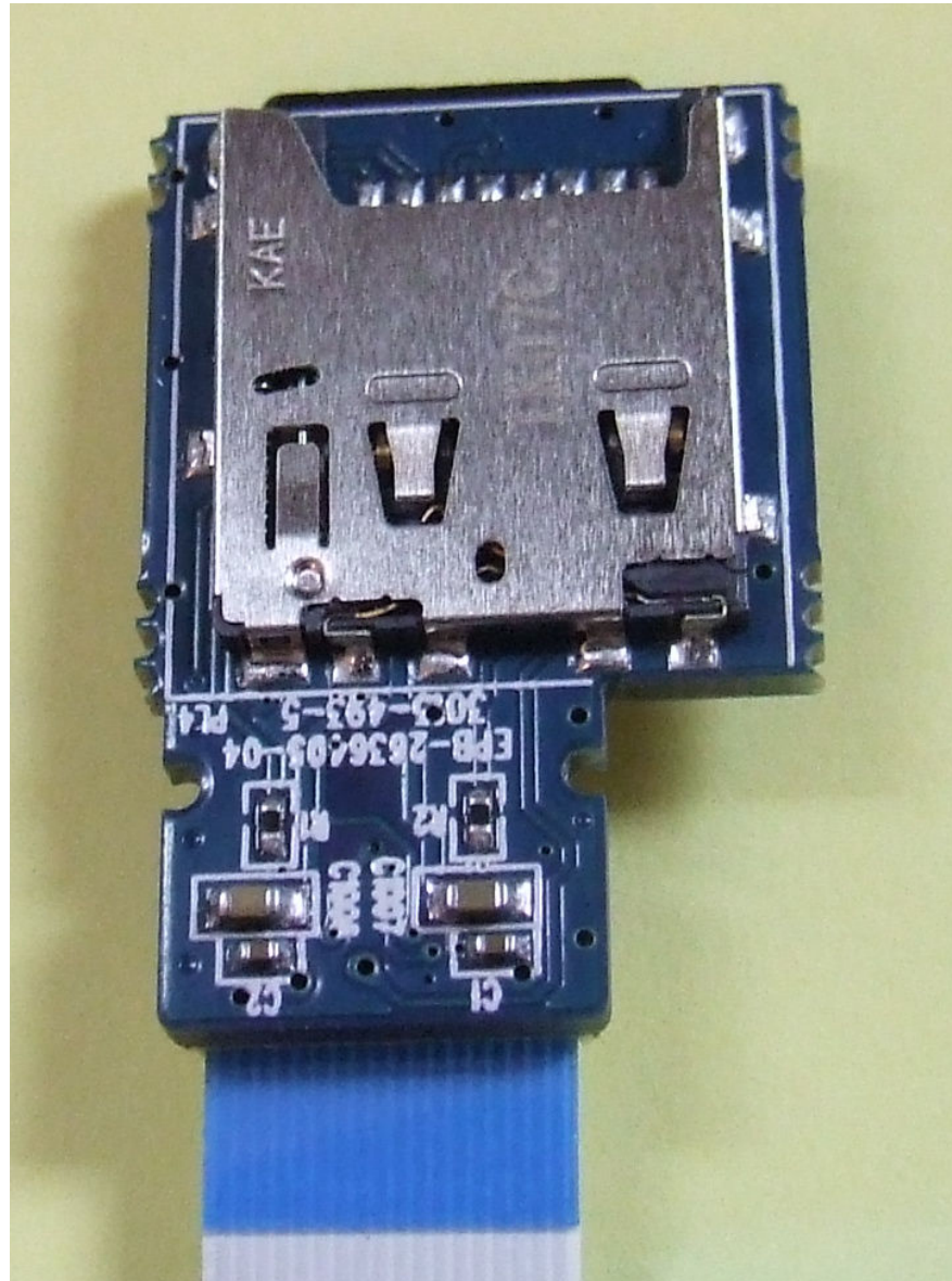
Figure 19 - Micro SD Reader (bottom)
