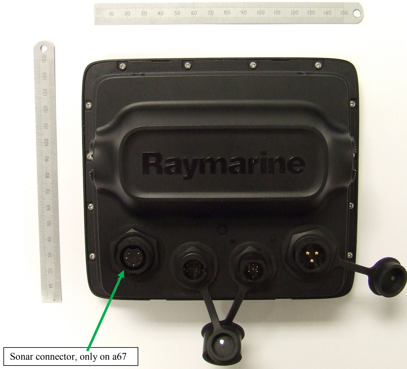
Figure 2 - Rear of A6
