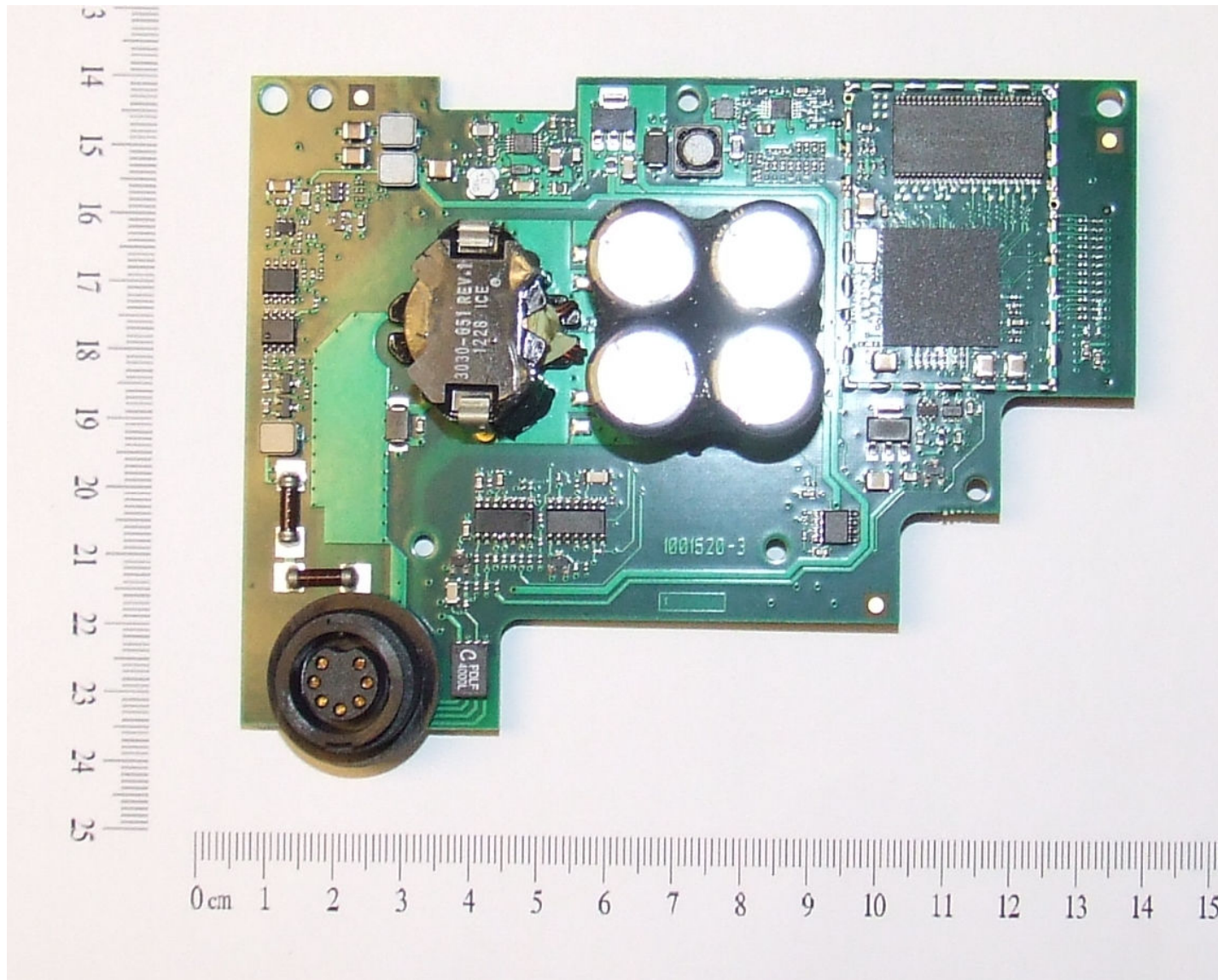
Figure 6 – a67 Sonar PCB (top)
