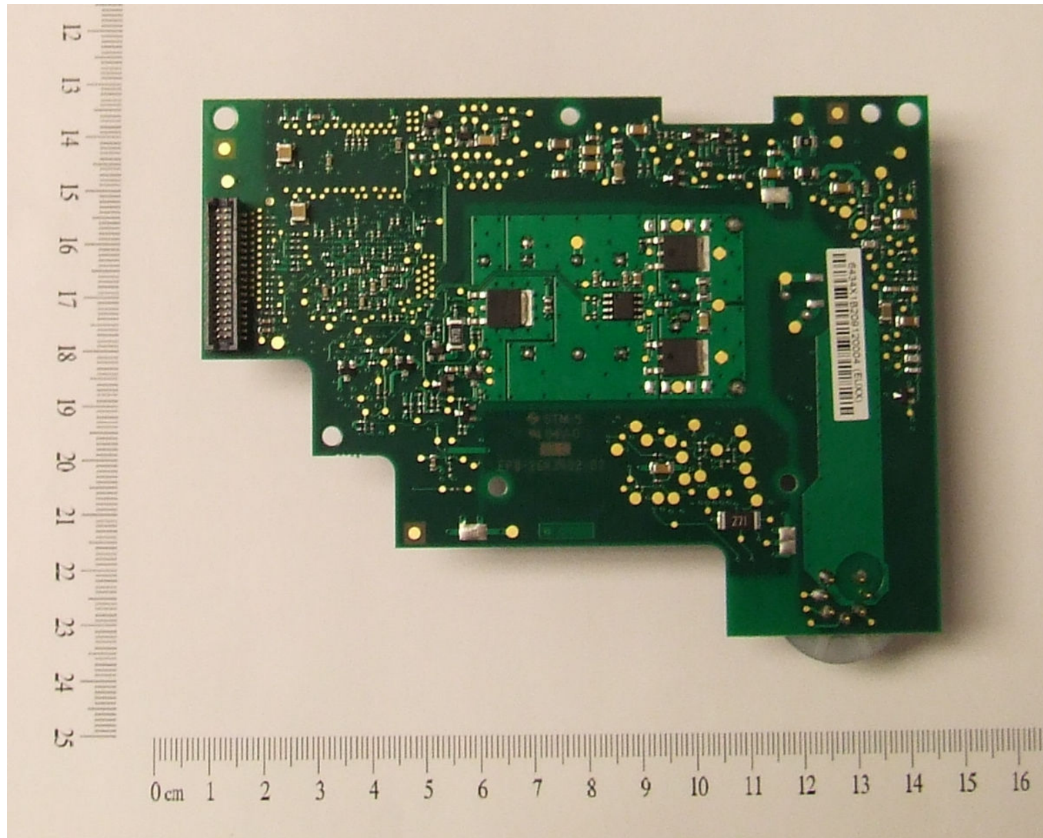
Figure 7 – a67 Sonar PCB (bottom)
