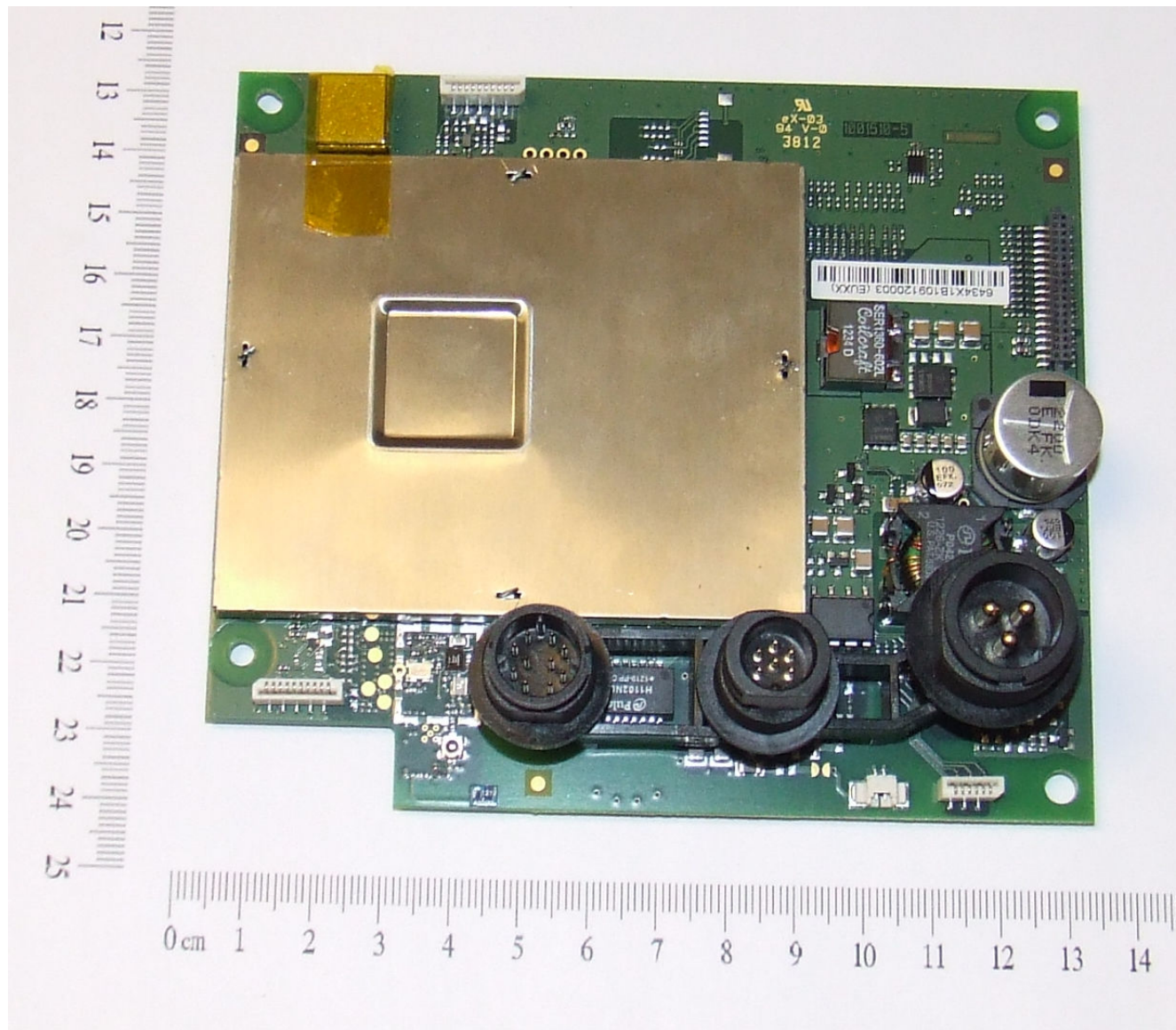
Figure 8 - CPU PCB (top)
