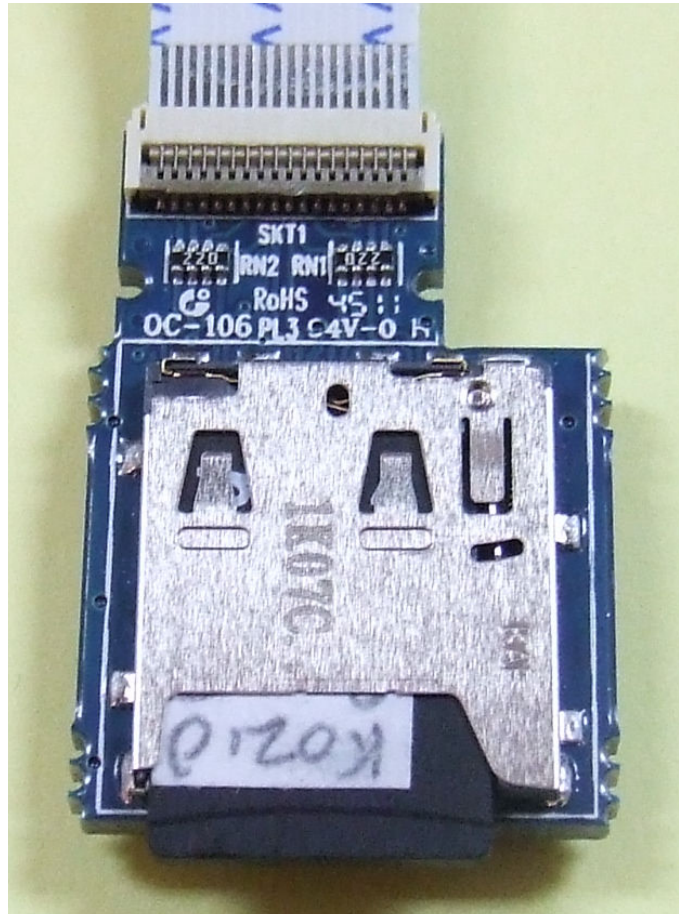
Figure 18 - Micro SD Reader (top)
