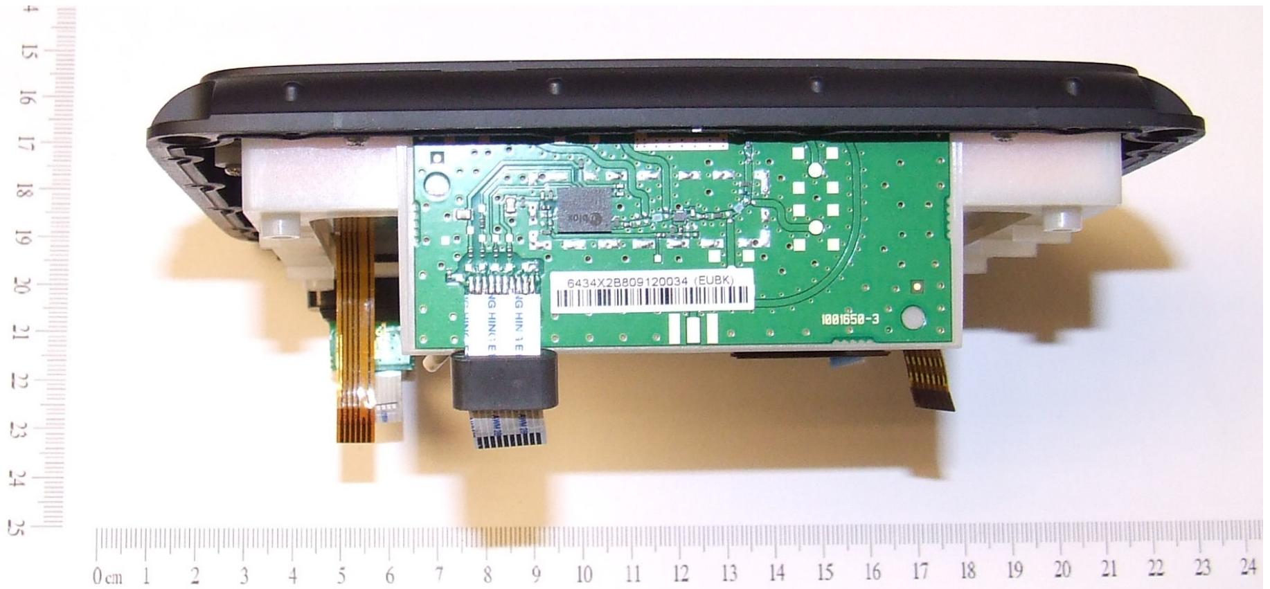
Figure 15 - GPS PCB (fitted)
