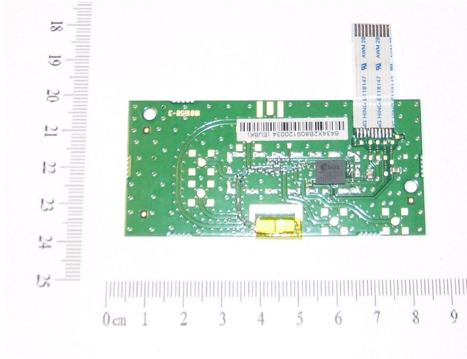
Figure 16 - GPS PCB (top)
