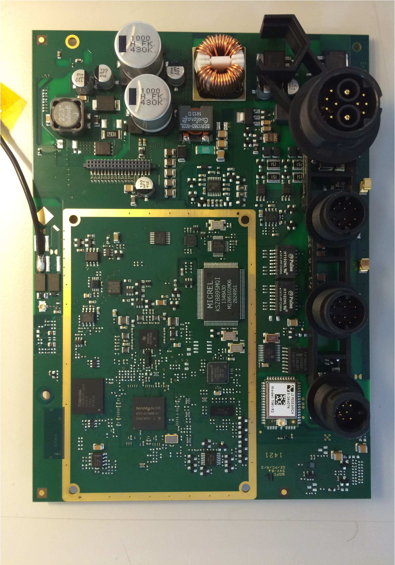
Figure 3 - CPU_PCBA_TOP
