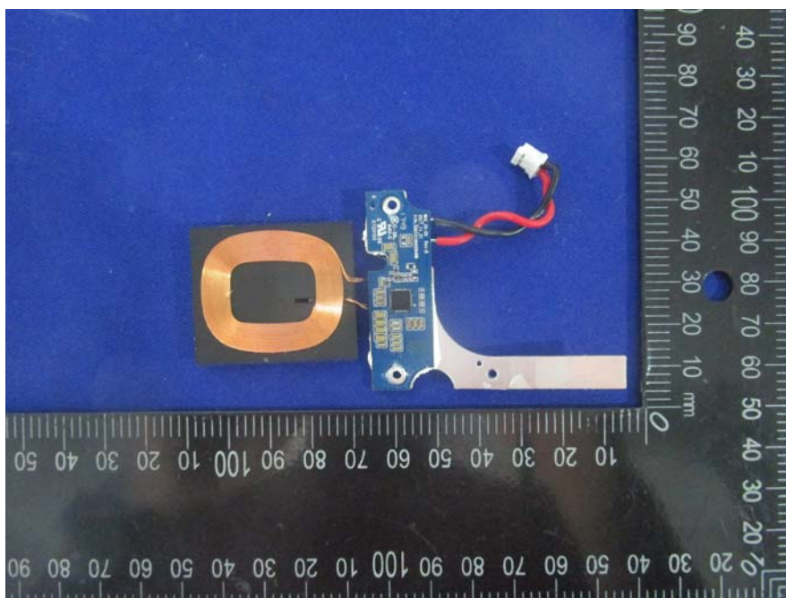
EUT –Wireless Charging Board Bottom View
