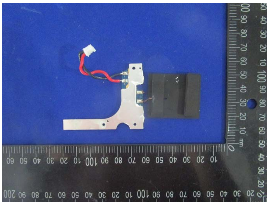
EUT –Wireless Charging Board Top View
