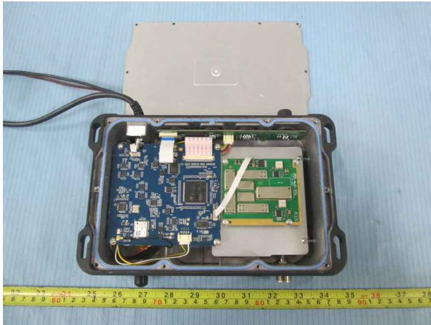
EUT (RAY91) – Cover off View 1
