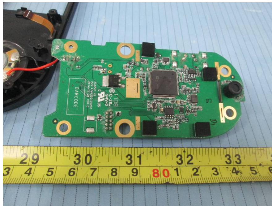
EUT (Handset) – Main Board Top Shielding off View
