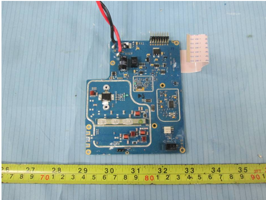
EUT– Main Board 5 Bottom Shielding off View
