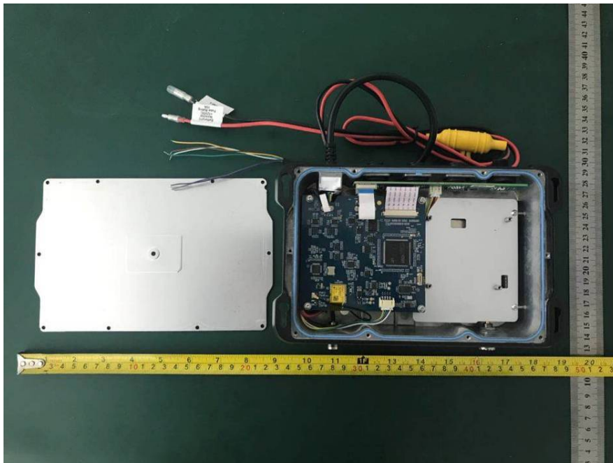
EUT (RAY90) – Cover off View 1
