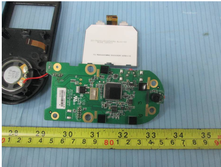
EUT (Handset) – Main Board Top View 2
