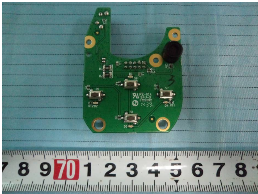
EUT –Microphone Main Board Top View
