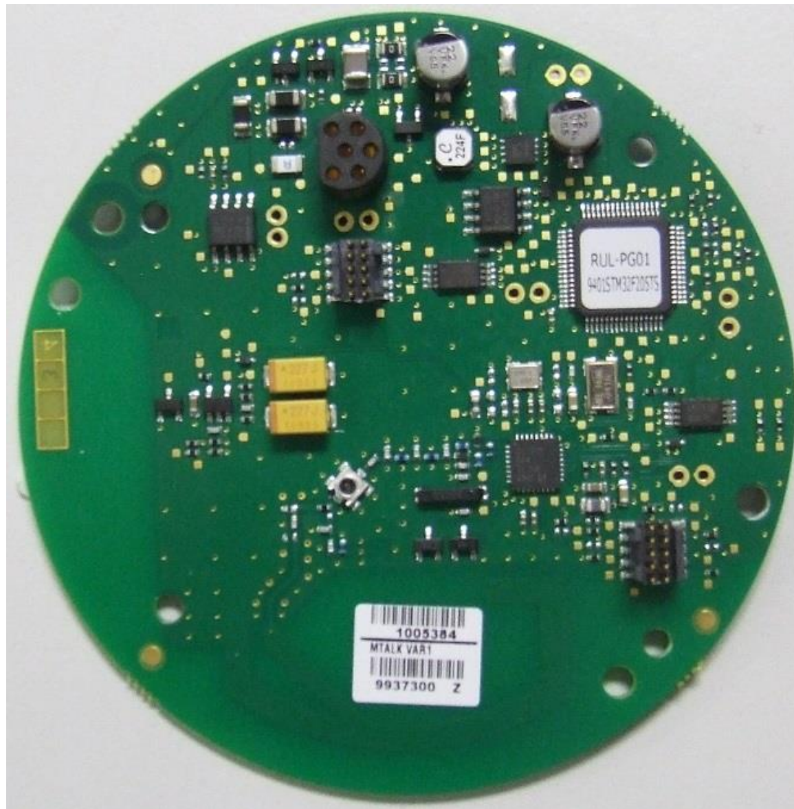
PCB rear
