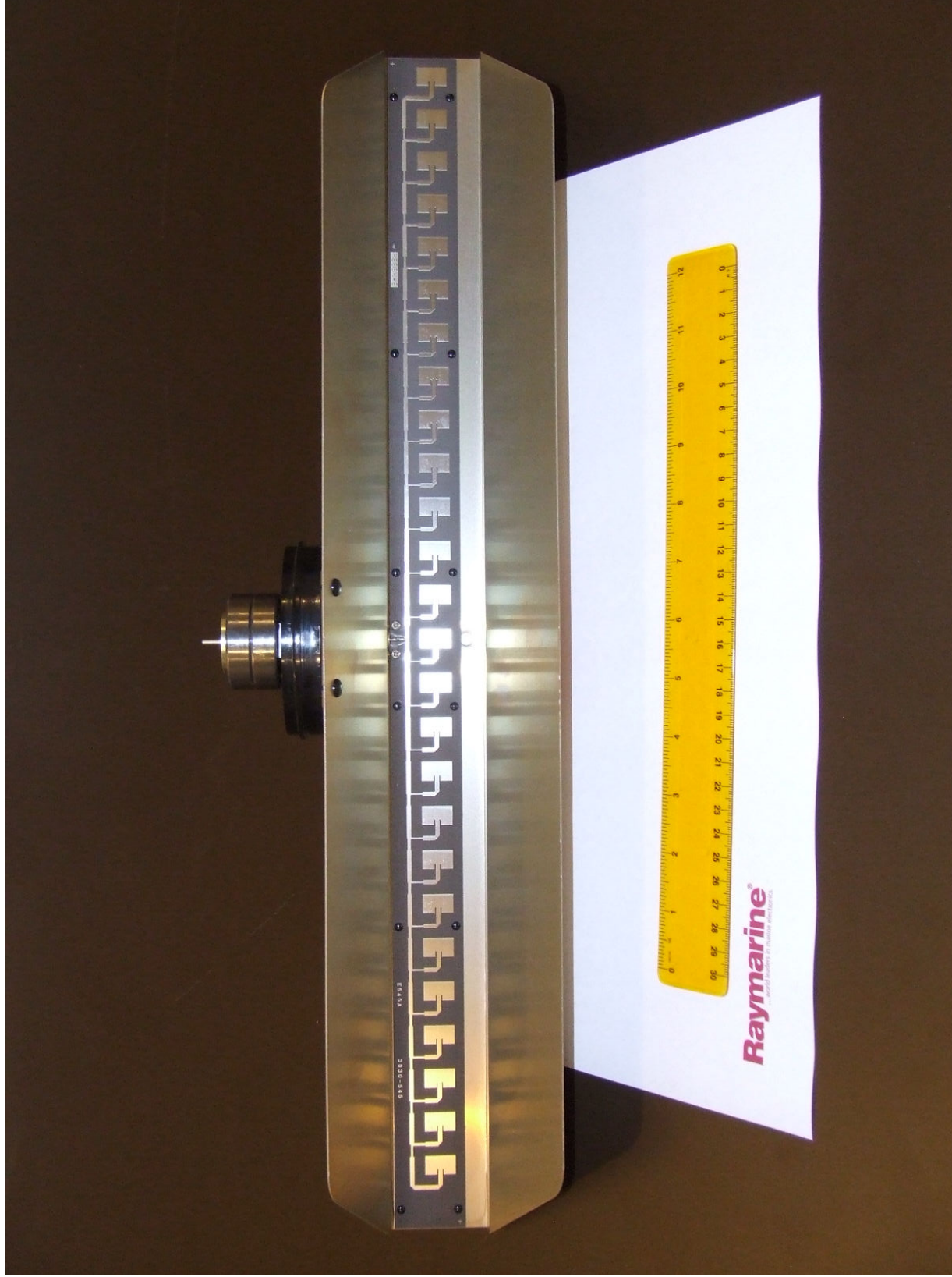
Figure 5 - RD424 Antenna Front
