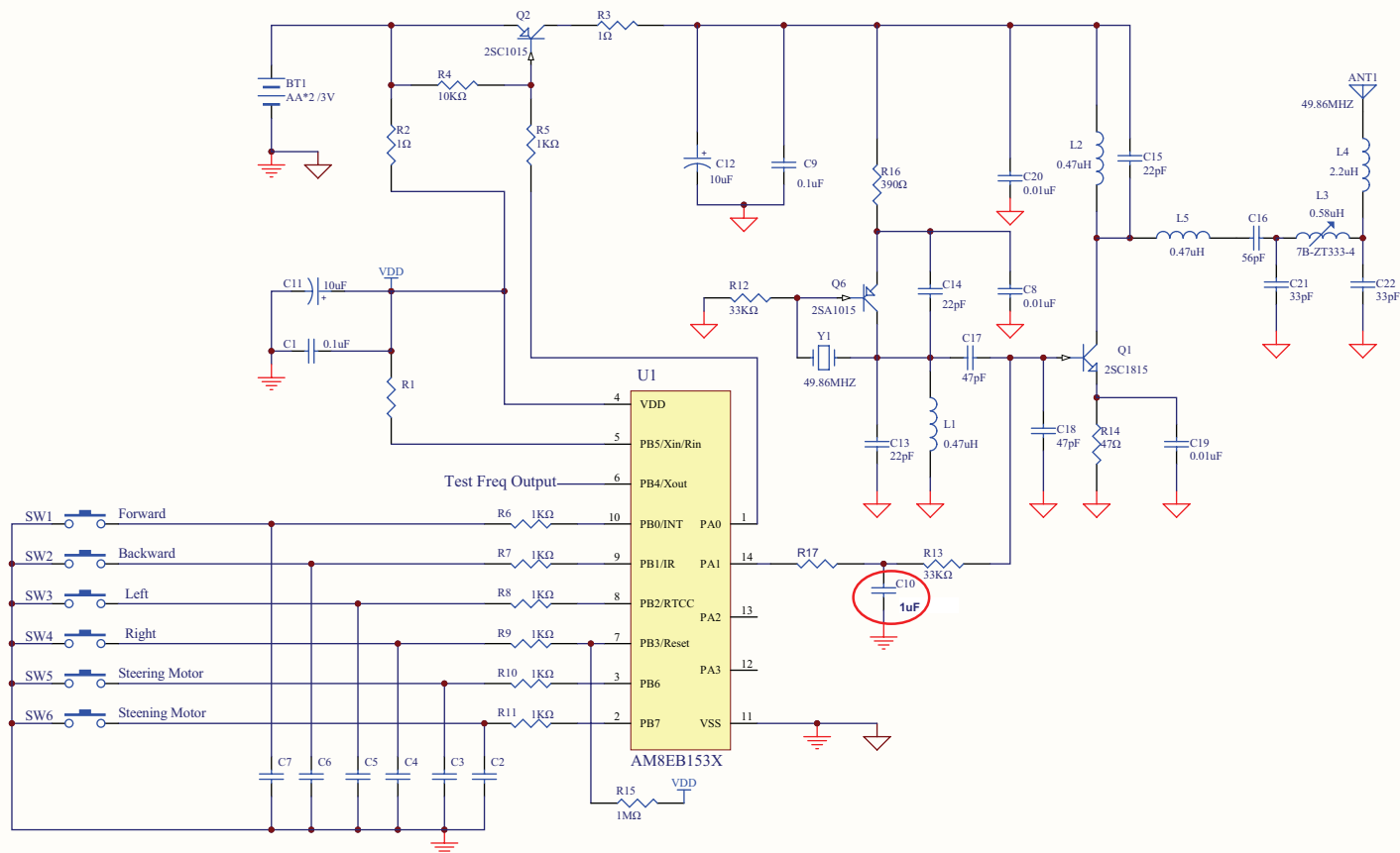
Transmitter schematic diagram
