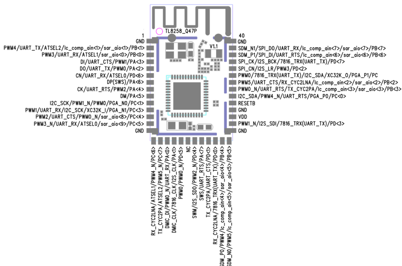
Figure 2-1 Pin assignment for MBTEL1
