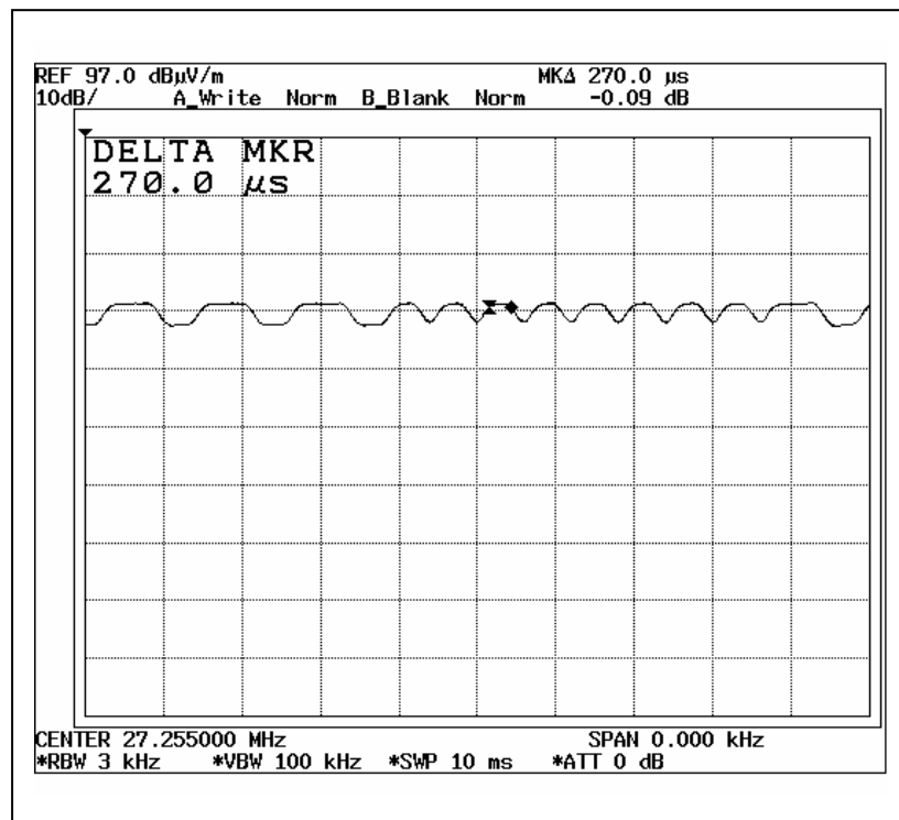
Duty Cycle 3
