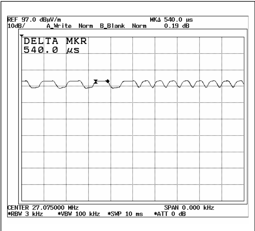
Duty Cycle 2
