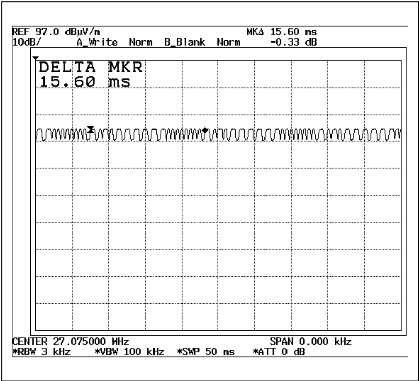
Duty Cycle 1
