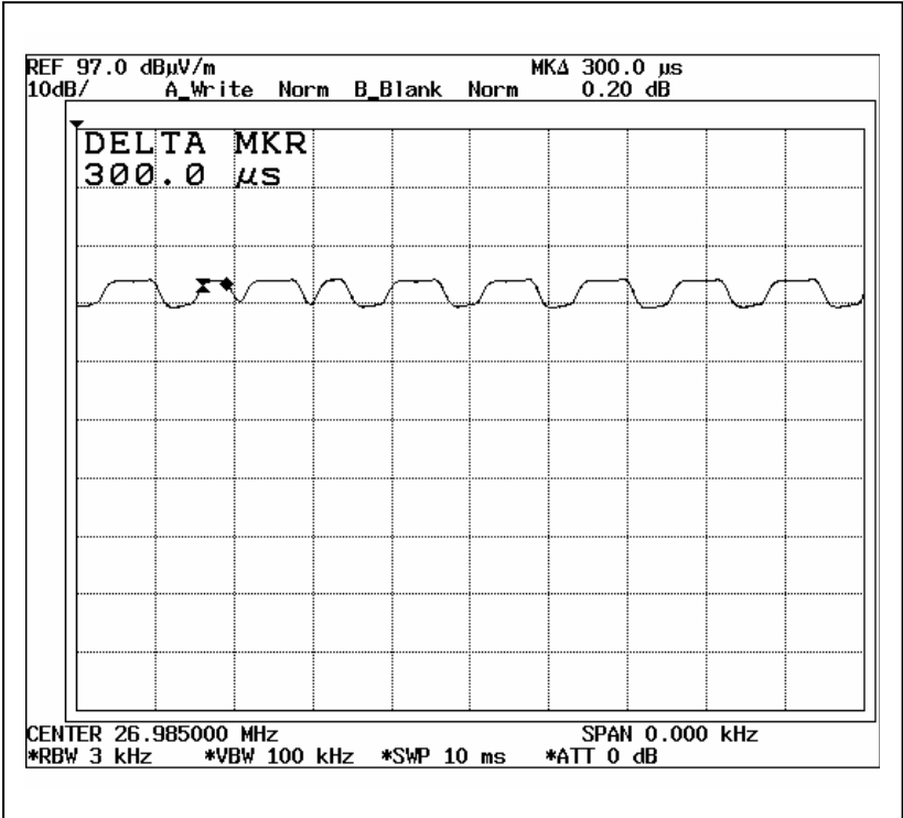
Duty Cycle 3
