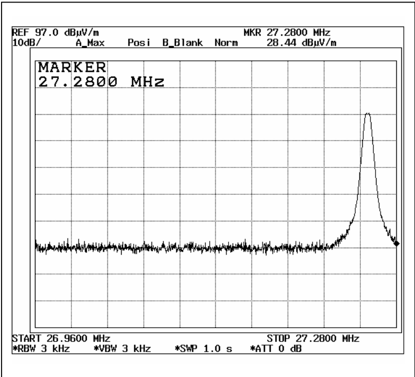
Bandwidth 2 (Channel 8)
