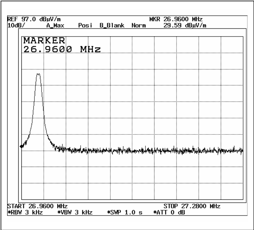
Bandwidth Plot
