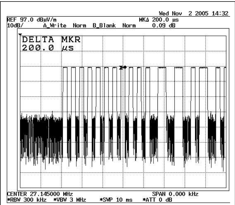
Duty Cycle 2
