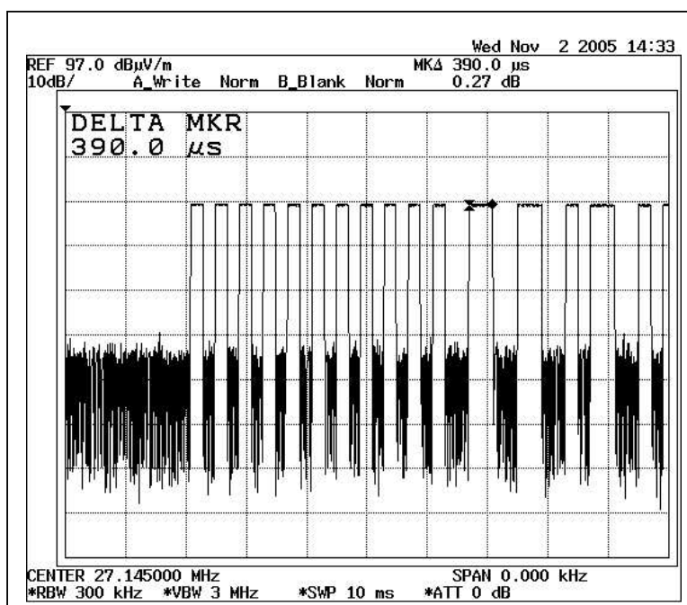
Duty Cycle 3
