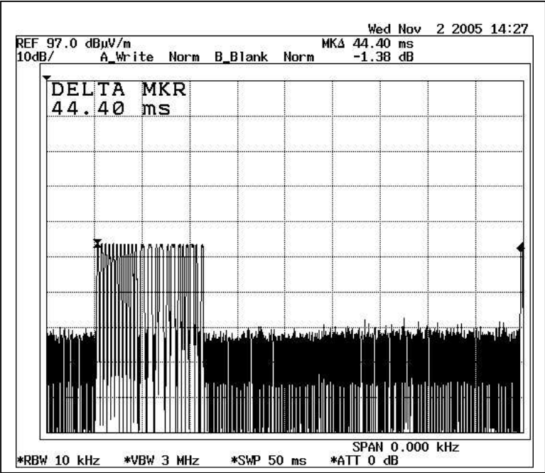
Duty Cycle 1
