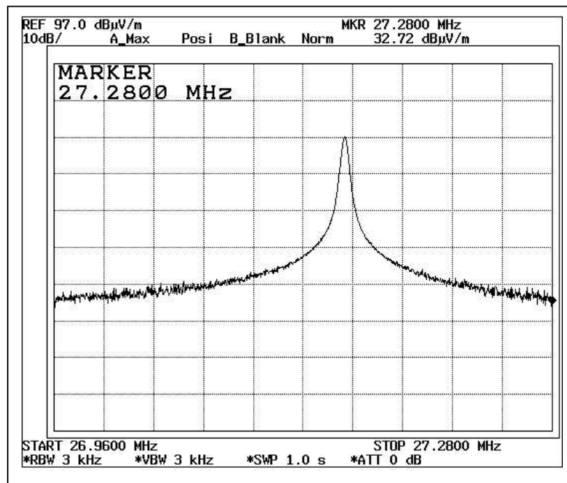
Bandwidth Plot
