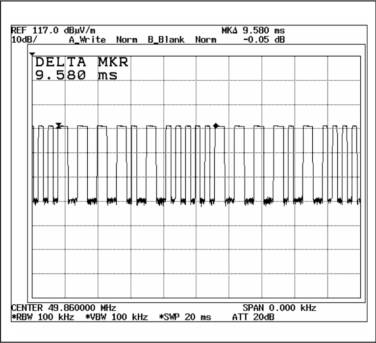
Duty Cycle
