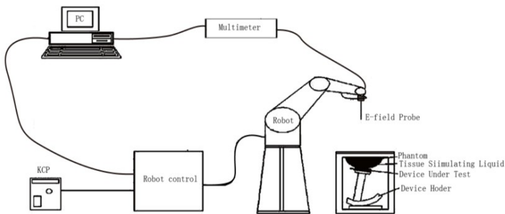
Figure 1: Schematic diagram of the SAR measurement system
