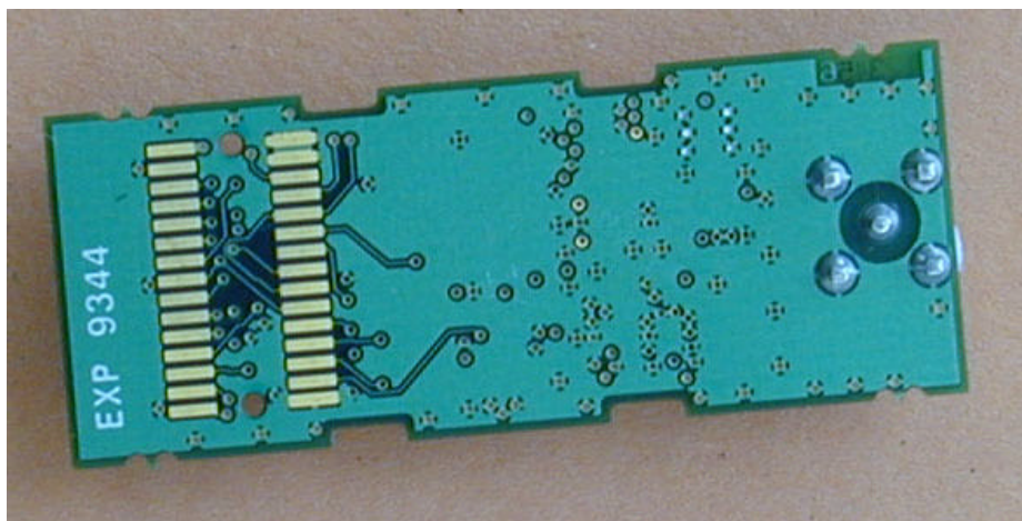
Module – Bottom View.
