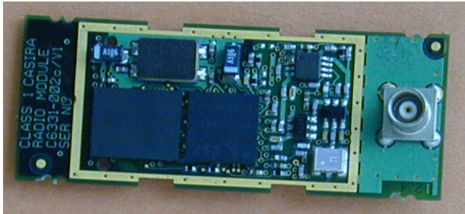
Module – Top View.
