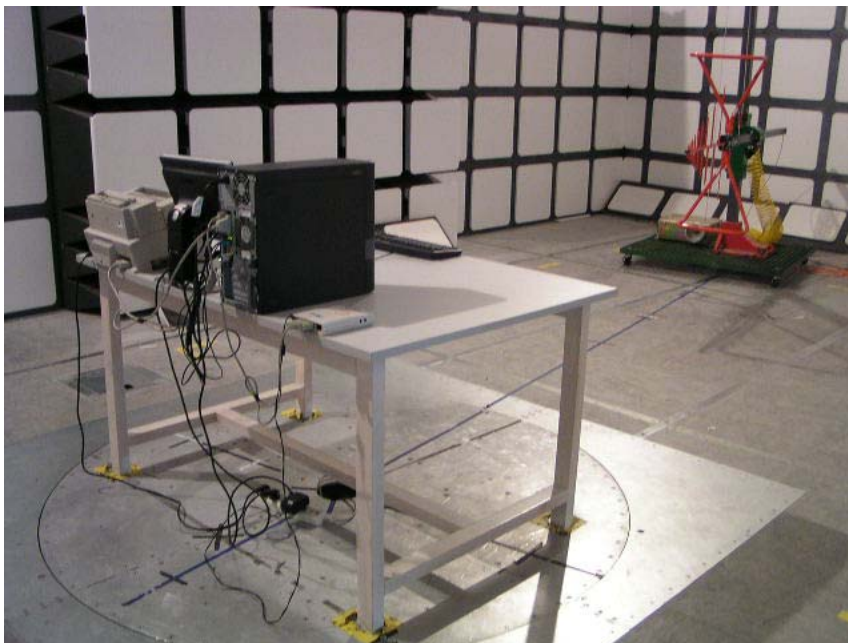
USB KEY 1 K: Radiated Emissions-Rear View (1)
