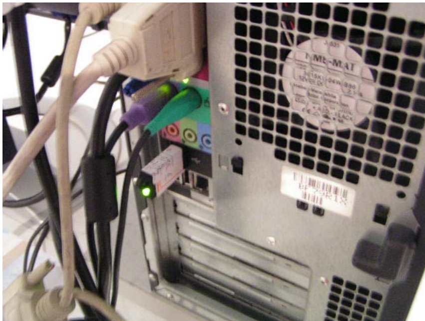
USB KEY 8 K: Radiated Emissions-Rear View (2)
