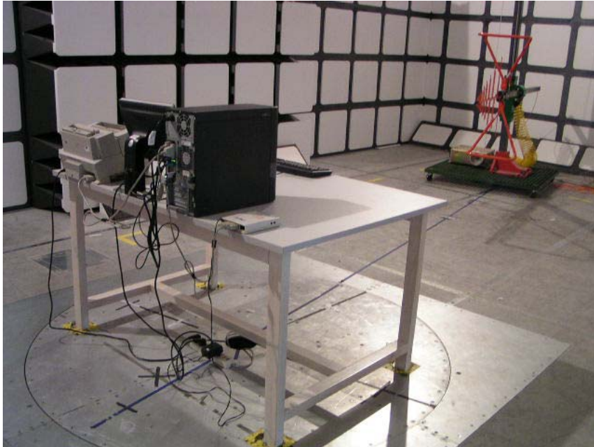
USB KEY 8 K: Radiated Emissions-Rear View (1)
