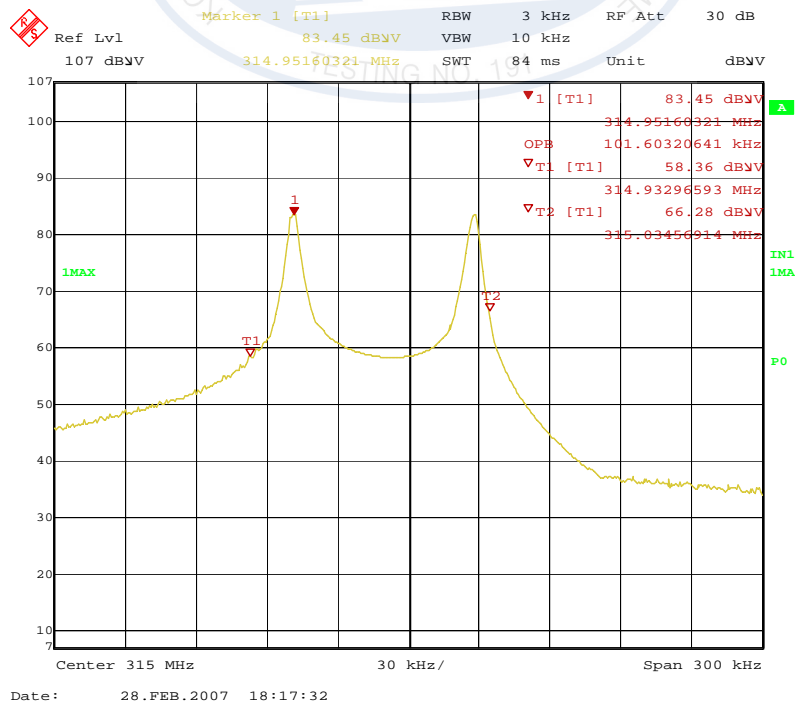
Figure 3: Measured value of the Occupied bandwidth(99 % Bandwidth)
