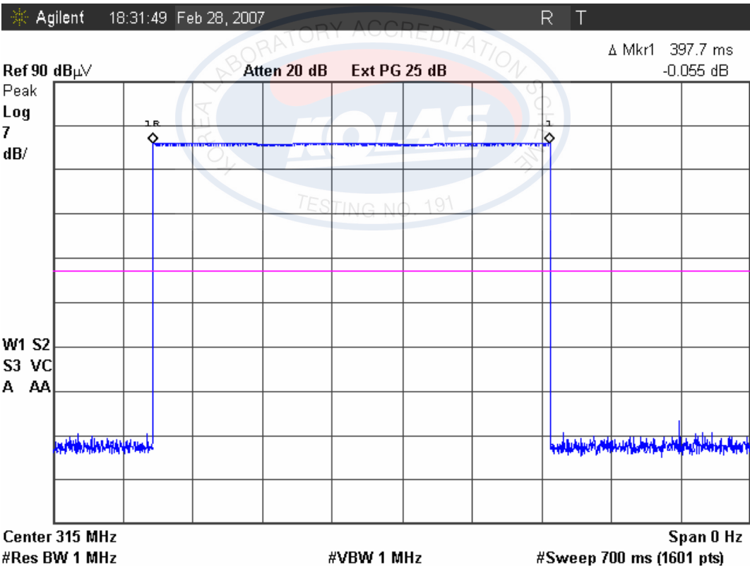
Figure 1: Measured value of the transmission duration
