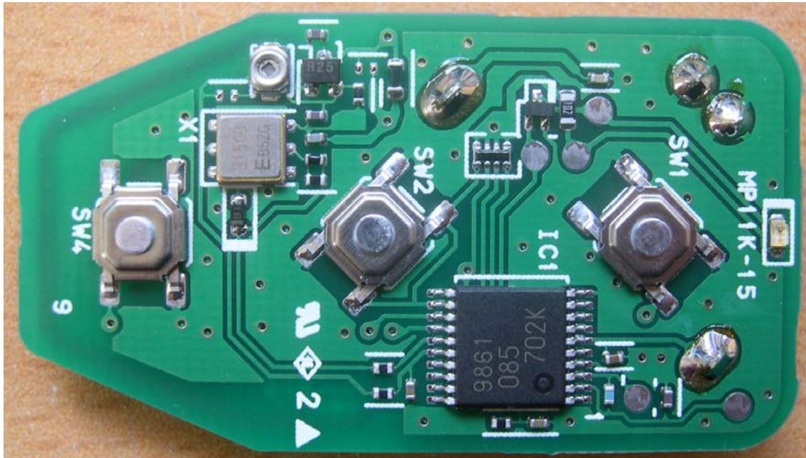
<Photograph 2: RF Board Front View>
