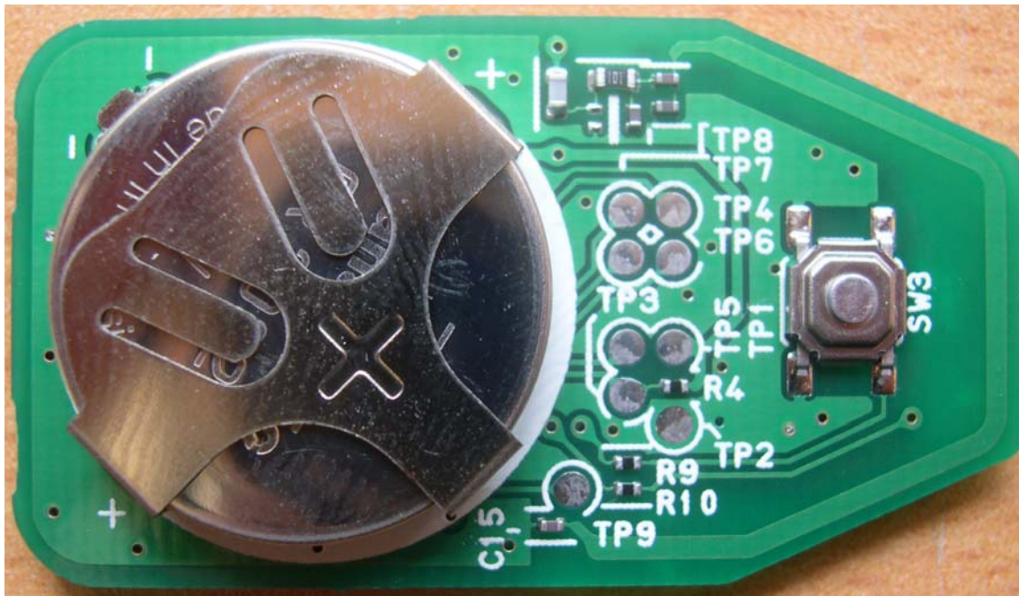
<Photograph 3: RF Board Rear View >
