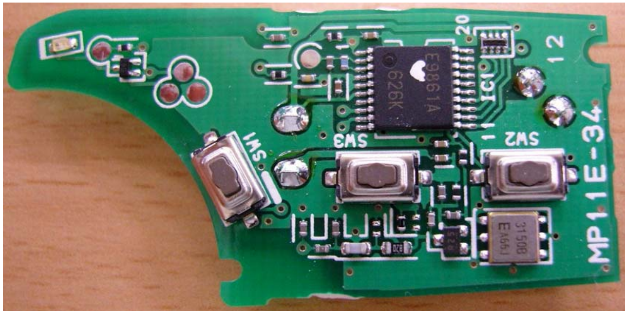
<Photograph 2: RF Board Front View>
