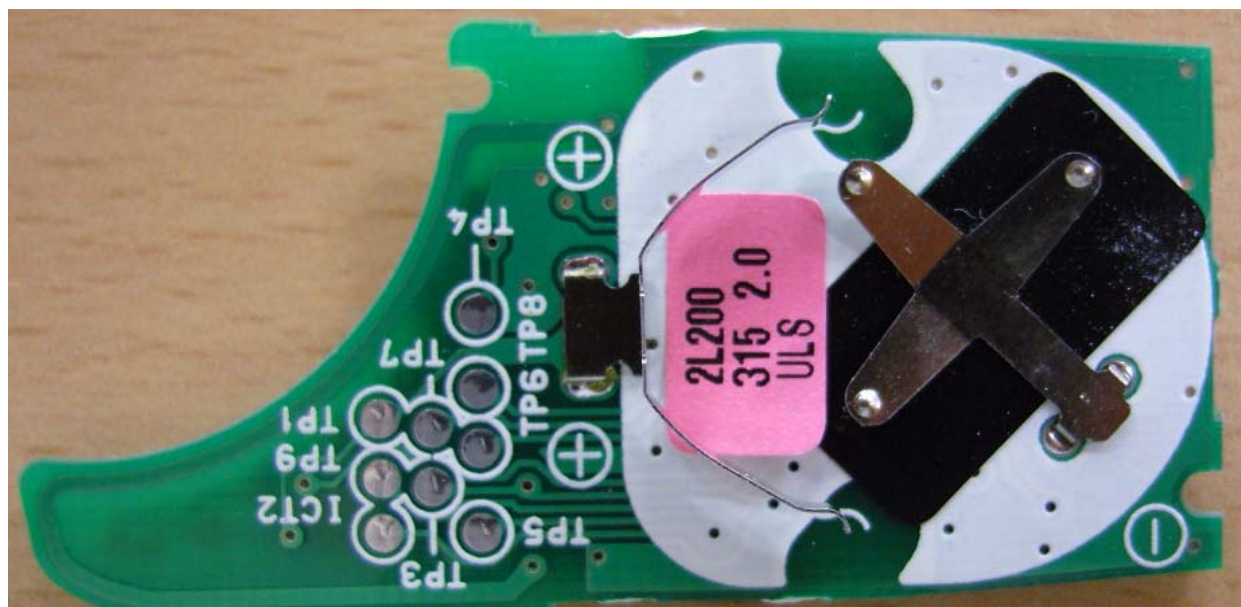
<Photograph 3: RF Board Rear View >
