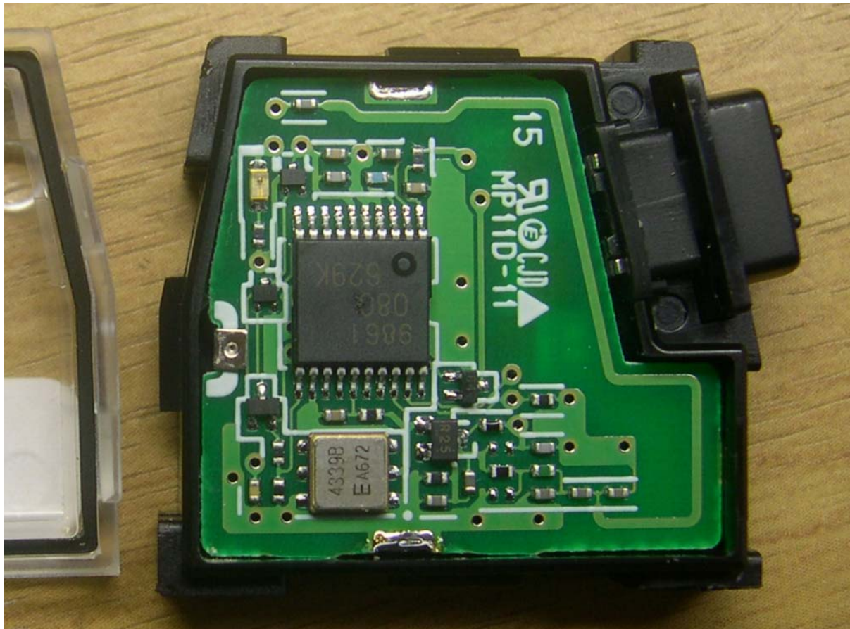
<Photograph 4: RF MODULE Internal View >
