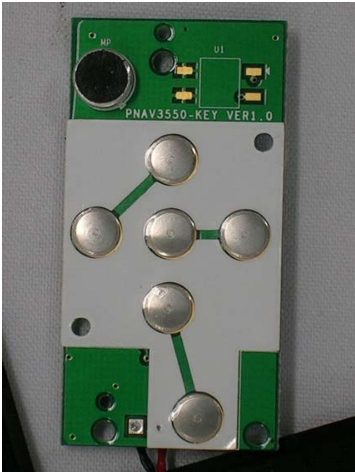
<FRONT VIEW OF KEYPAD BOARD>
