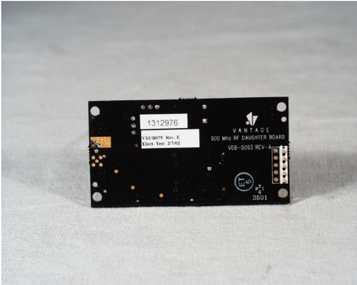
Bottom View of The VSUB075(REV A1)
