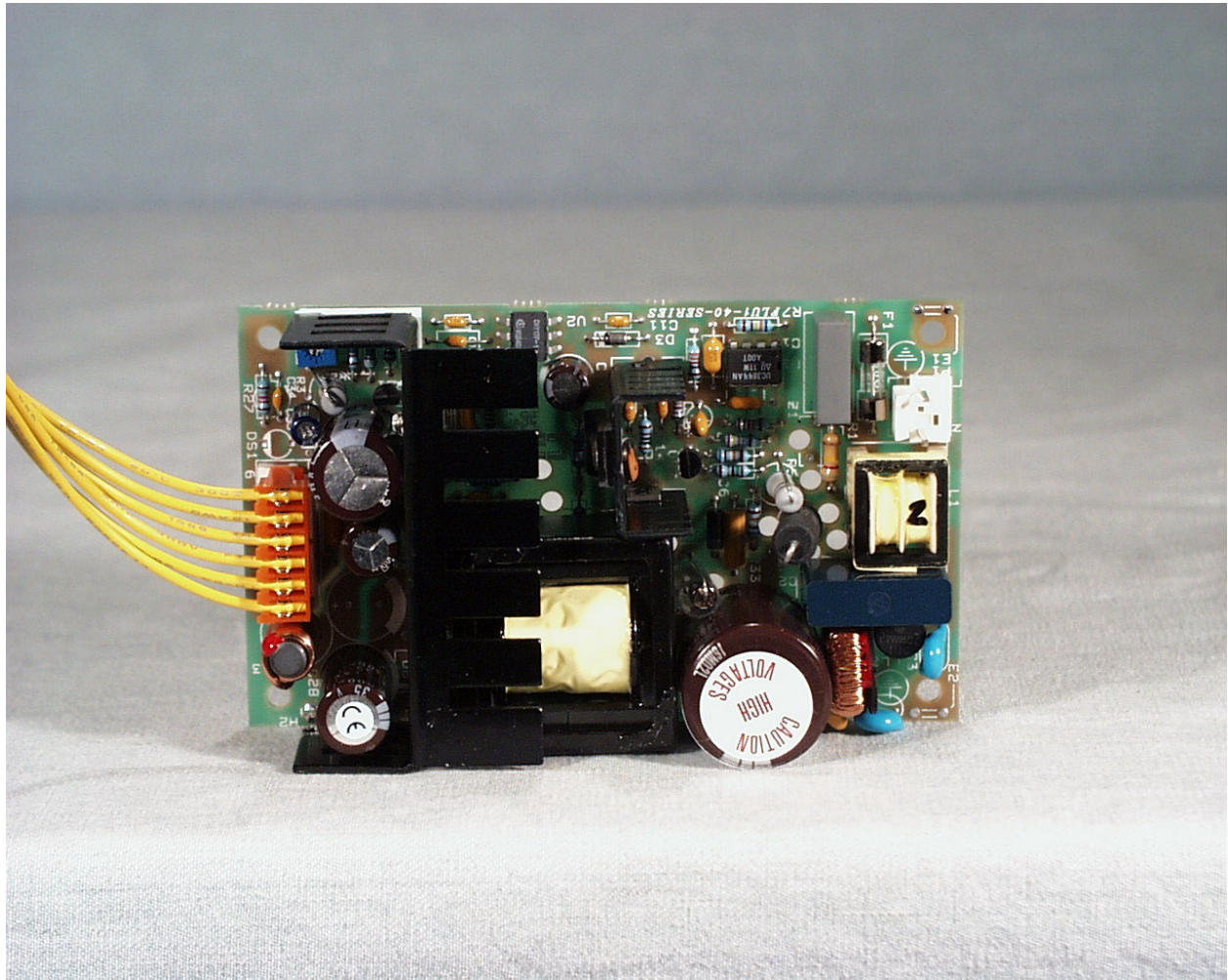
Front View of the 12 Volt Power Supply Board
