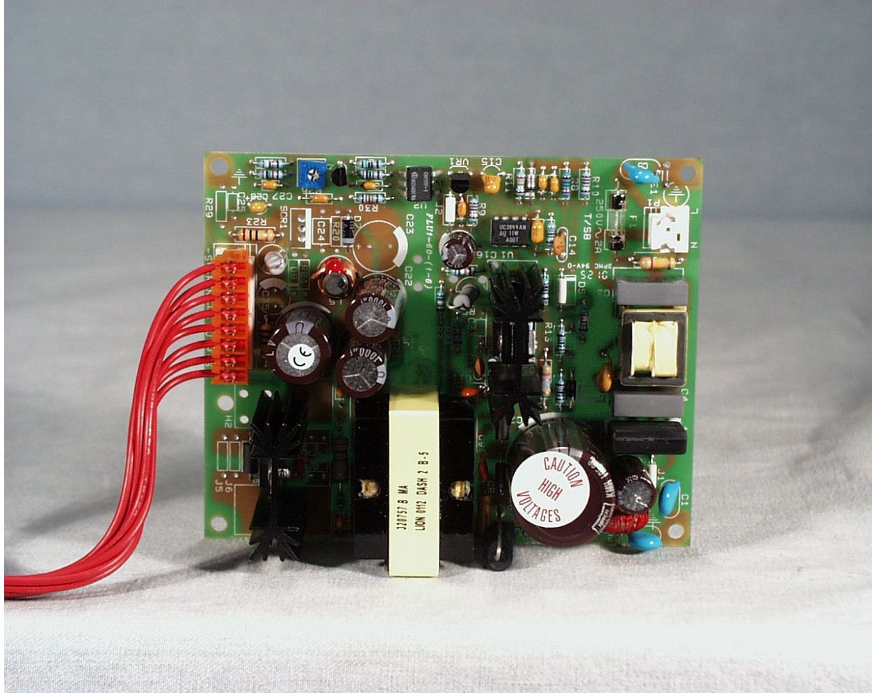
Front View of the 24 Volt Power Supply Board
