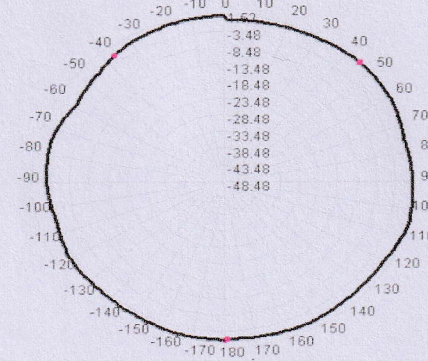
910.0MHz Total(E2-YZ), Max= 1.52dBi
