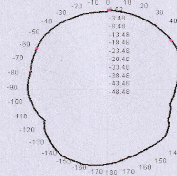
910.0MHz Total(E1-XZ), Max= -0.11dBi
