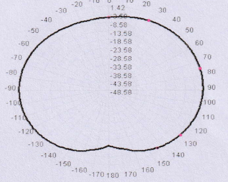
Total(H-XY), Max= 0.40dBi, CirD=16.01
