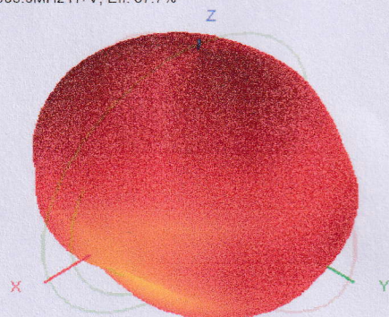
900.0MHz H+V, Eff: 67.7%
