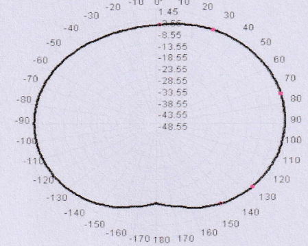
Total(H-XY), Max= 0.59dBi, CirD=14.33
