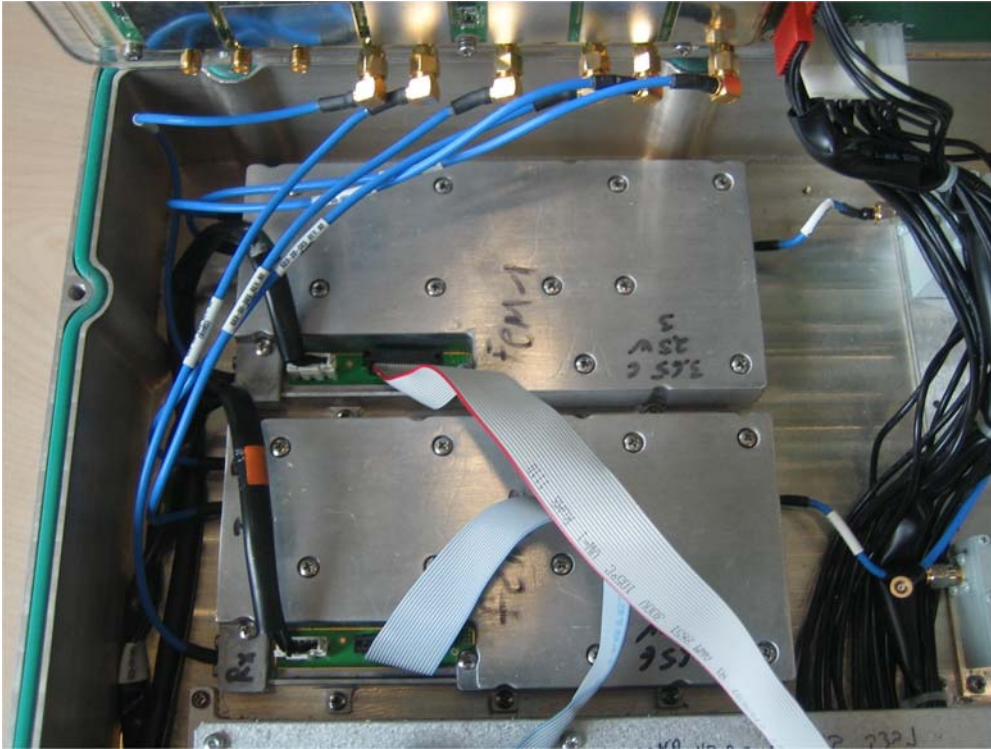
Photograph No.7 “uMAXe/AirGrid 3.65 GHz” RF power amplifiers
