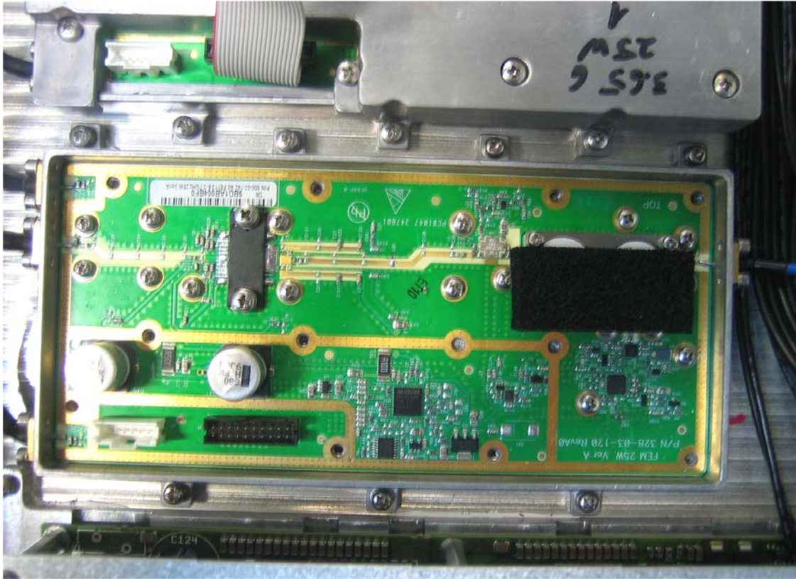
Photograph No.8 RF power amplifier internal view
