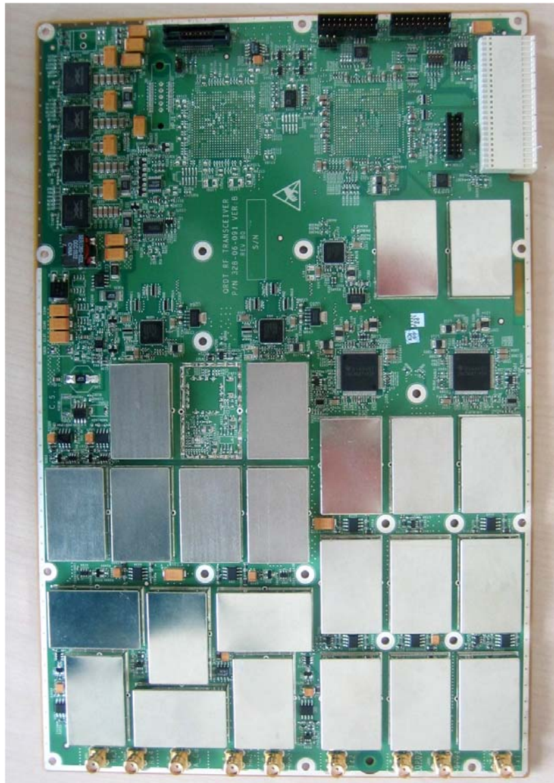
Photograph No.2 “uMAXe/AirGrid 3.65 GHz” RF card front view
