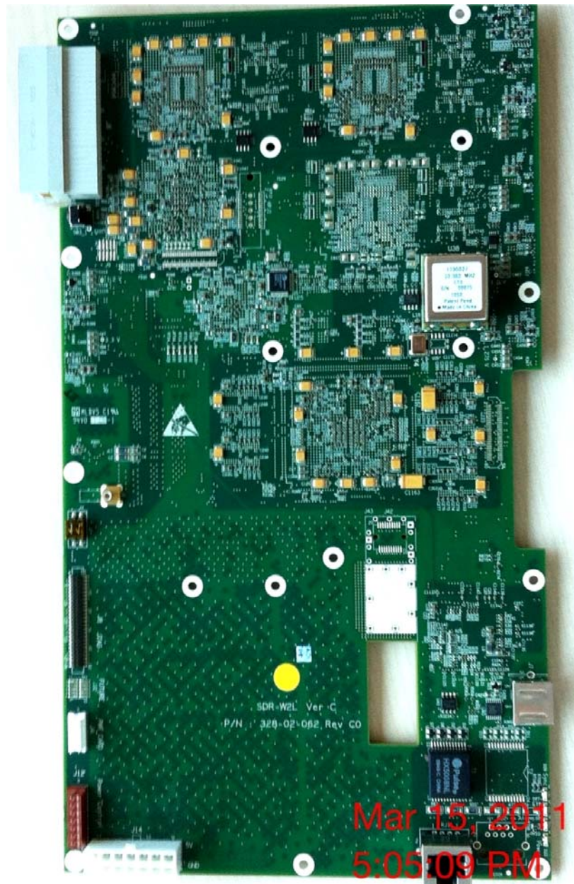
Photograph No.5 “uMAXe/AirGrid 3.65 GHz” digital PCB front view
