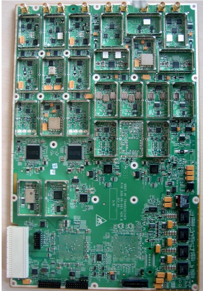
Photograph No.3 “uMAXe/AirGrid 3.65 GHz” RF card without shielding
