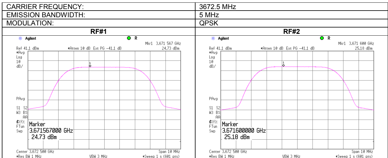
Plot 7.1.3 Peak output power density test results at high frequency
