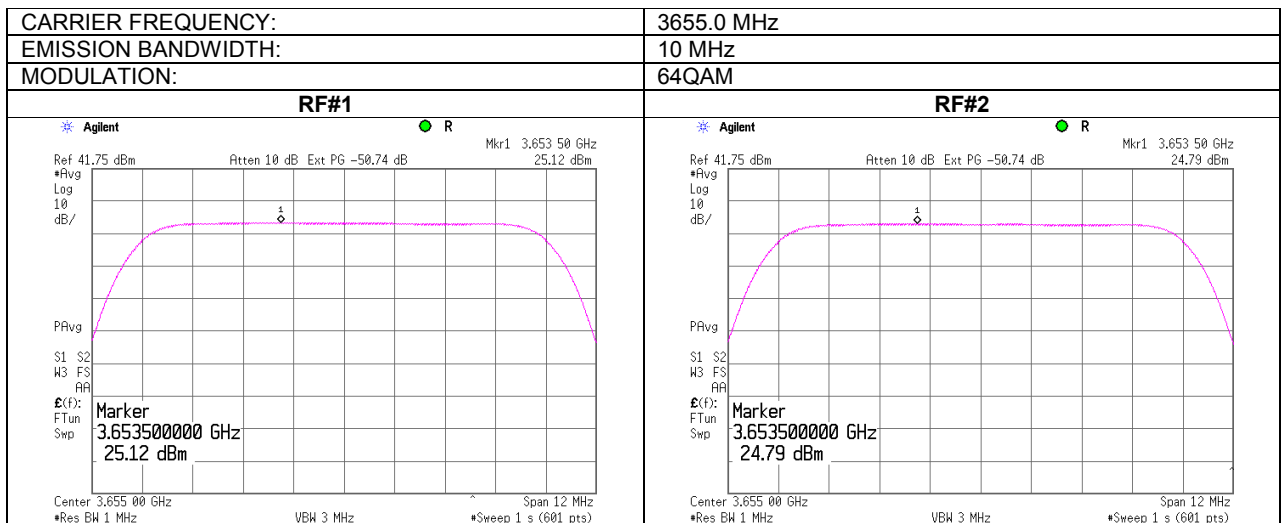
Plot 7.1.17 Peak output power density test results at mid frequency
