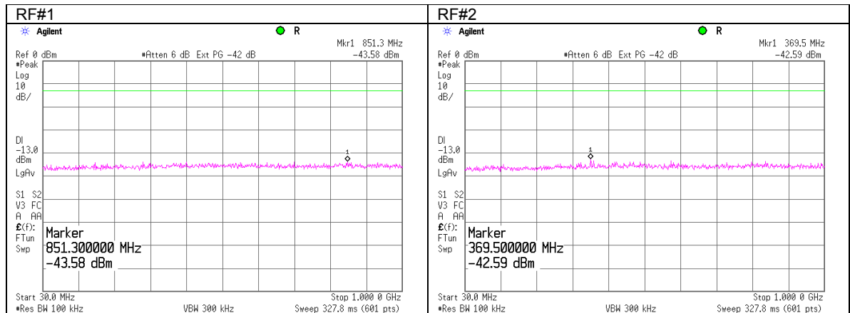
Plot 7.5.7 Spurious emission measurements in 30.0 - 1000 MHz range at low carrier frequency
