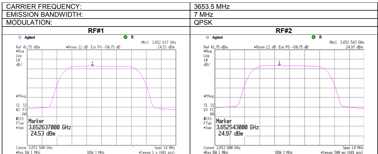
Plot 7.1.8 Peak output power density test results at mid frequency
