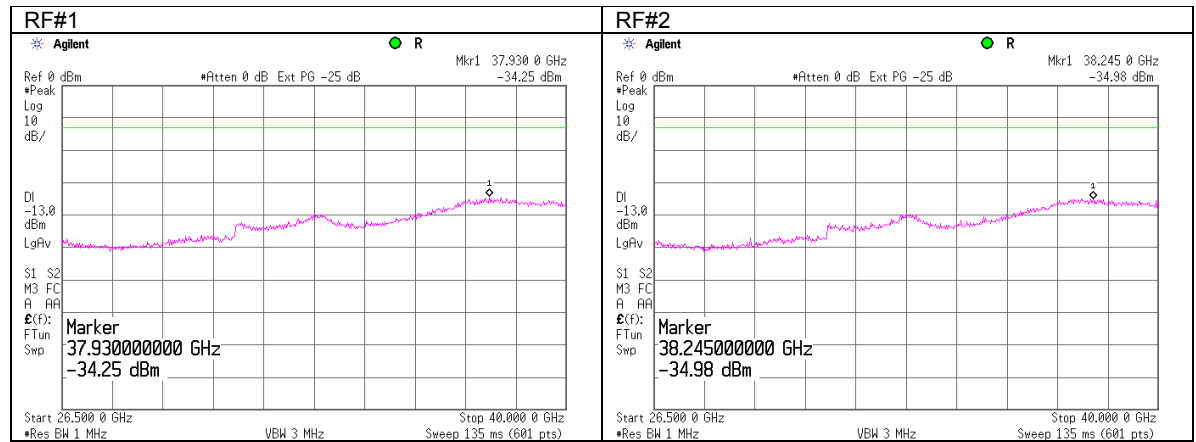
Plot 7.5.21 Spurious emission measurements in 26500 - 40000 MHz at high carrier frequency
