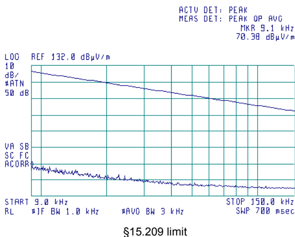
Plot 7.4.2 Radiated emission measurements in 9 - 150 kHz range
