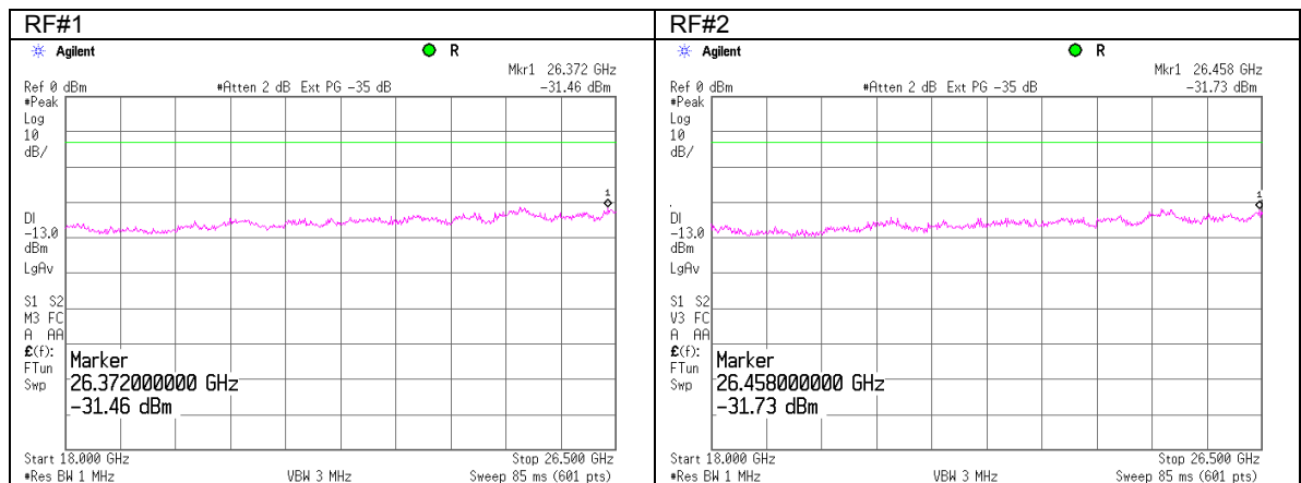
Plot 7.5.16 Spurious emission measurements in 18000 - 26500 MHz range at low carrier frequency
