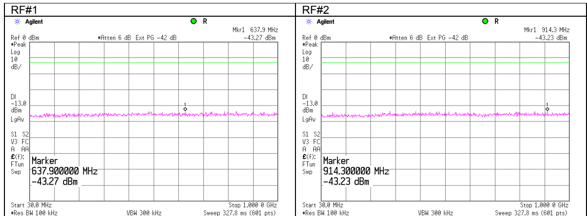
Plot 7.5.9 Spurious emission measurements in 30.0 - 1000 MHz range at high carrier frequency
