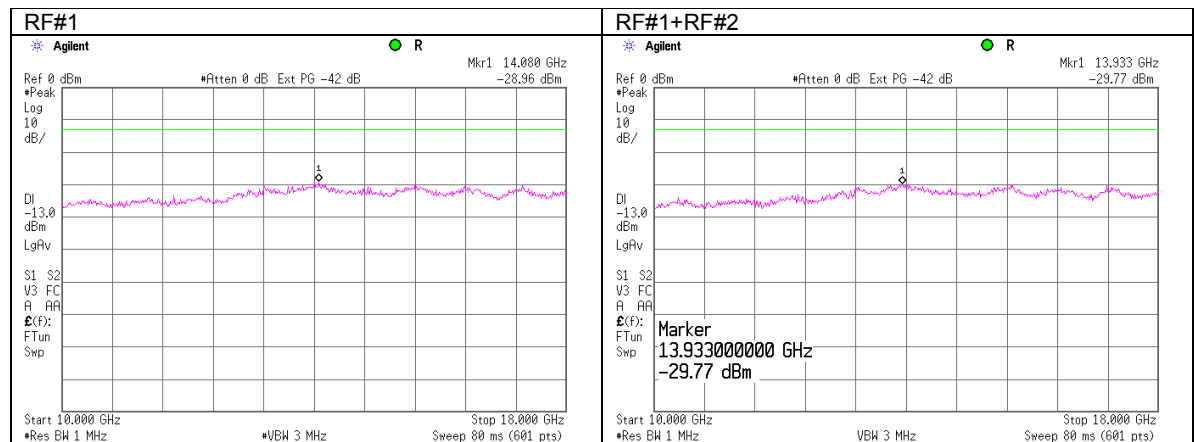
Plot 7.5.13 Spurious emission measurements in 10000 - 18000 MHz range at low carrier frequency
