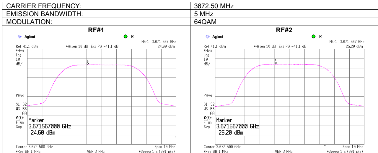
Plot 7.1.6 Peak output power density test results at high frequency
