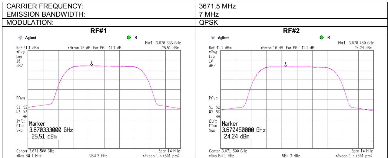
Plot 7.1.9 Peak output power density test results at high frequency
