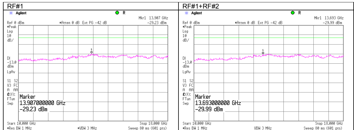
Plot 7.5.14 Spurious emission measurements in 10000 - 18000 MHz at mid carrier frequency
