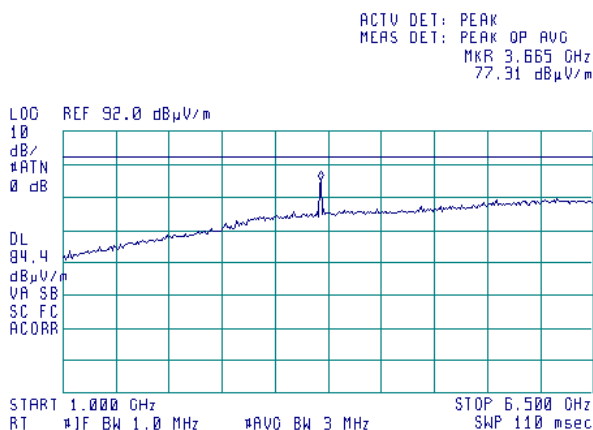
Plot 7.4.11 Radiated emission measurements in 1000 – 6500 MHz range
