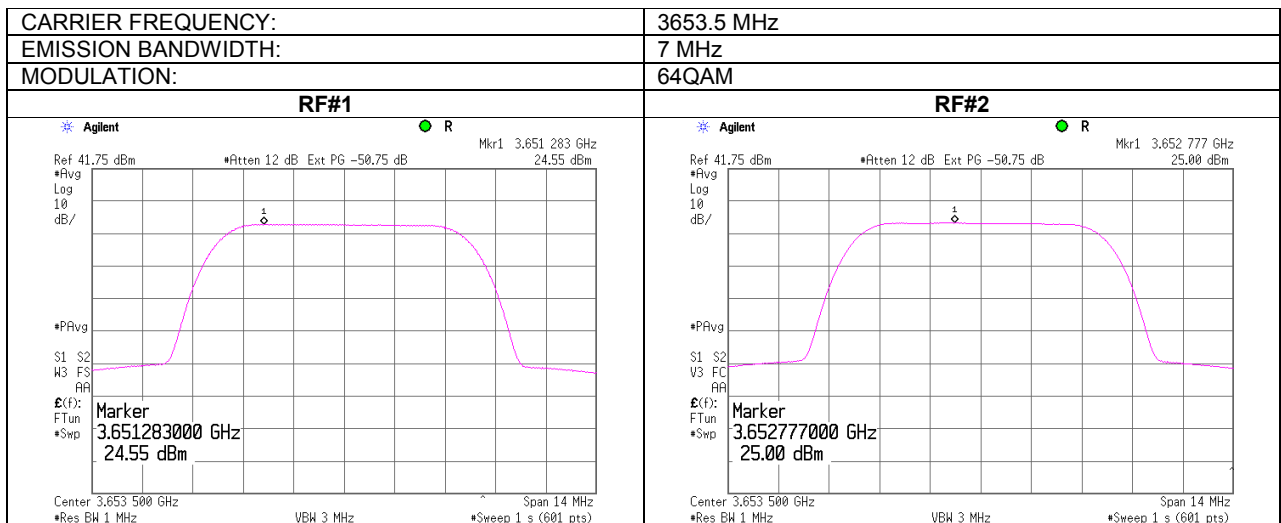
Plot 7.1.11 Peak output power density test results at mid frequency
