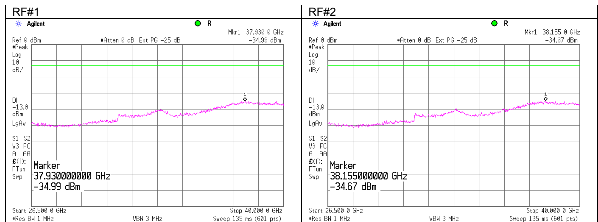
Plot 7.5.20 Spurious emission measurements in 26500 - 40000 MHz at mid carrier frequency
