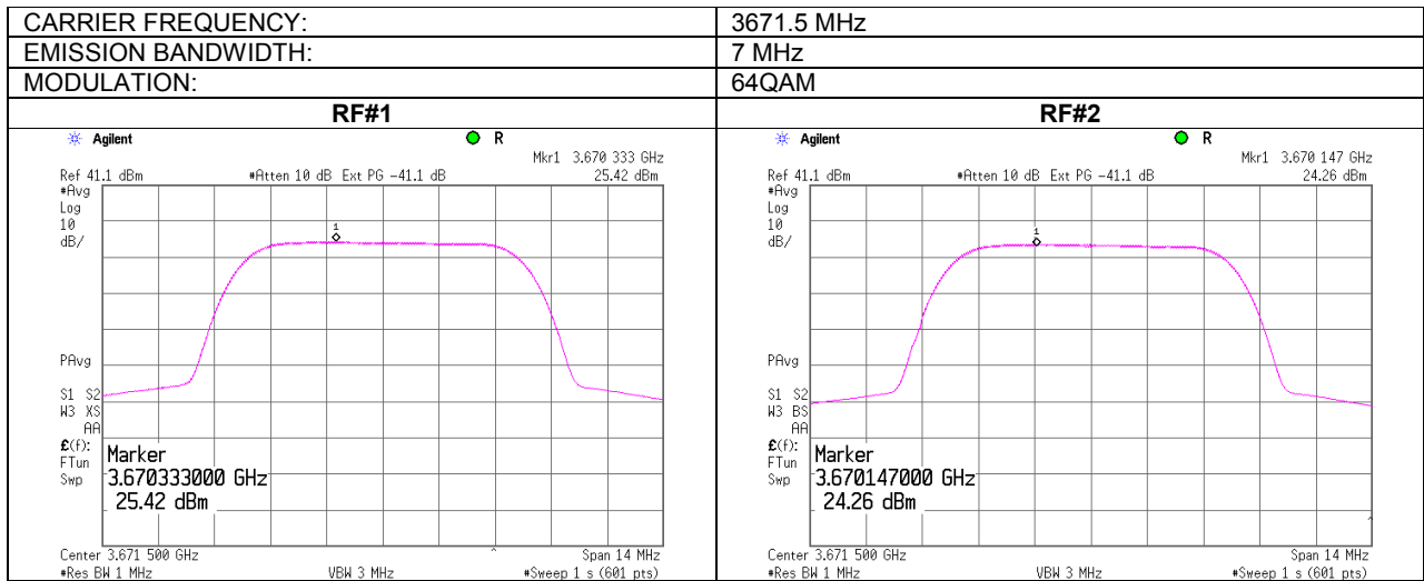
Plot 7.1.12 Peak output power density test results at high frequency
