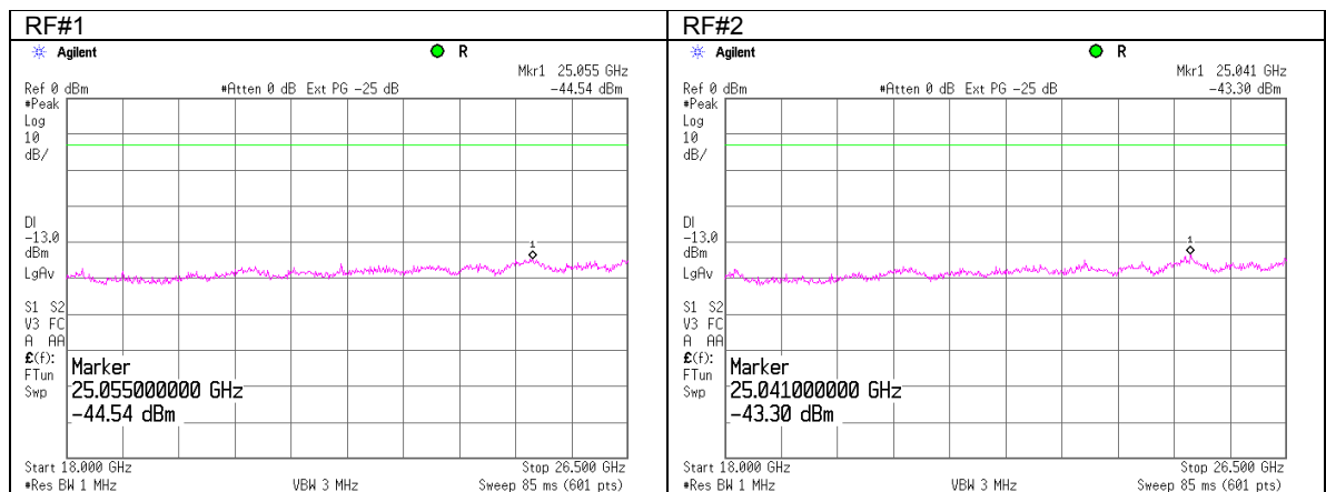
Plot 7.5.18 Spurious emission measurements in 18000 - 26500 MHz at high carrier frequency
