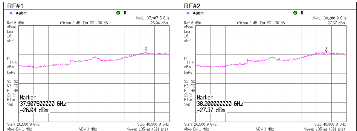
Plot 7.5.19 Spurious emission measurements in 26500 - 40000 MHz range at low carrier frequency
