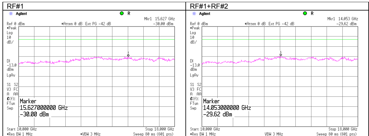
Plot 7.5.15 Spurious emission measurements in 10000 - 18000 MHz at high carrier frequency
