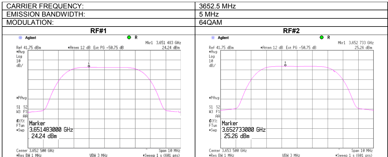
Plot 7.1.5 Peak output power density test results at mid frequency
