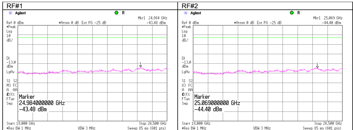
Plot 7.5.17 Spurious emission measurements in 18000 - 26500 MHz at mid carrier frequency
