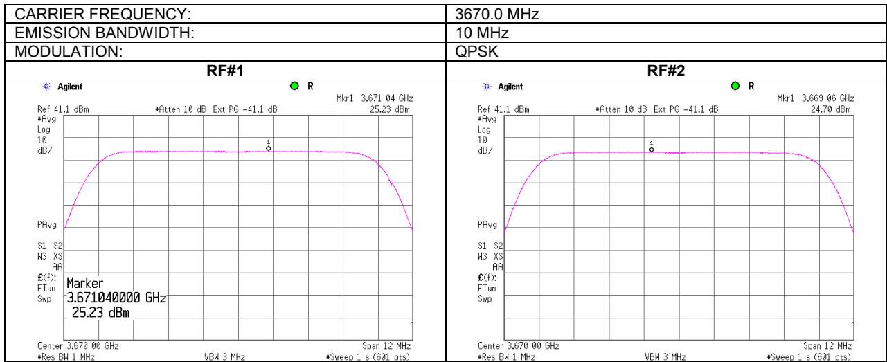
Plot 7.1.15 Peak output power density test results at high frequency
