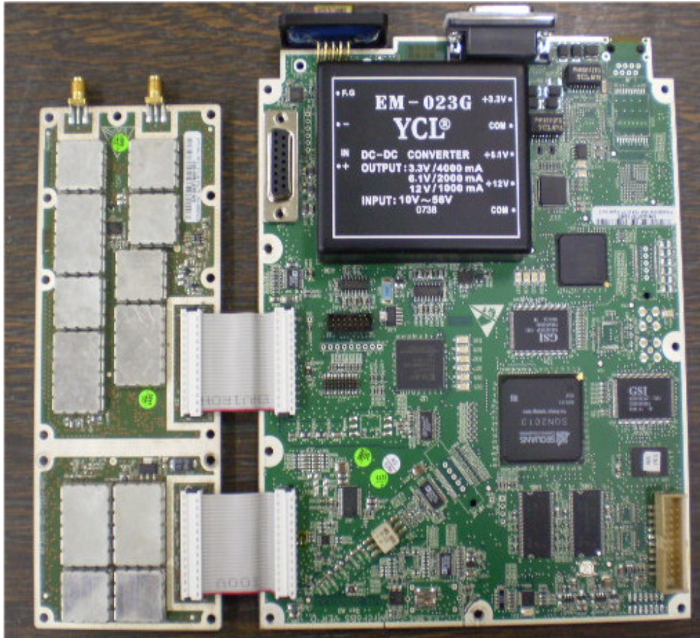
Photograph No.4 MicroMax RF module and digital interface PCB
