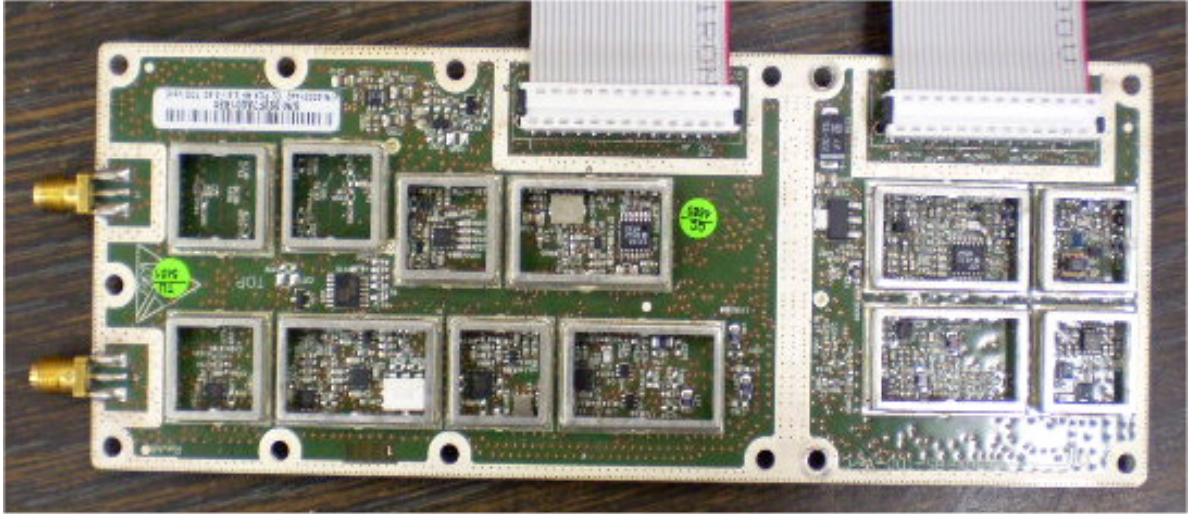
Photograph No.8 RF module without shields
