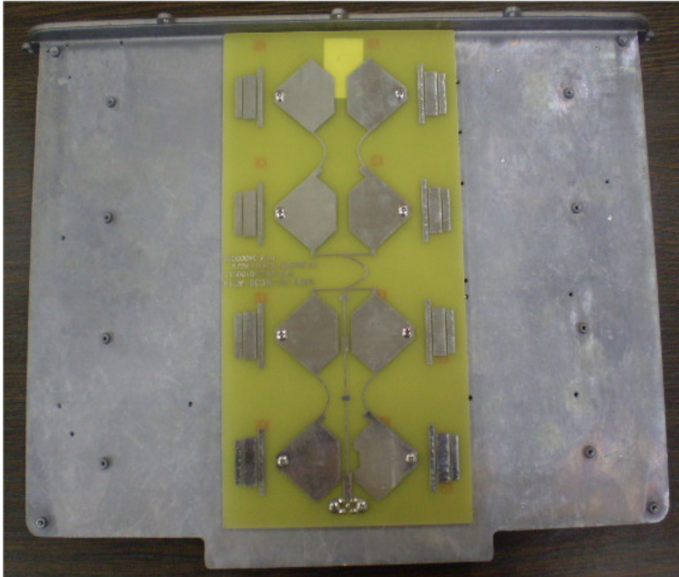
Photograph No.2 MicroMax cover with antenna
