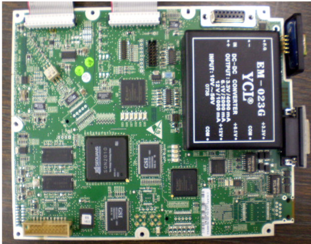
Photograph No.15 Digital interface PCB front view
