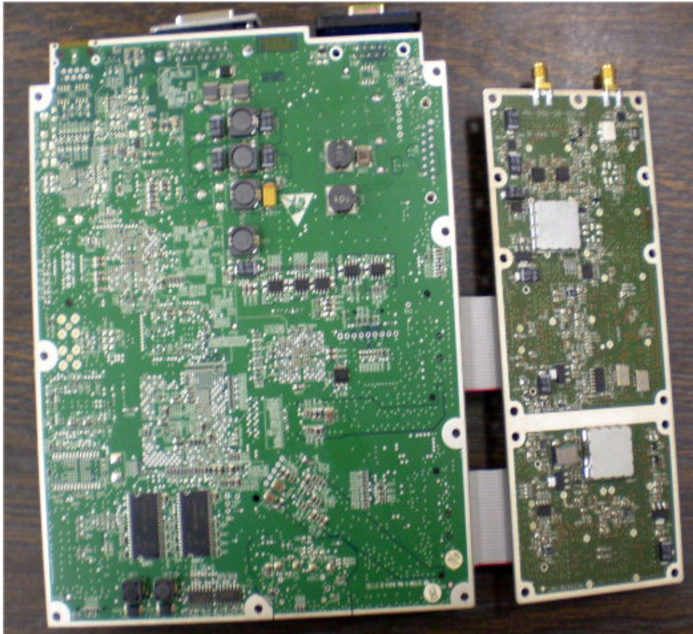
Photograph No.5 MicroMax RF module and digital interface PCB second side view
