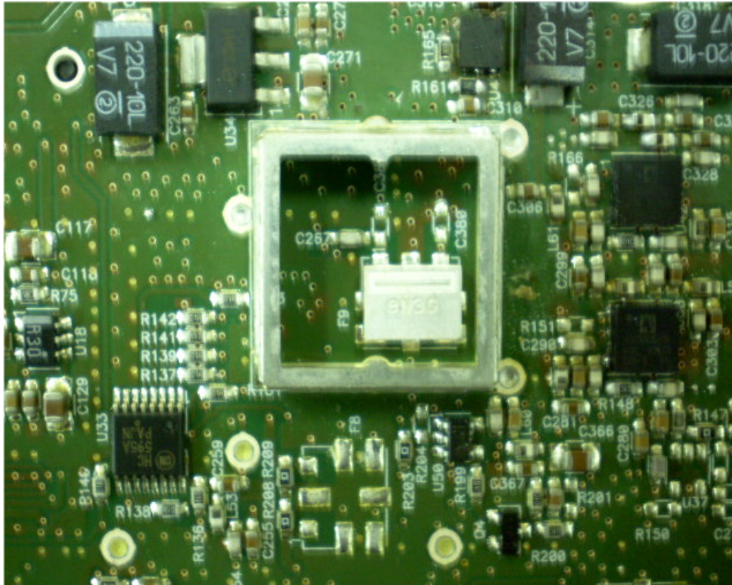
Photograph No.14 PCB second side close view, without shields
