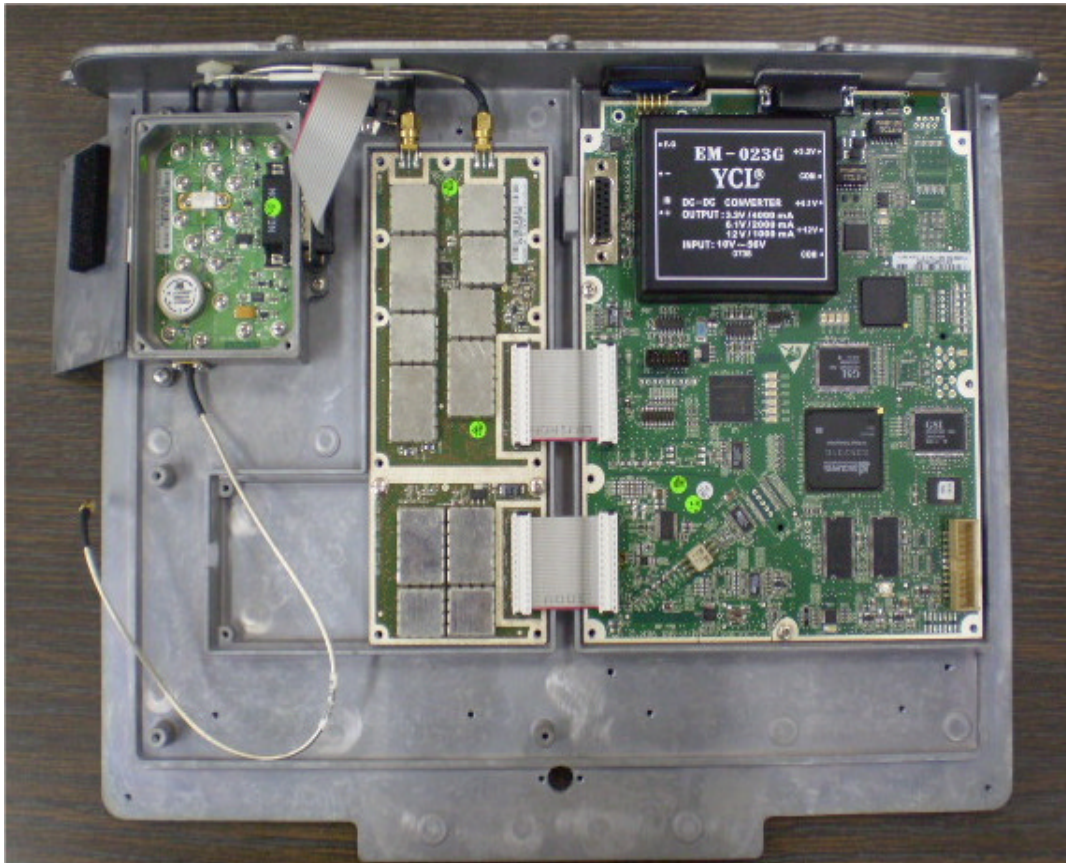
Photograph No.3 MicroMax internal view without screens
