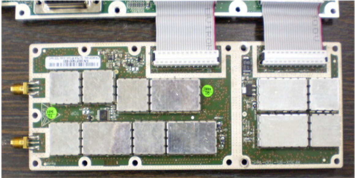
Photograph No.7 MicroMax RF module front view
