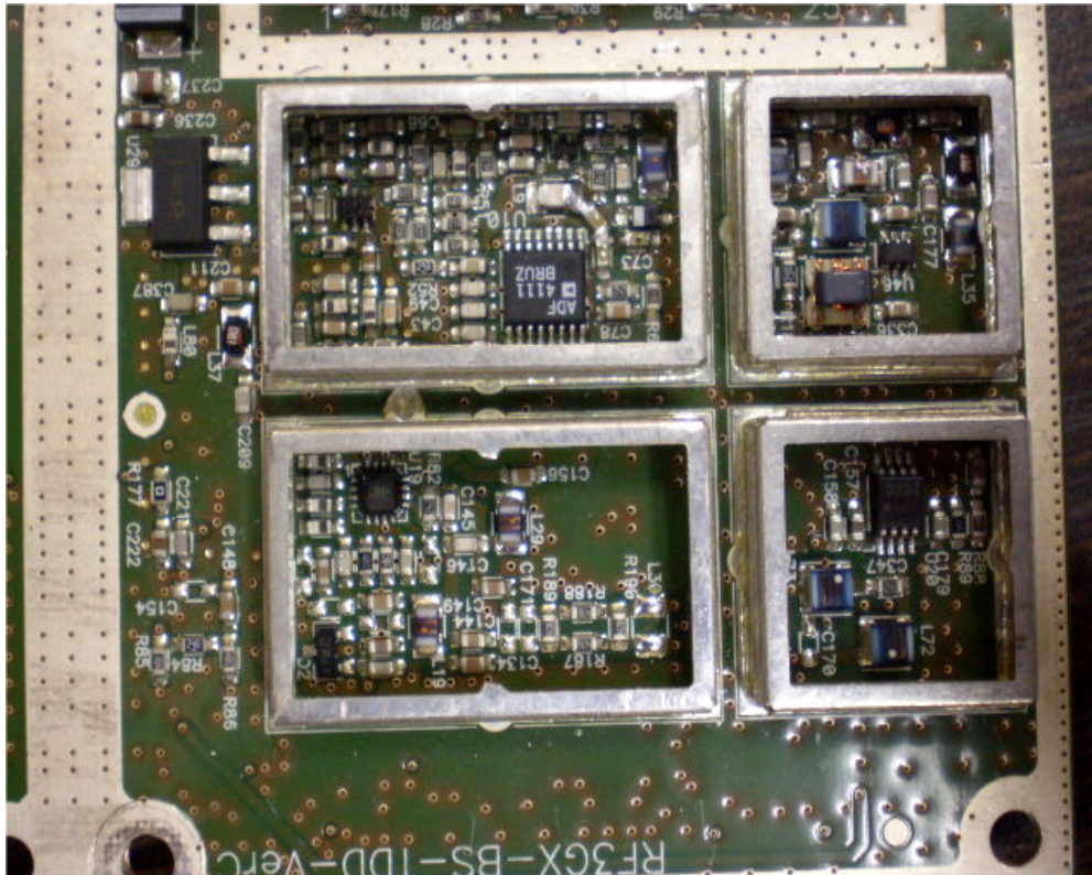
Photograph No.9 Close view without shield
