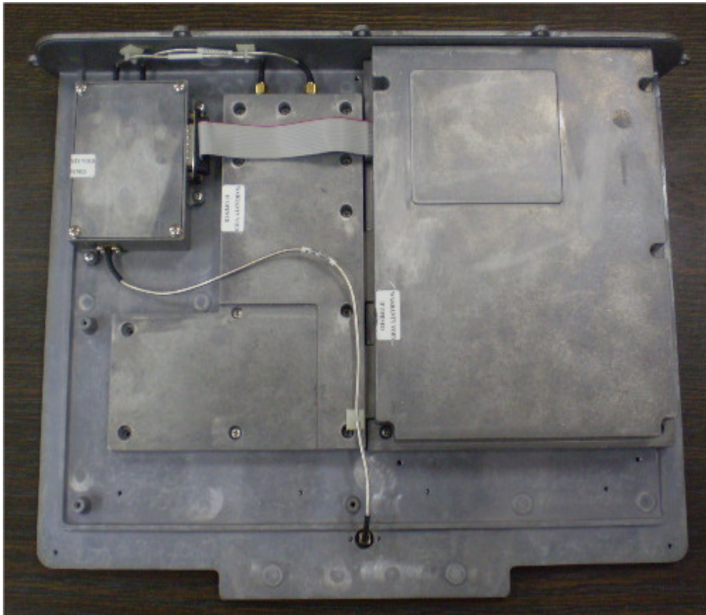
Photograph No.1 MicroMax 3.7 GHz TDD internal view
