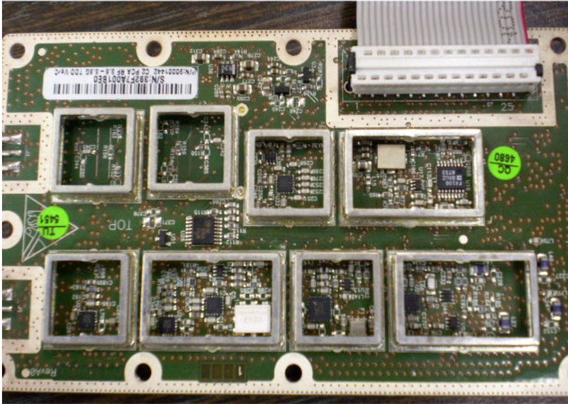
Photograph No.10 PCB left part of front side
