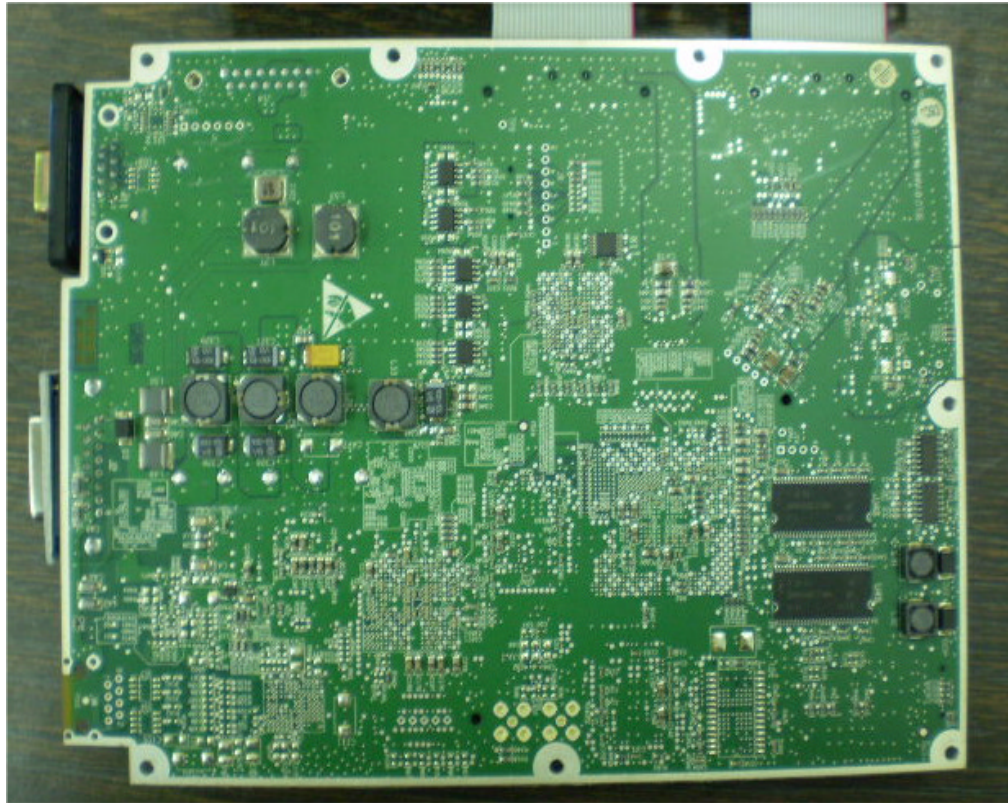
Photograph No.16 Digital interface PCB second side view
