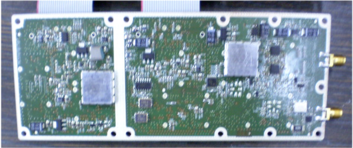
Photograph No.11 MicroMax RF module second side view
