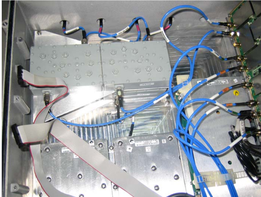
Photograph No.9 “MacroMAXe 2510H” RF filters
