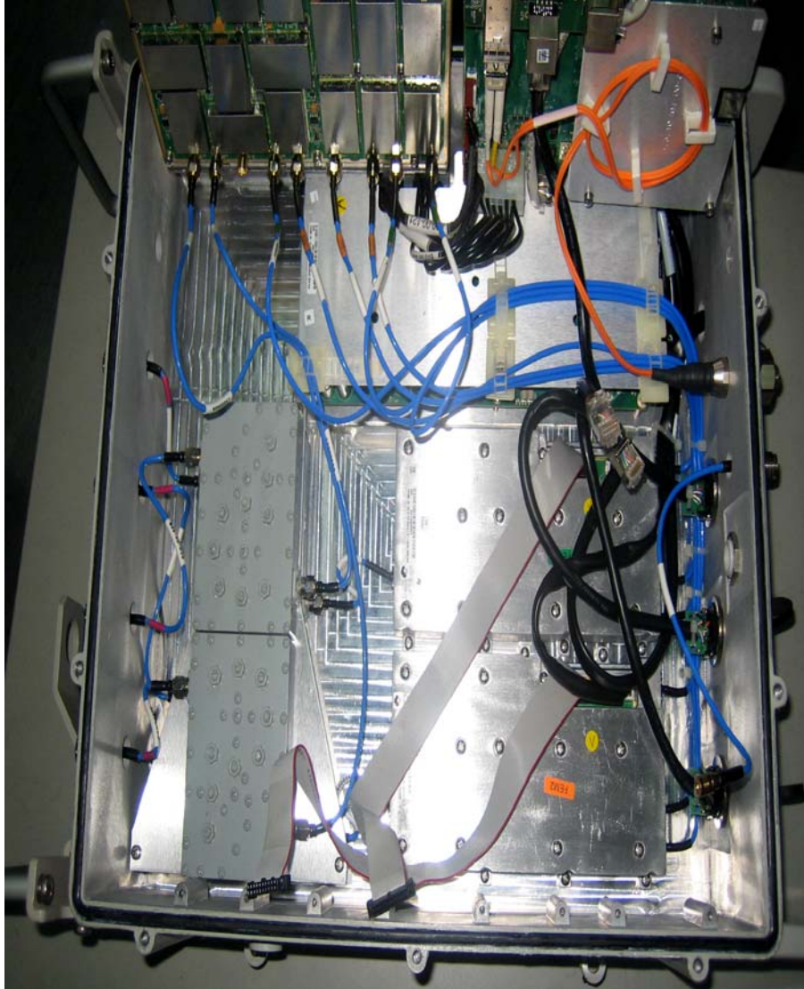
Photograph No.6 “MacroMAXe 2510H” RF power amplifiers
