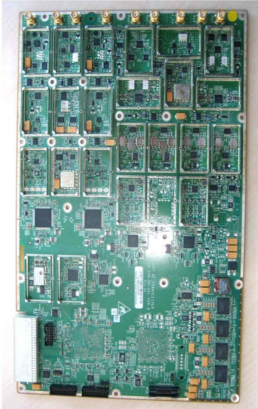
Photograph No.3 “MacroMAXe 2510H” RF card without shielding
