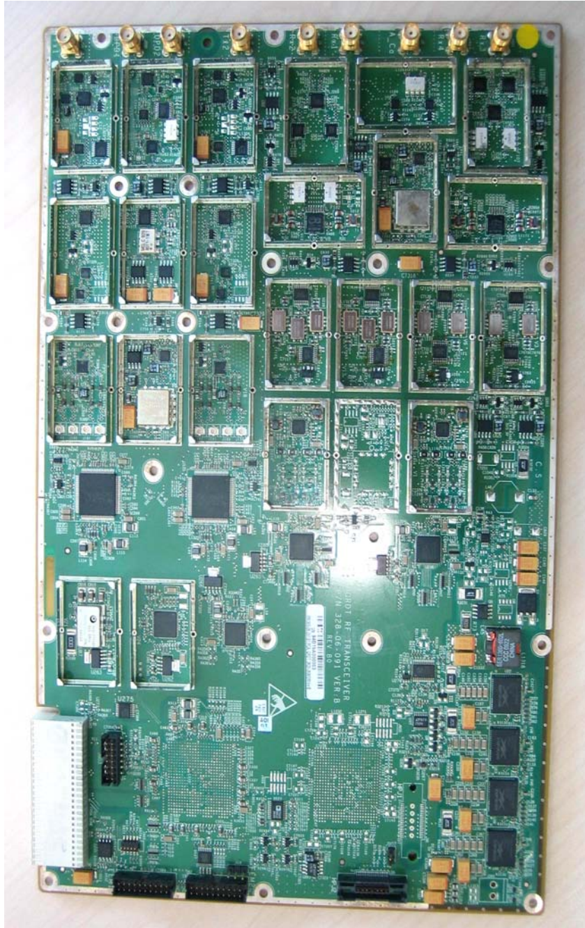
Photograph No.3 “MacroMAXe 2510 Mid” RF card without shielding
