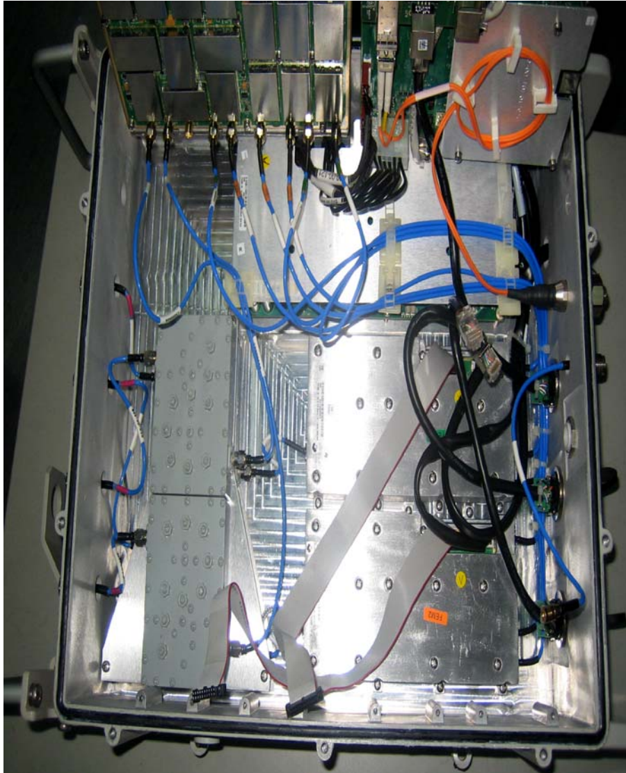
Photograph No.6 “MacroMAXe 2510 Mid” RF power amplifiers
