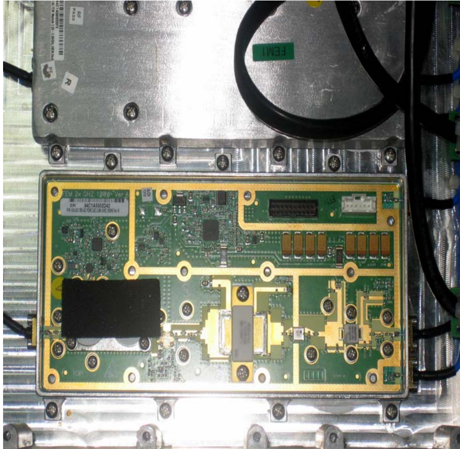
Photograph No.7 RF power amplifier internal view
