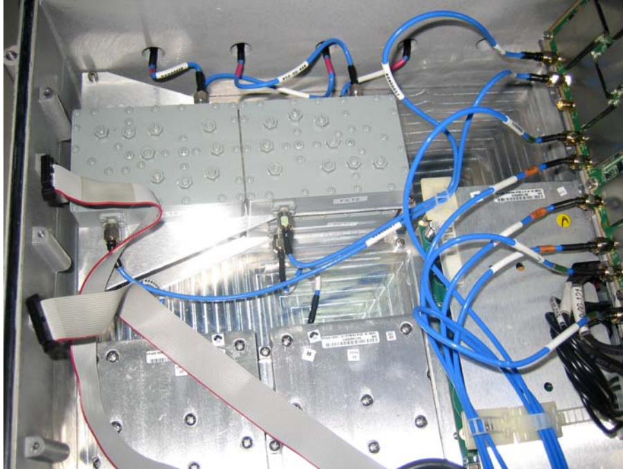
Photograph No.9 “MacroMAXe 2510L” RF filters
