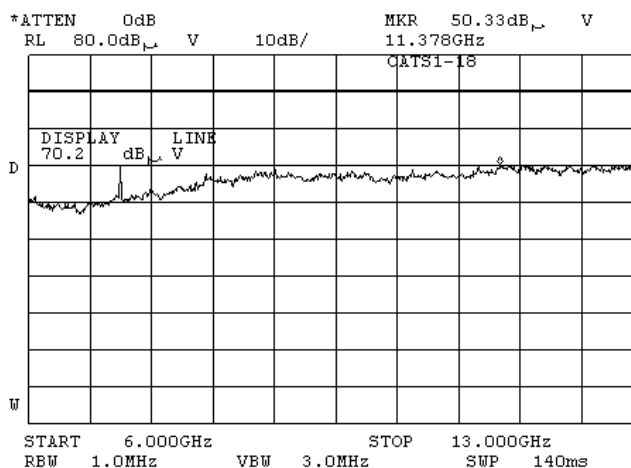
Plot 7.4.33 Radiated emission measurements in 6000 – 13000 MHz range
