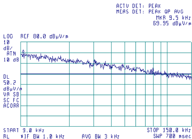
Plot 7.4.4 Radiated emission measurements from 9 to 150 kHz
