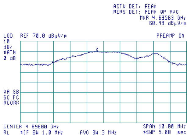
Plot 7.4.43 Radiated emission measurements at the 2 nd harmonic
