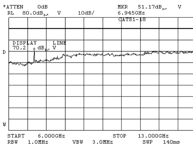
Plot 7.4.31 Radiated emission measurements in 6000 – 13000 MHz range
