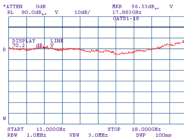
Plot 7.4.37 Radiated emission measurements in 13000 – 18000 MHz range
