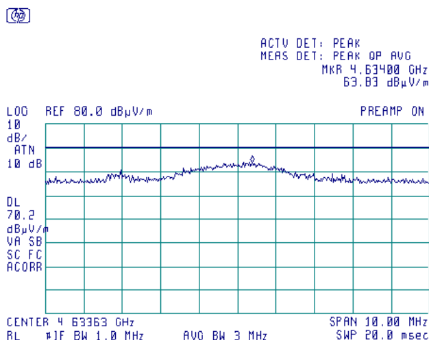
Plot 7.4.41 Radiated emission measurements at the 2 nd harmonic
