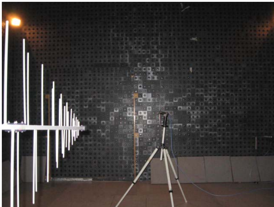
Photograph No.6 Setup for substitution ERP measurements of spurious
