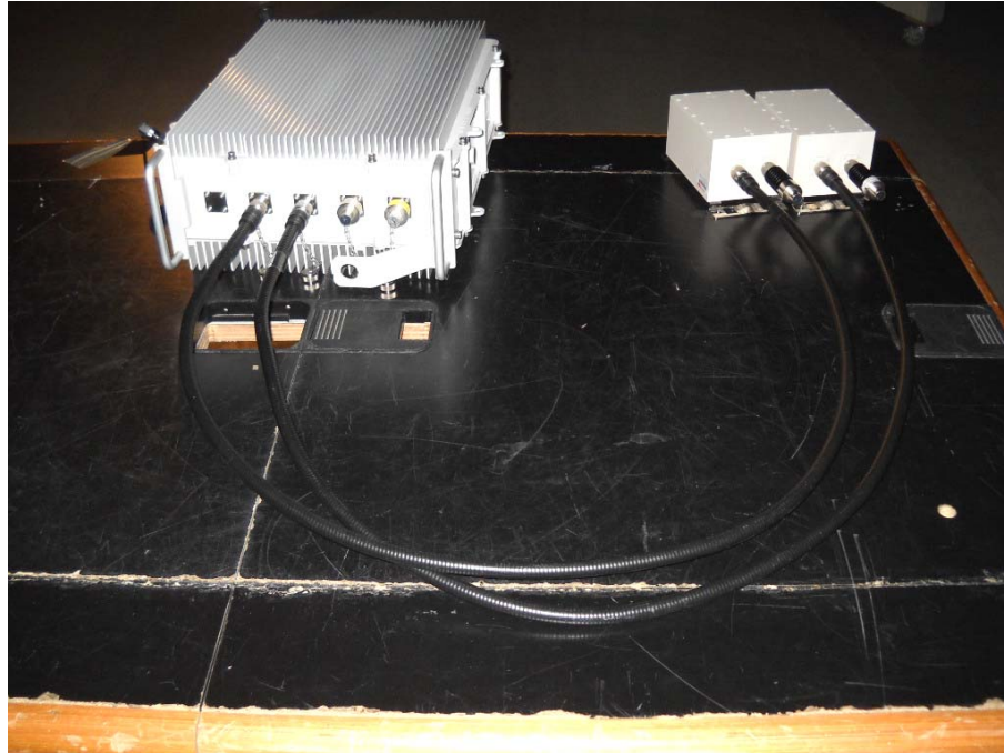
Photograph No.5 Radiated emissions measurement setup in the anechoic chamber, EUT close view
