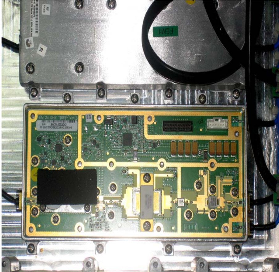
Photograph No.8 RF power amplifier internal view
