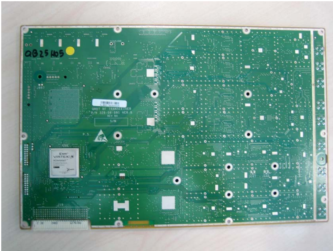
Photograph No.4 “Air4G-MacroMAXe 2310L” RF card second side view
