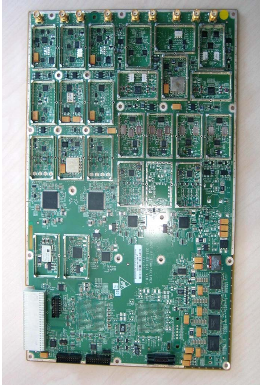
Photograph No.3 “Air4G-MacroMAXe 2310L” RF card without shielding
