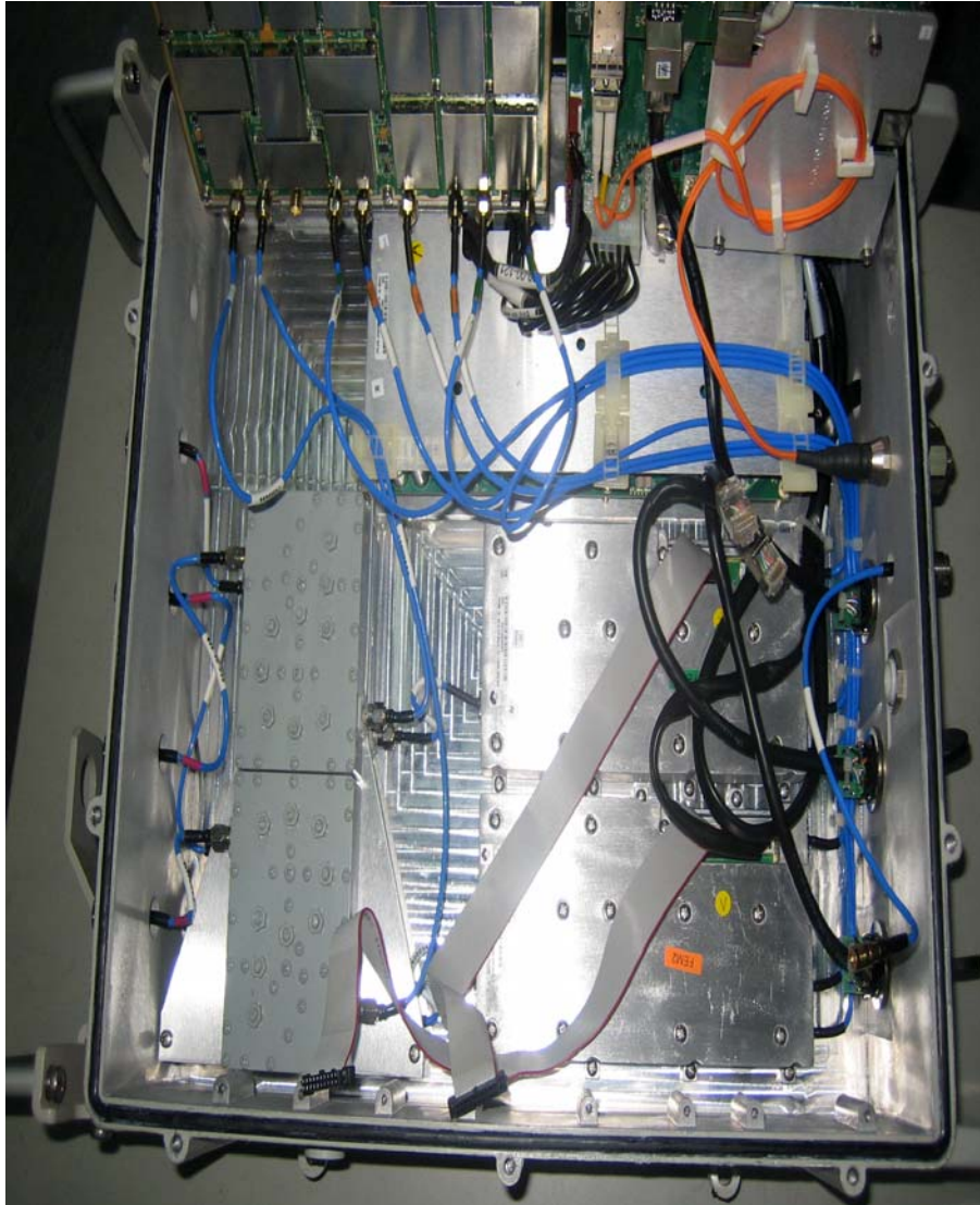
Photograph No.7 “Air4G-MacroMAXe 2310L” RF power amplifiers
