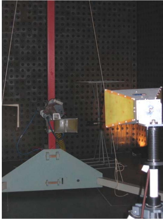
Photograph No.6 Setup for substitution ERP measurements of spurious
