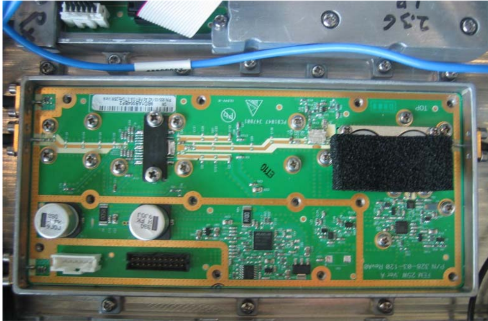
Photograph No.8 RF power amplifier internal view
