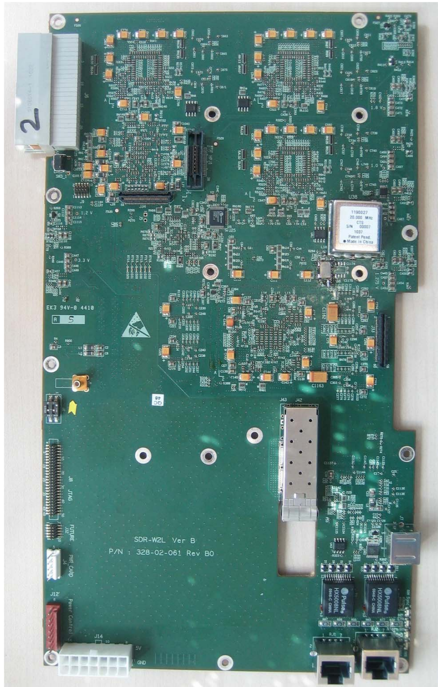
Photograph No.5 Digital PCB front view
