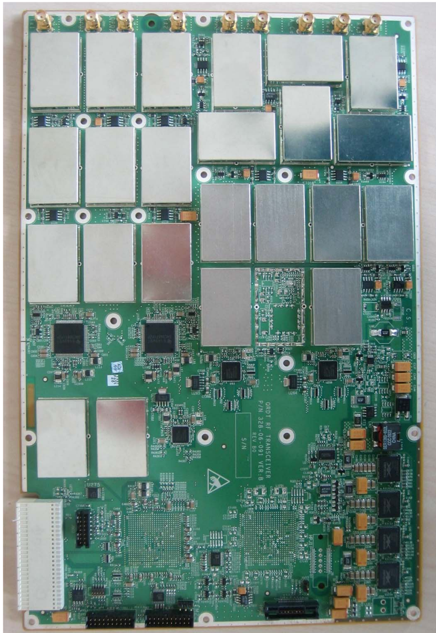
Photograph No.2 “uMAXe 2310L” RF card front view
