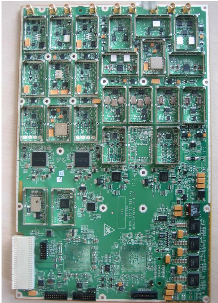
Photograph No.3 “uMAXe 2310L” RF card without shielding
