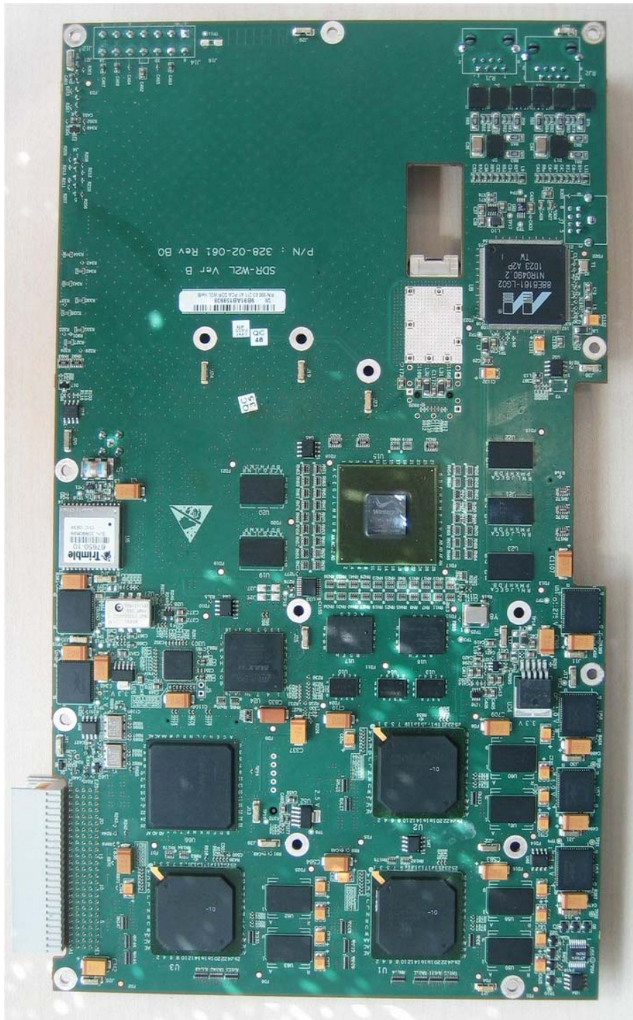
Photograph No.6 Digital PCB rear side view
