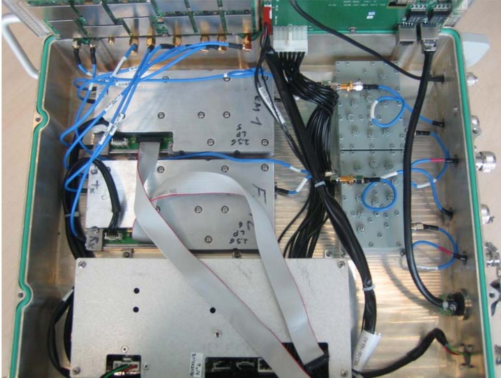
Photograph No.7 “uMAXe 2310L” RF power amplifiers
