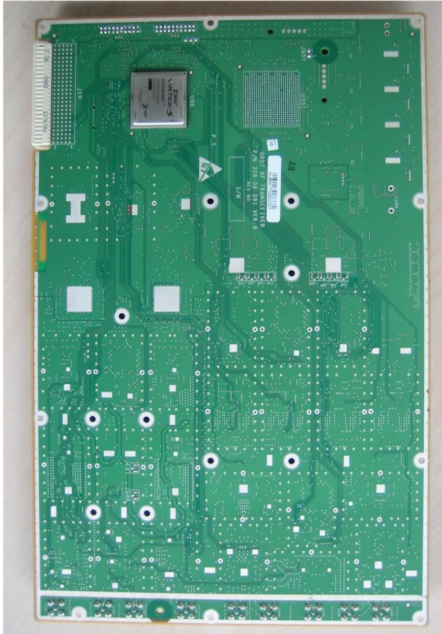
Photograph No.4 “uMAXe 2310L” RF card second side view
