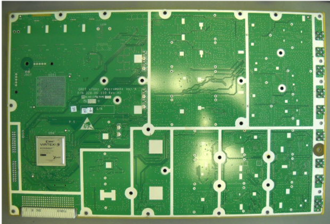
Photograph No6 "MacroMAXe 0707 700M Ext" RF card second side view
