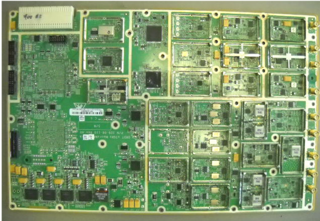
Photograph No4 “MacroMAXe 0707 700M Ext” RF card without shielding
