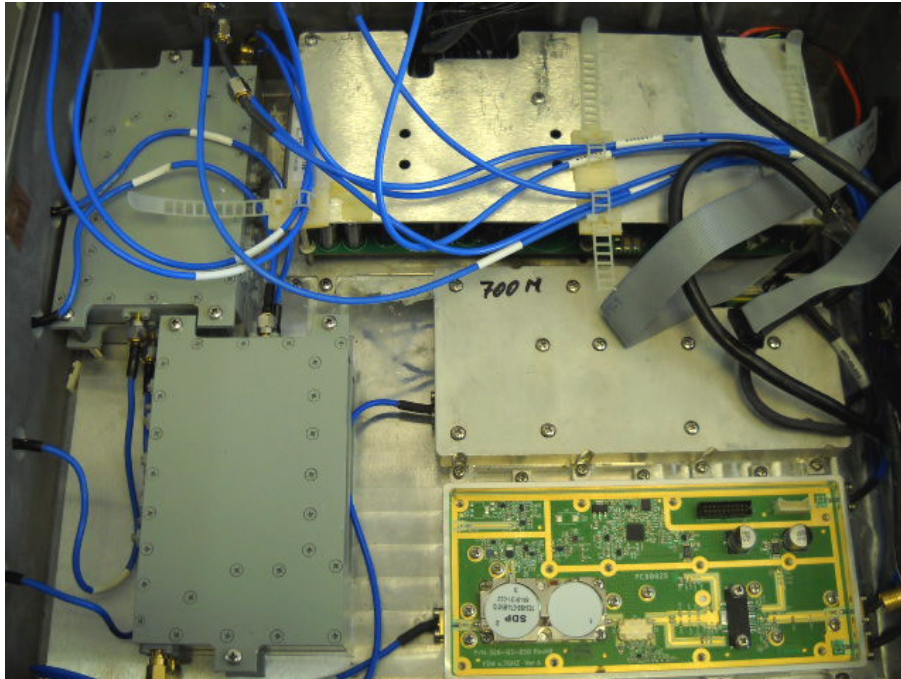
Photograph No2 RF cavity filters assembly
