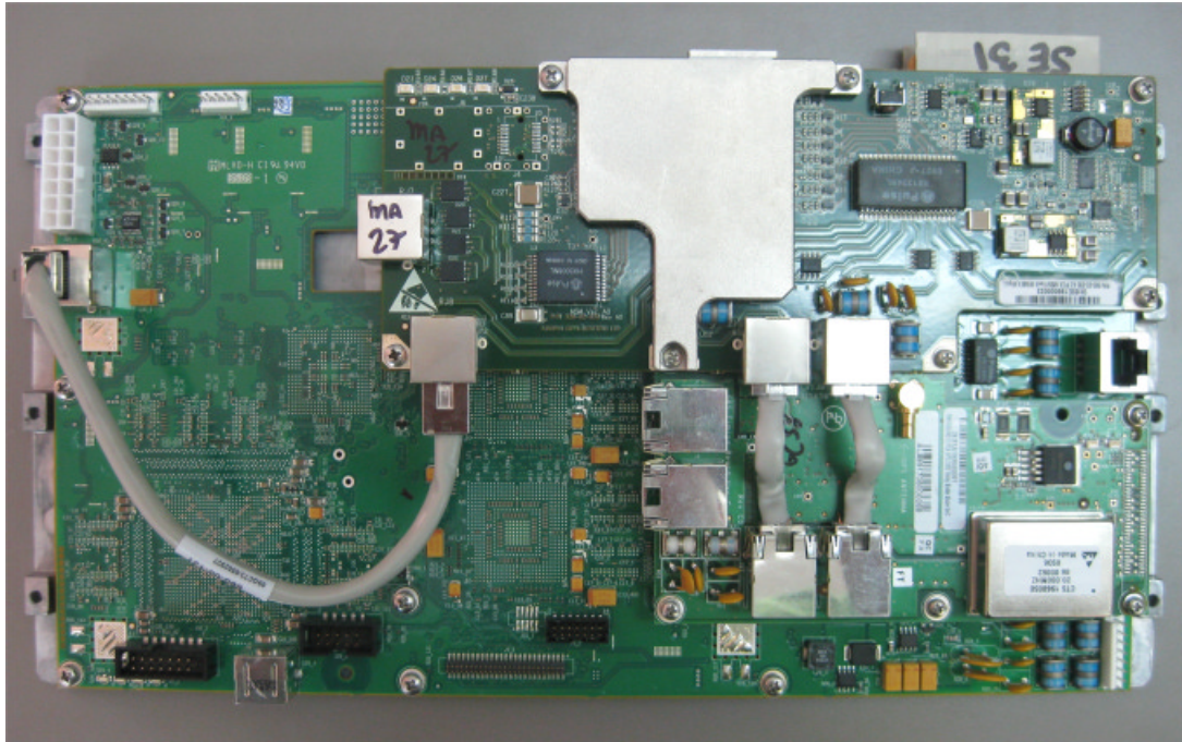
Photograph No.7 Digital PCB front view
