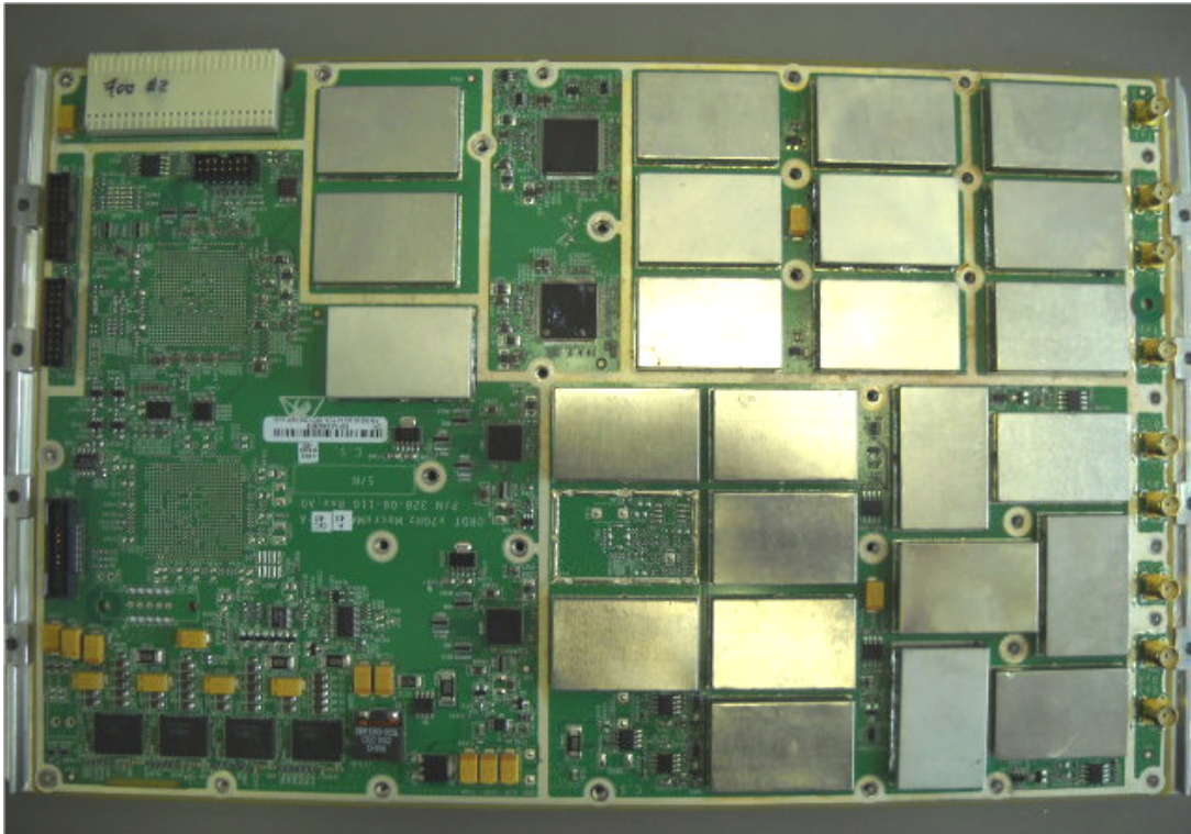
Photograph No3 “MacroMAXe 0707 700M Ext” RF card front view
