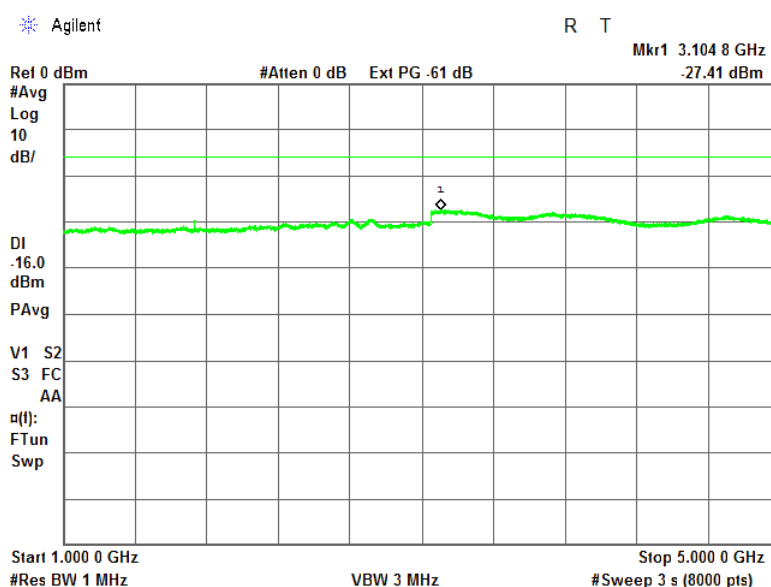
Plot 7.5.13 Spurious emission measurements in 1000 - 5000 MHz at ant.1
