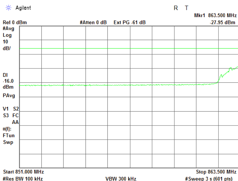
Plot 7.5.4 Spurious emission measurements in 851.0 – 863.5 MHz range at ant.0
