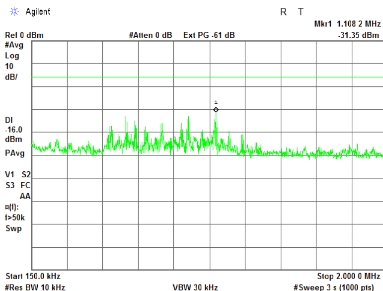
Plot 7.5.9 Spurious emission measurements in 0.15 - 2.0 MHz range at ant.1
