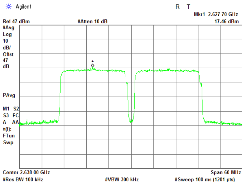
Plot 7.2.7 Power spectral density test results at low frequency, QPSK, 40 MHz EBW RF # 2
