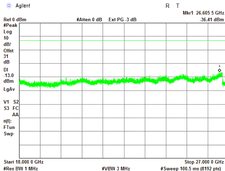
Plot 7.4.27 Spurious emission measurements in 18000 - 27000 MHz at high carrier frequency
