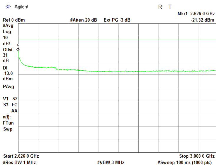
Plot 7.4.16 Spurious emission measurements in 2626 - 3000 MHz range at low carrier frequency
