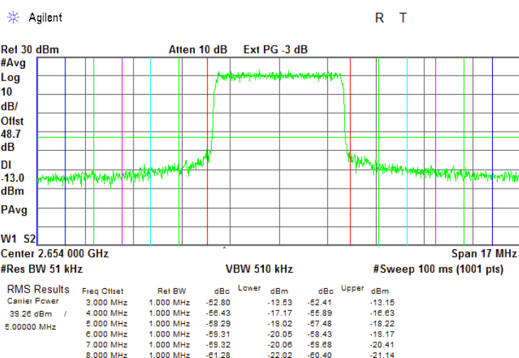
Plot 7.3.6 Spurious emission at band edges test results at high carrier frequency, 5 MHz EBW
