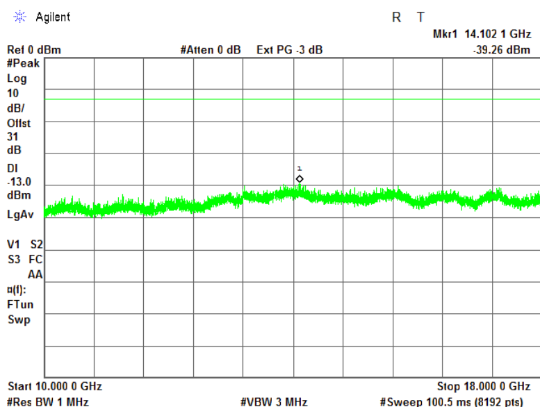
Plot 7.4.23 Spurious emission measurements in 10000 - 18000 MHz at mid carrier frequency
