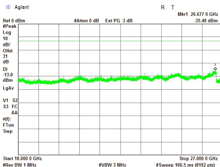
Plot 7.4.25 Spurious emission measurements in 18000-27000 MHz range at low carrier frequency
