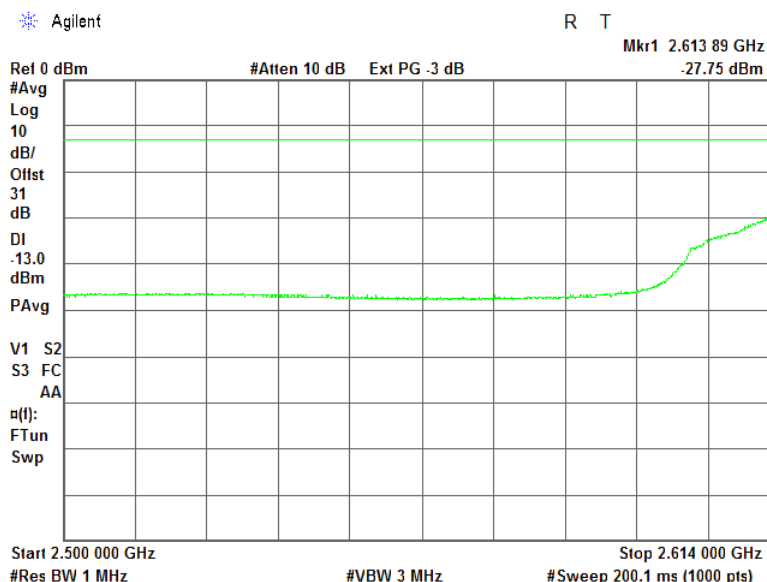
Plot 7.4.11 Spurious emission measurements in 2500 – 2614 MHz range at low carrier frequency
