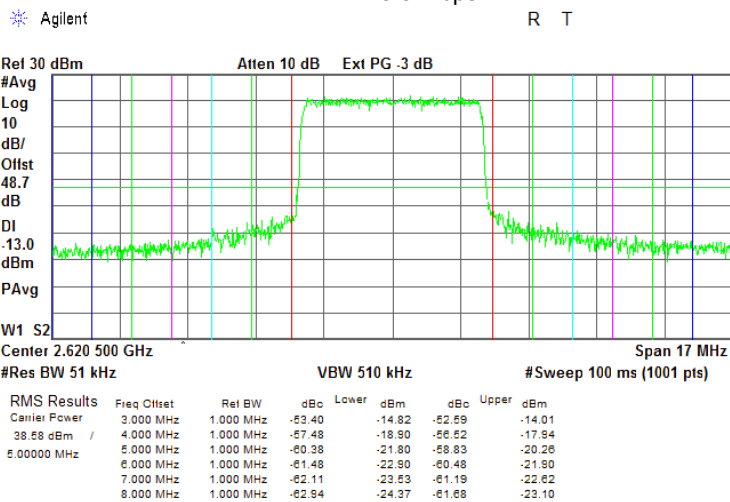
Plot 7.3.2 Spurious emission at band edges test results at mid carrier frequency, 5 MHz EBW
