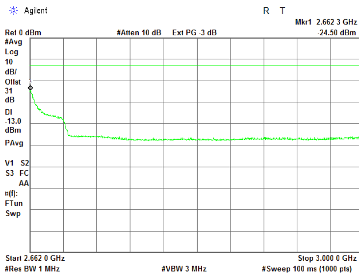
Plot 7.4.17 Spurious emission measurements in 2662 - 3000 MHz at mid carrier frequency
