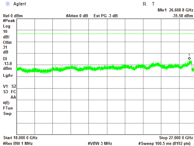
Plot 7.4.26 Spurious emission measurements in 18000 - 27000 MHz at mid carrier frequency
