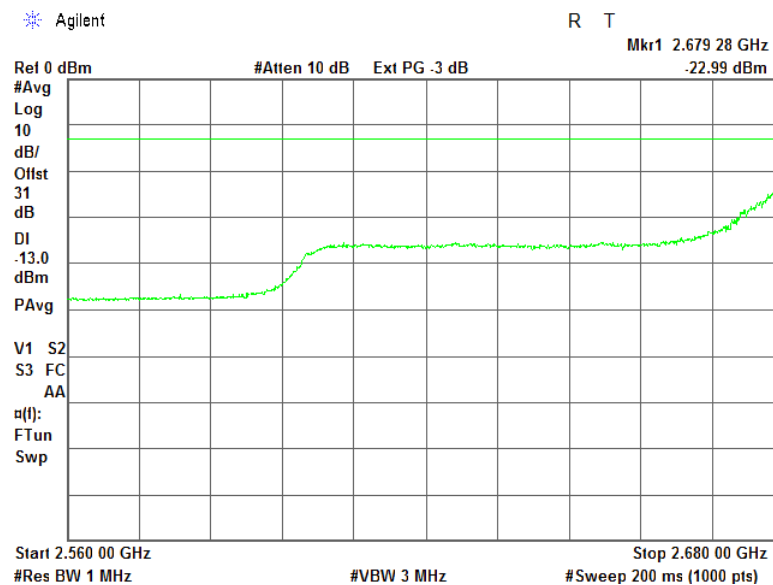
Plot 7.4.15 Spurious emission measurements in 2560 - 2680 MHz at high carrier
