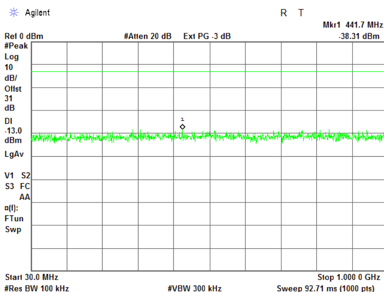
Plot 7.4.8 Spurious emission measurements in 30 - 1000 MHz range at mid carrier frequency
