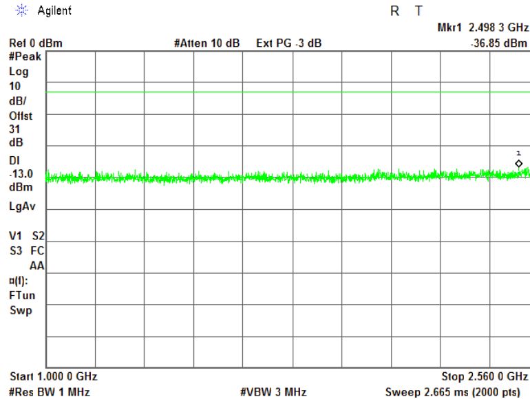
Plot 7.4.14 Spurious emission measurements in 1000 - 2560 MHz at high carrier frequency
