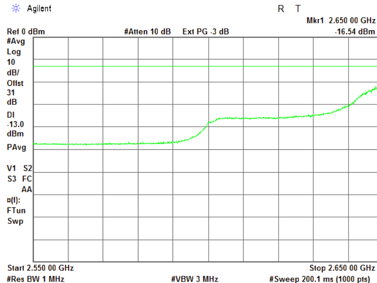
Plot 7.4.13 Spurious emission measurements in 2550 - 2650 MHz at mid carrier frequency
