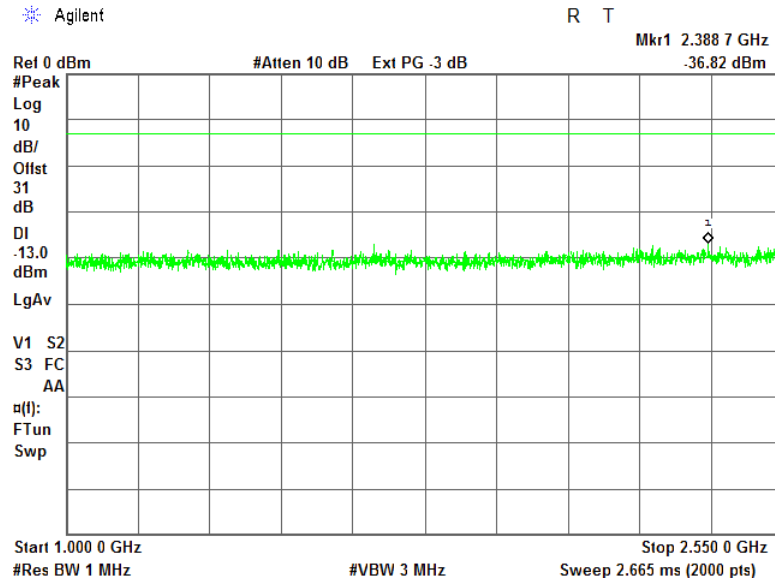
Plot 7.4.12 Spurious emission measurements in 1000 - 2550 MHz at mid carrier frequency
