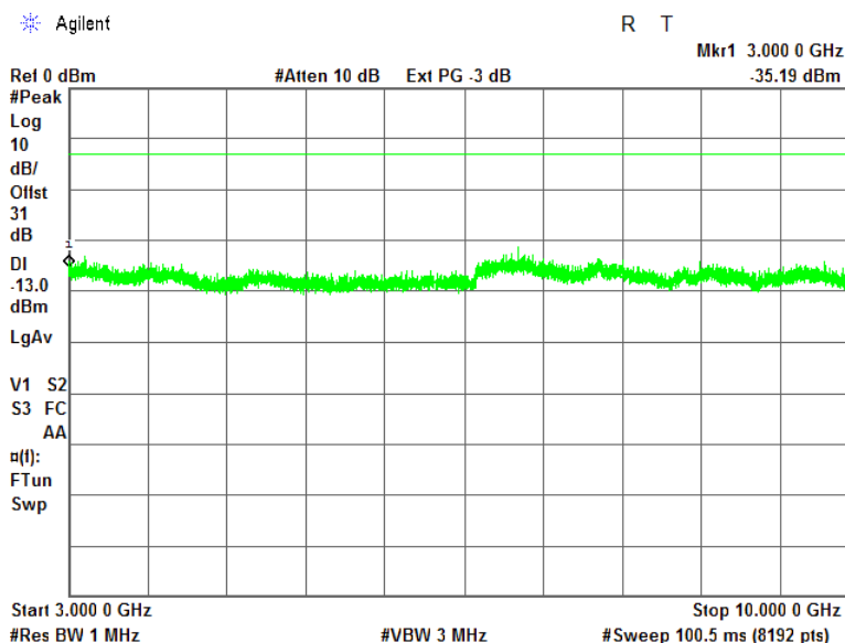
Plot 7.4.19 Spurious emission measurements in 3000-10000 MHz range at low carrier frequency
