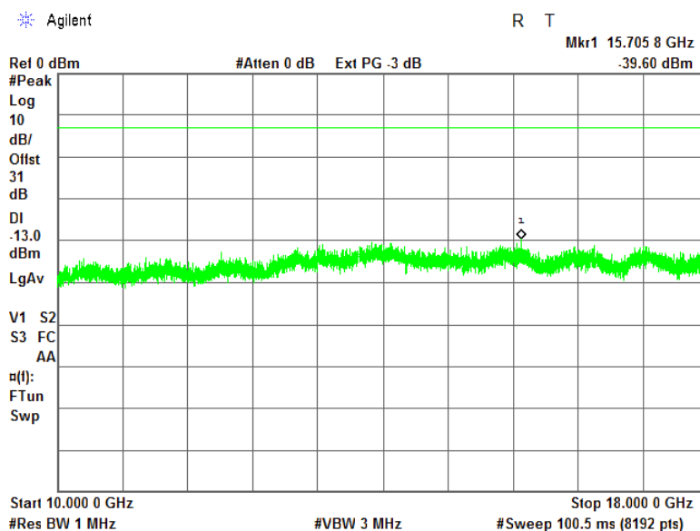
Plot 7.4.24 Spurious emission measurements in 10000 - 18000 MHz at high carrier frequency
