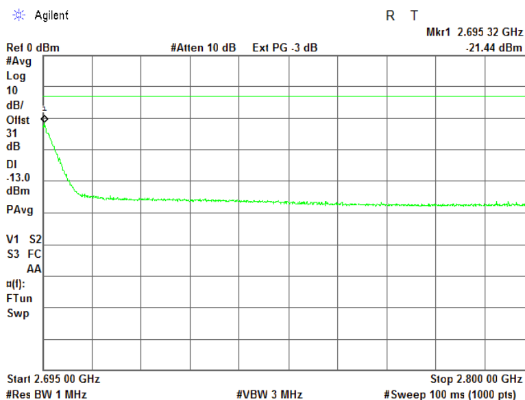
Plot 7.4.18 Spurious emission measurements in 2695 - 2800 MHz at high carrier frequency
