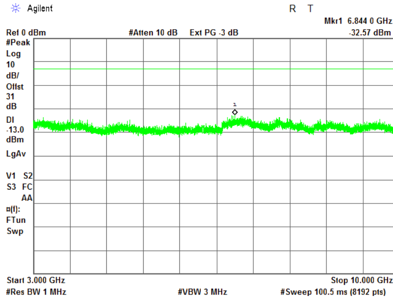
Plot 7.4.20 Spurious emission measurements in 3000 - 10000 MHz at mid carrier frequency
